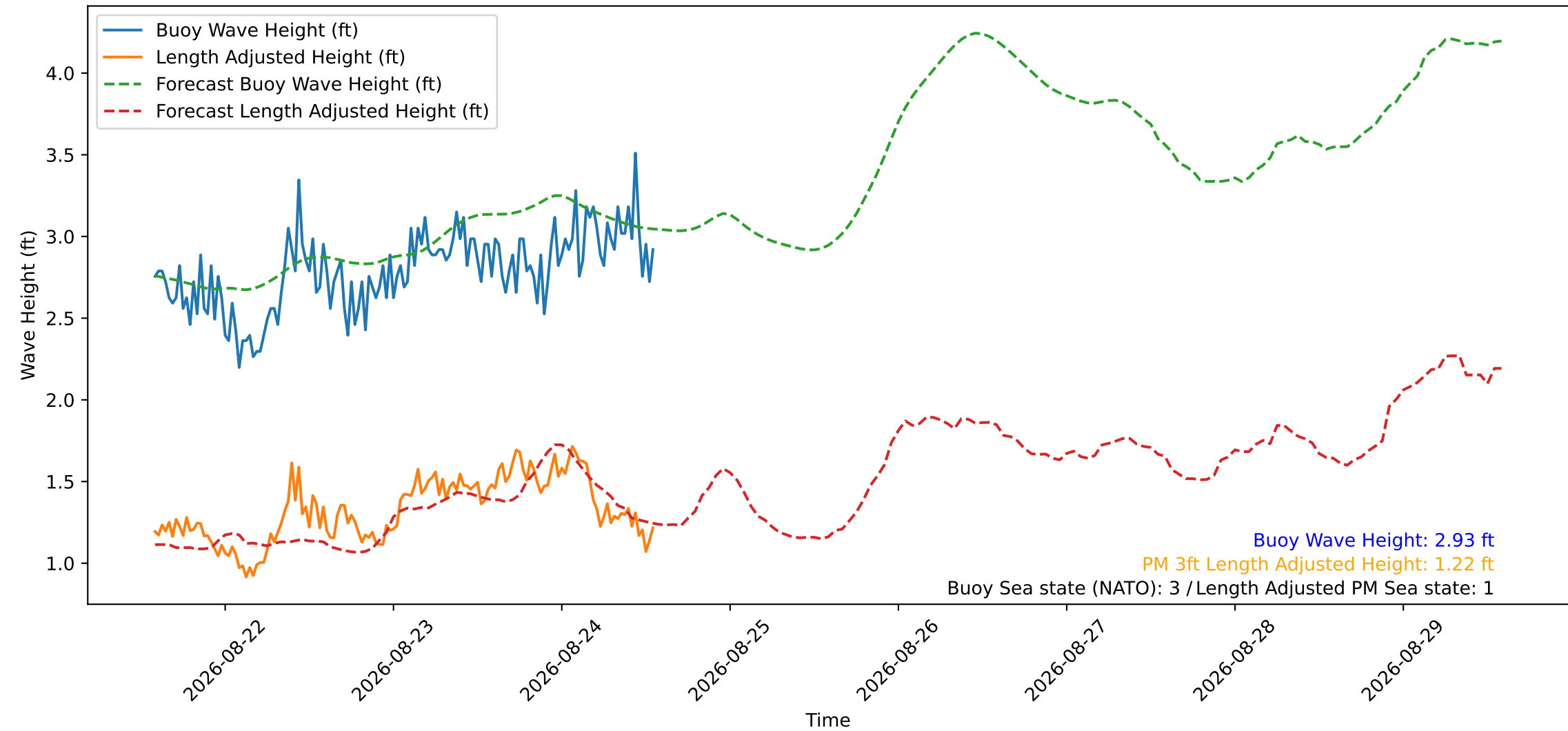
Wave Heights over Time for Oceanside Harbor at 2026-08-24 14:00:30
