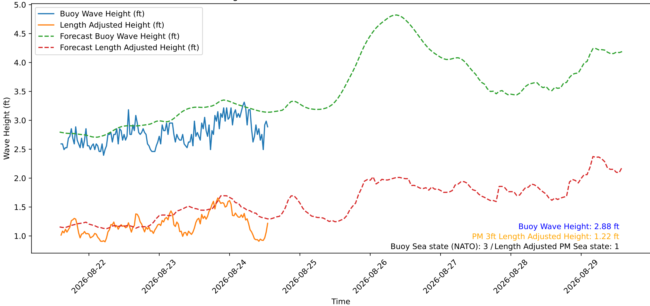
Wave Heights over Time for Green Beach at 2026-08-24 14:01:12
