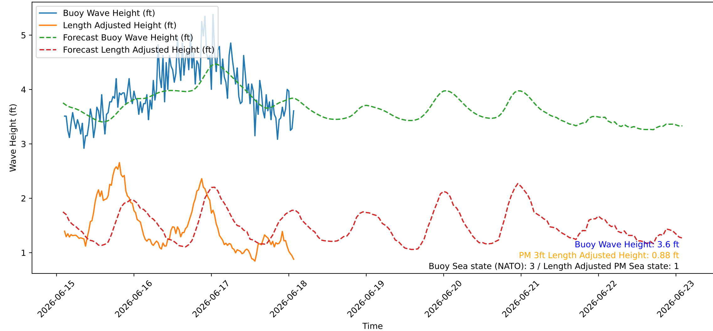
Wave Heights over Time for Red Beach at 2026-06-18 02:10:45
