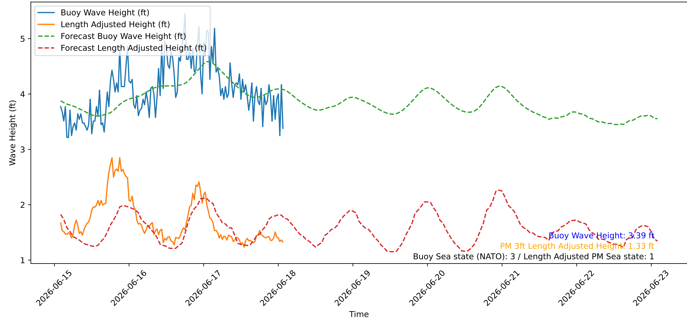
Wave Heights over Time for Oceanside Harbor at 2026-06-18 02:10:26
