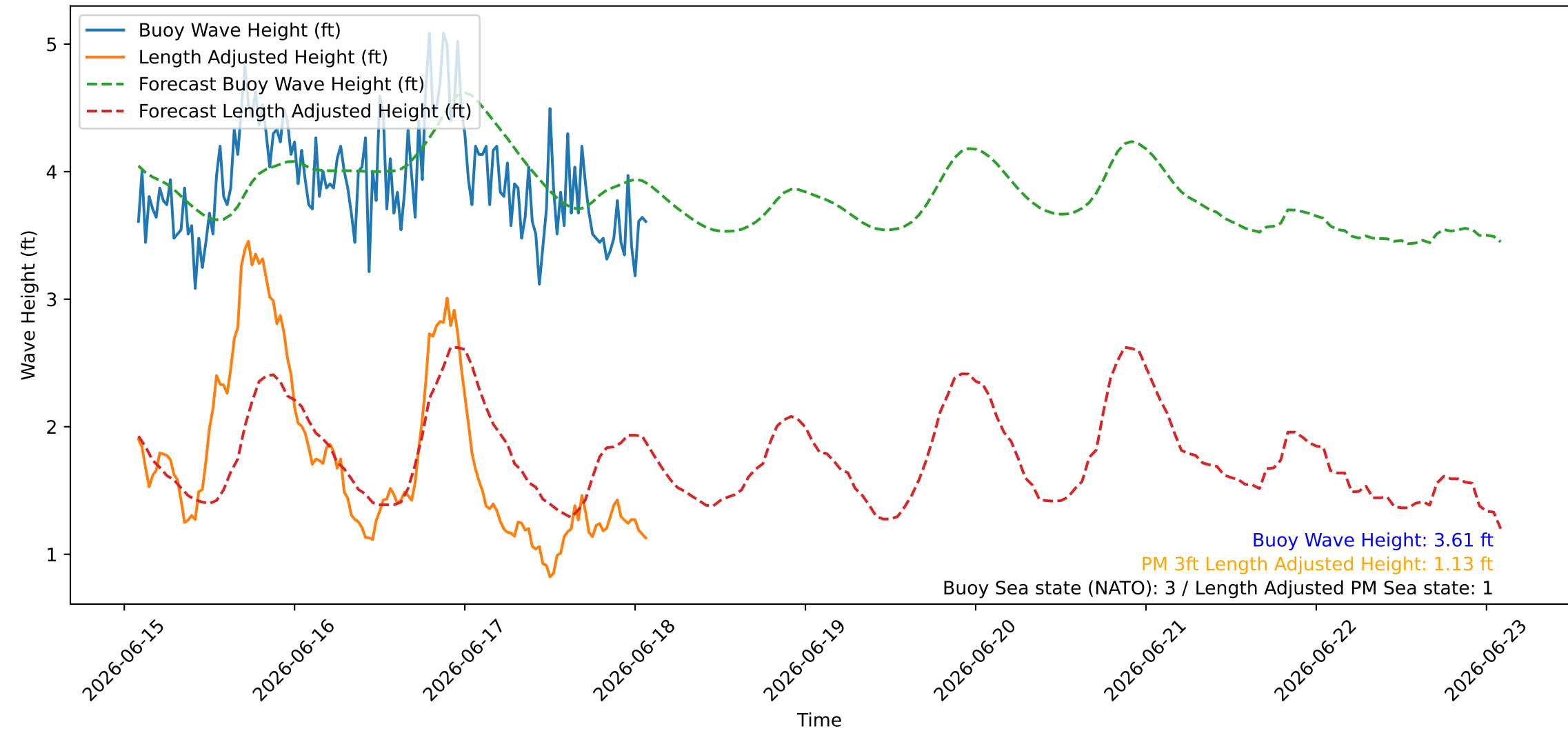
Wave Heights over Time for Green Beach at 2026-06-18 02:11:07
