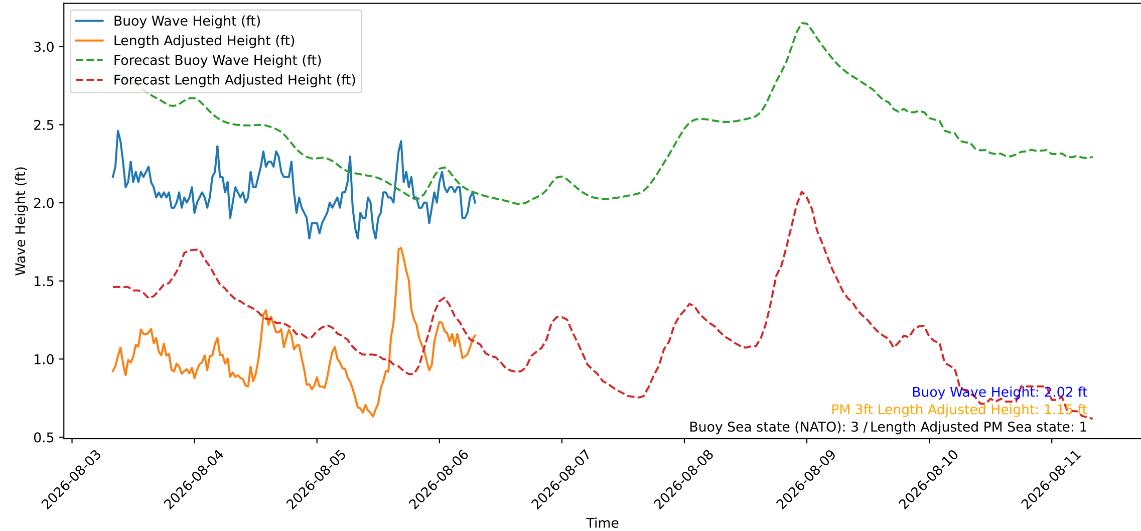
Wave Heights over Time for Red Beach at 2026-08-06 07:50:47
