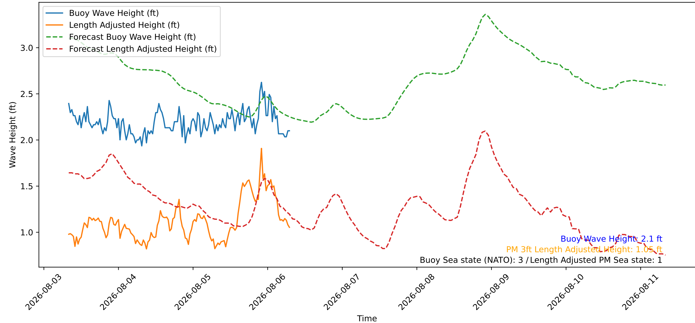
Wave Heights over Time for Green Beach at 2026-08-06 07:51:10
