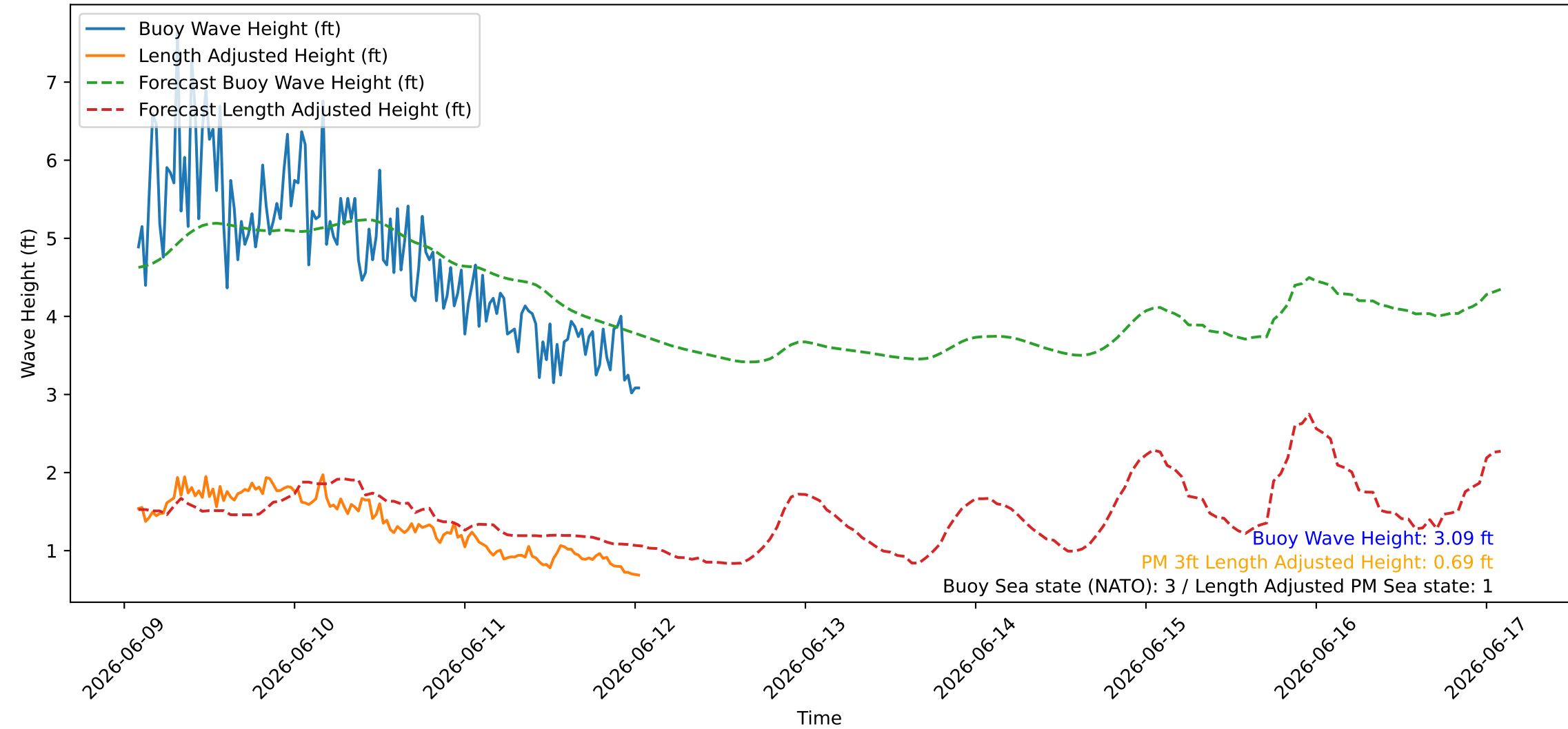
Wave Heights over Time for Red Beach at 2026-06-12 01:30:45
