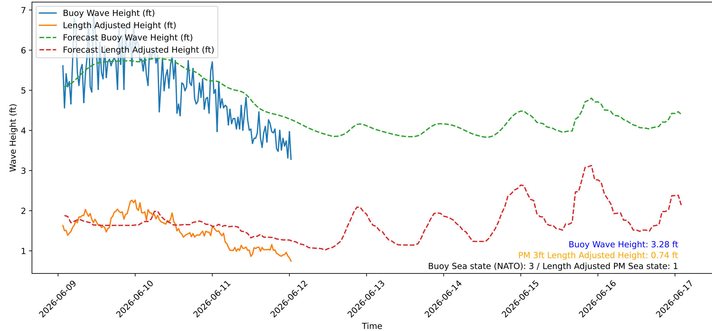
Wave Heights over Time for Green Beach at 2026-06-12 01:31:07
