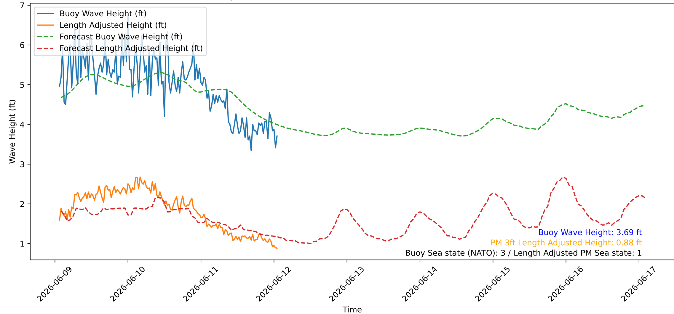
Wave Heights over Time for Oceanside Harbor at 2026-06-12 01:30:26
