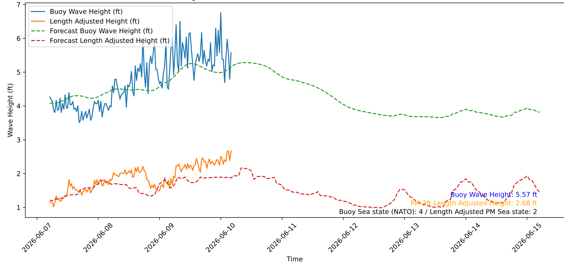
Wave Heights over Time for Oceanside Harbor at 2026-06-10 05:00:26
