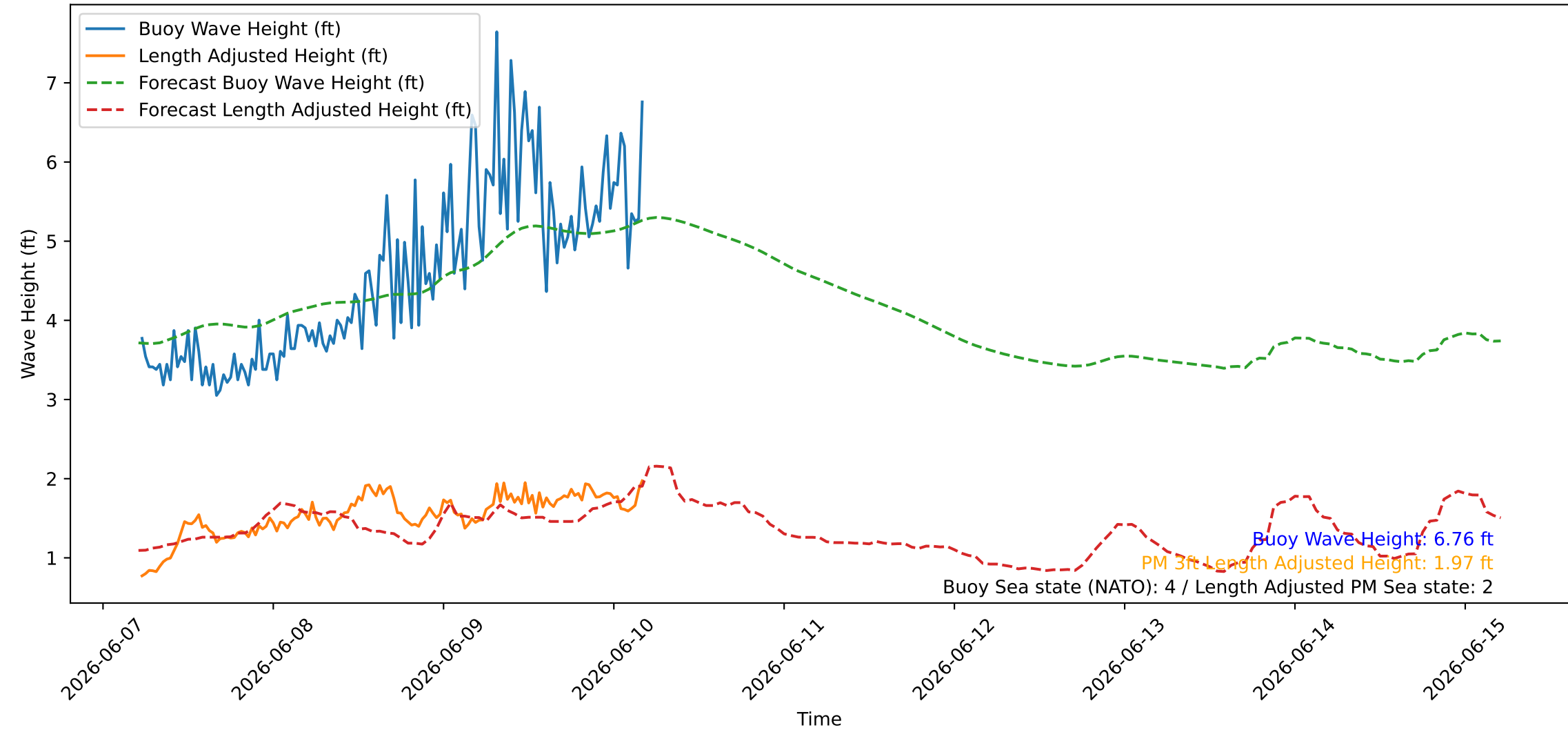
Wave Heights over Time for Red Beach at 2026-06-10 05:00:47
