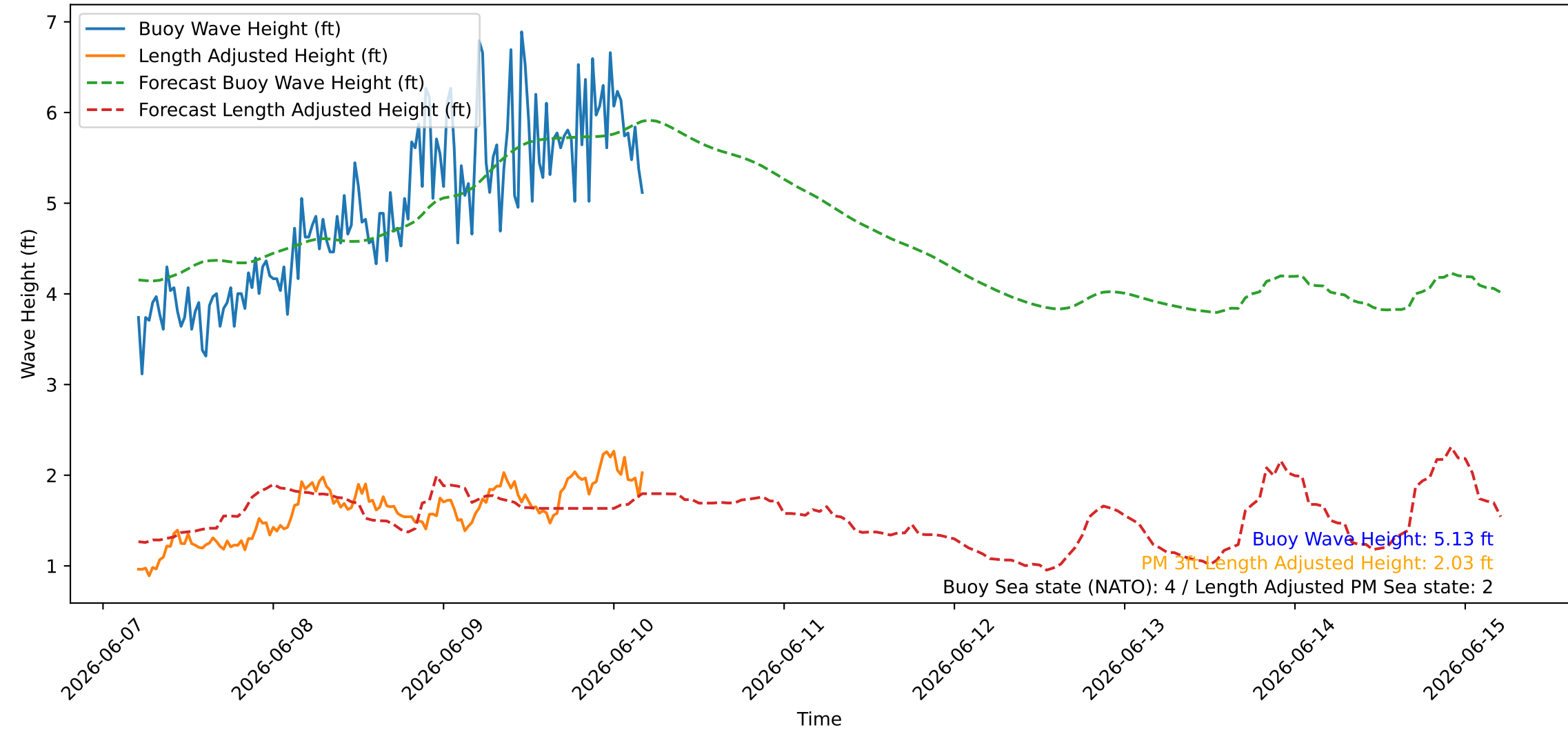
Wave Heights over Time for Green Beach at 2026-06-10 05:01:10
