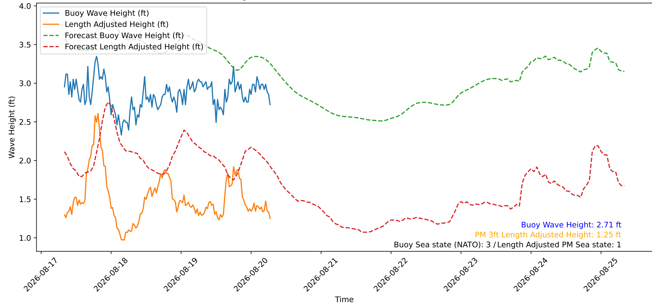
Wave Heights over Time for Red Beach at 2026-08-20 07:30:46
