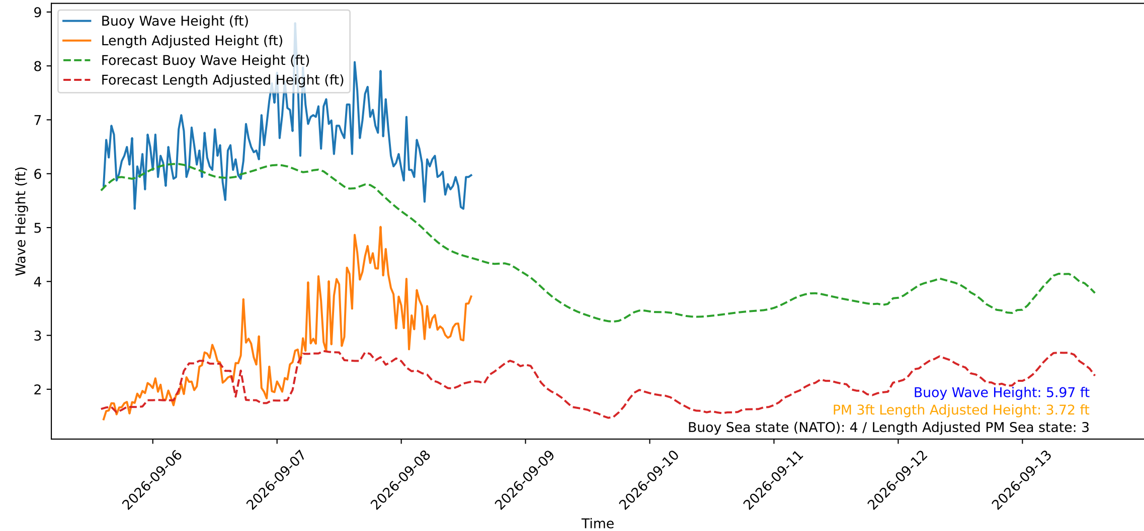
Wave Heights over Time for Green Beach at 2026-09-08 14:21:15
