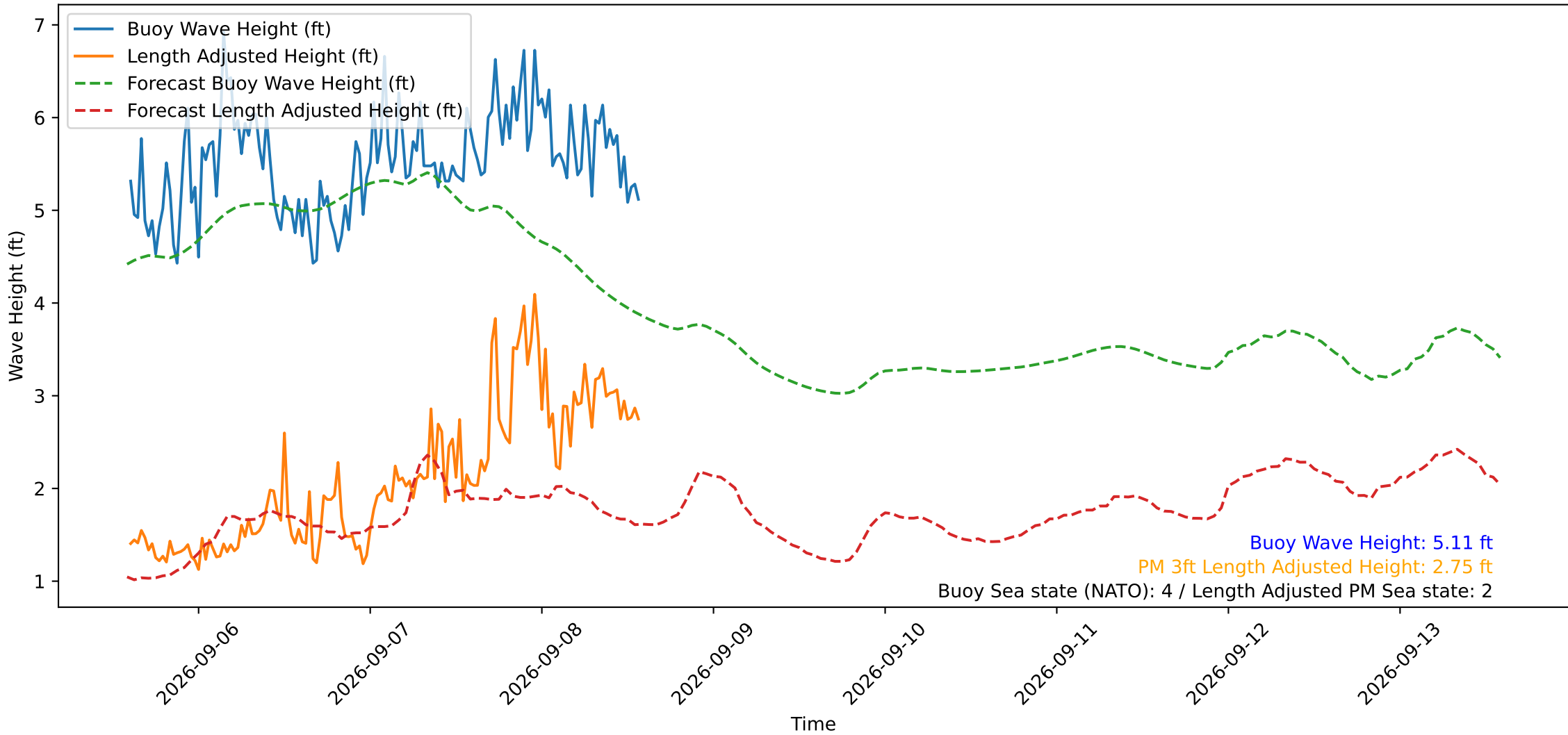
Wave Heights over Time for Red Beach at 2026-09-08 14:20:51
