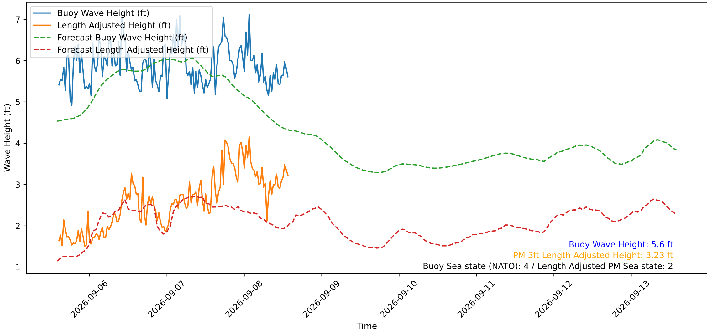
Wave Heights over Time for Oceanside Harbor at 2026-09-08 14:20:30
