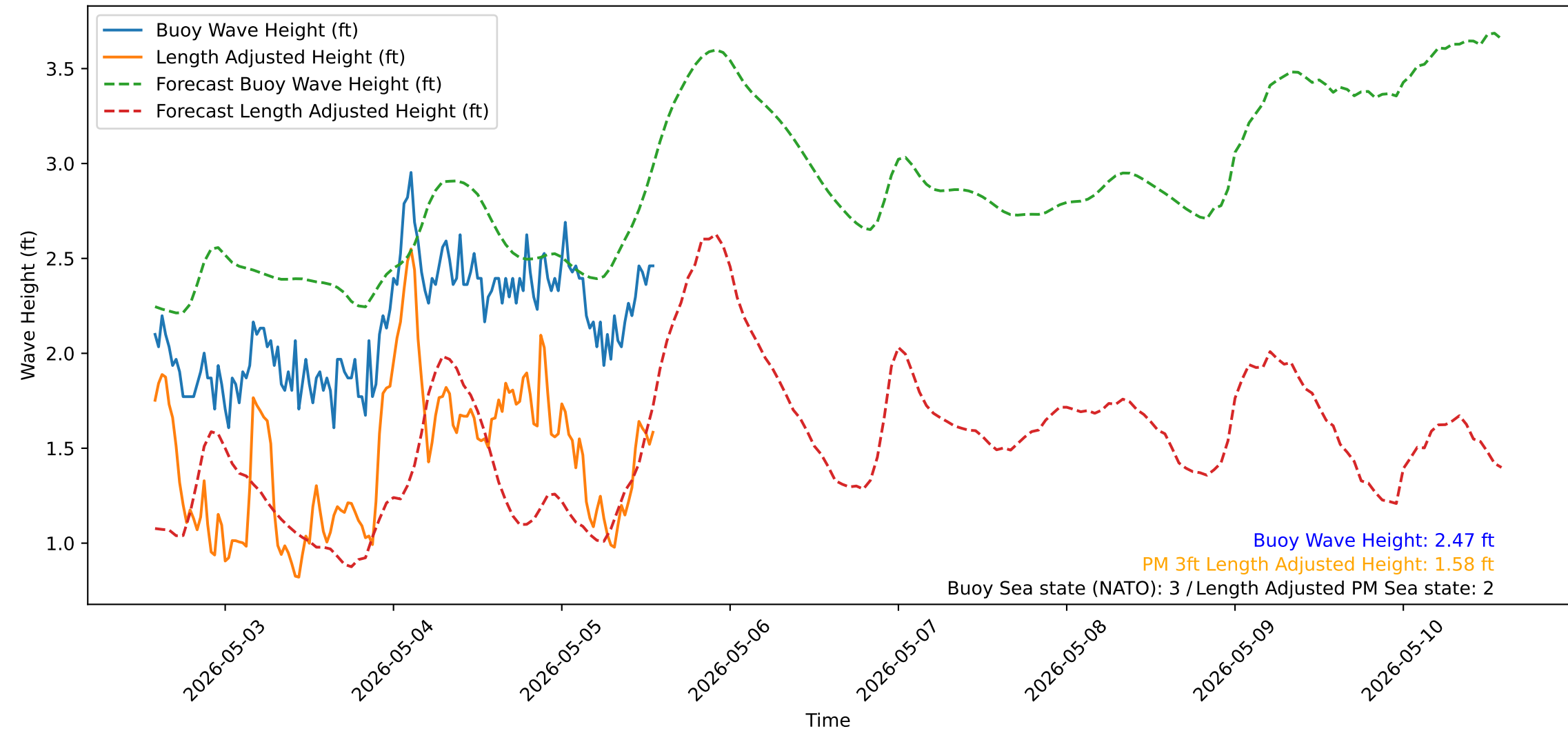
Wave Heights over Time for Red Beach at 2026-05-05 13:50:52
