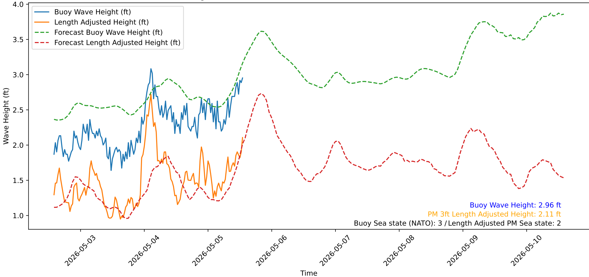
Wave Heights over Time for Oceanside Harbor at 2026-05-05 13:50:32
