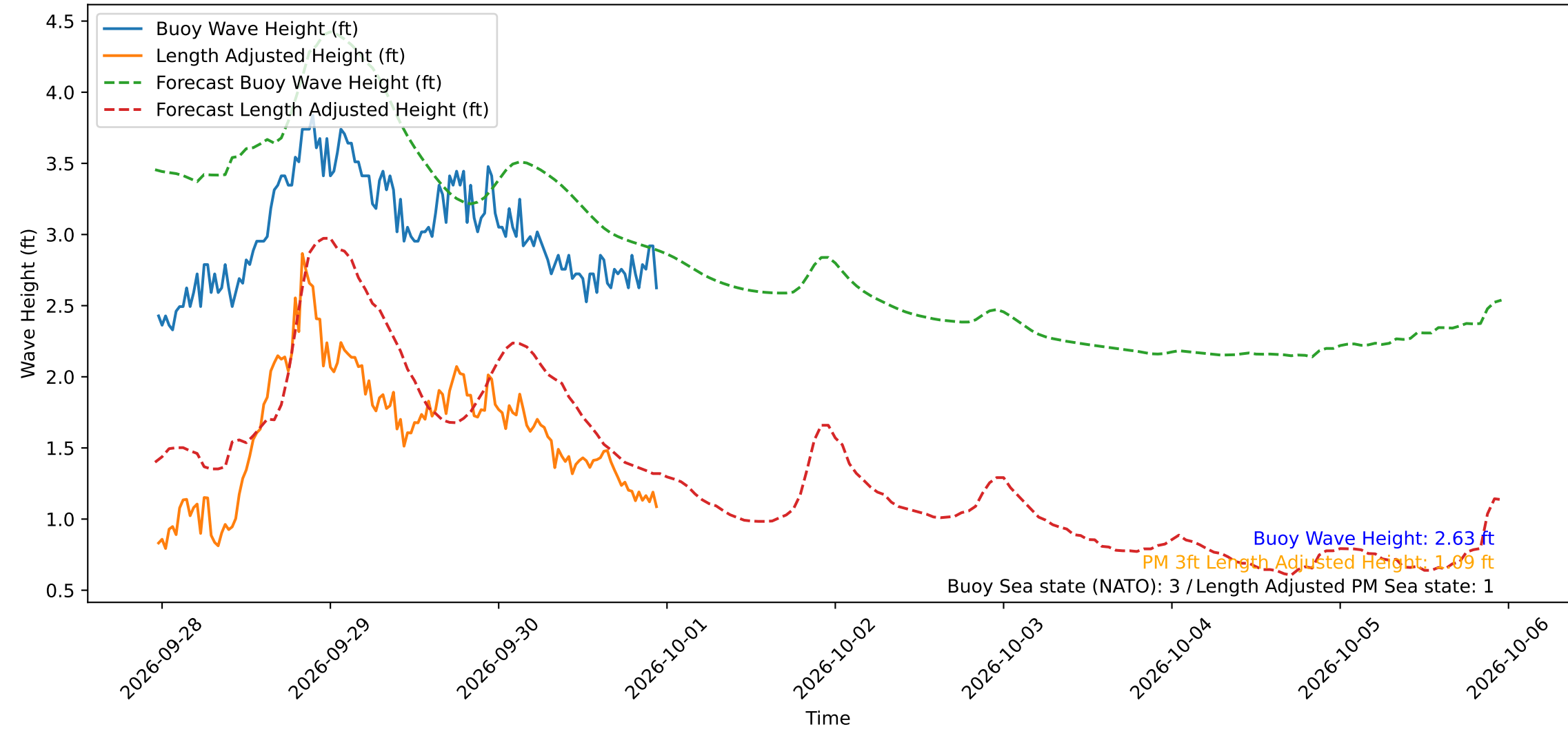
Wave Heights over Time for Red Beach at 2026-09-30 23:10:50
