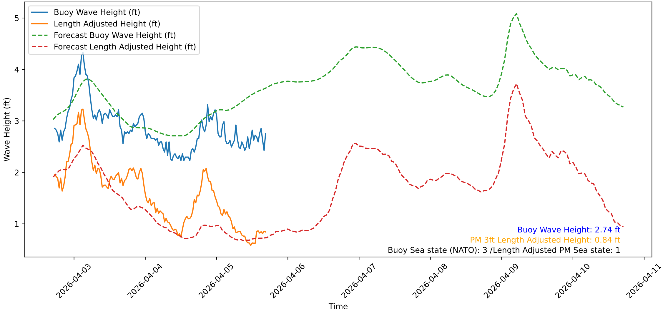
Wave Heights over Time for Green Beach at 2026-04-05 17:21:15
