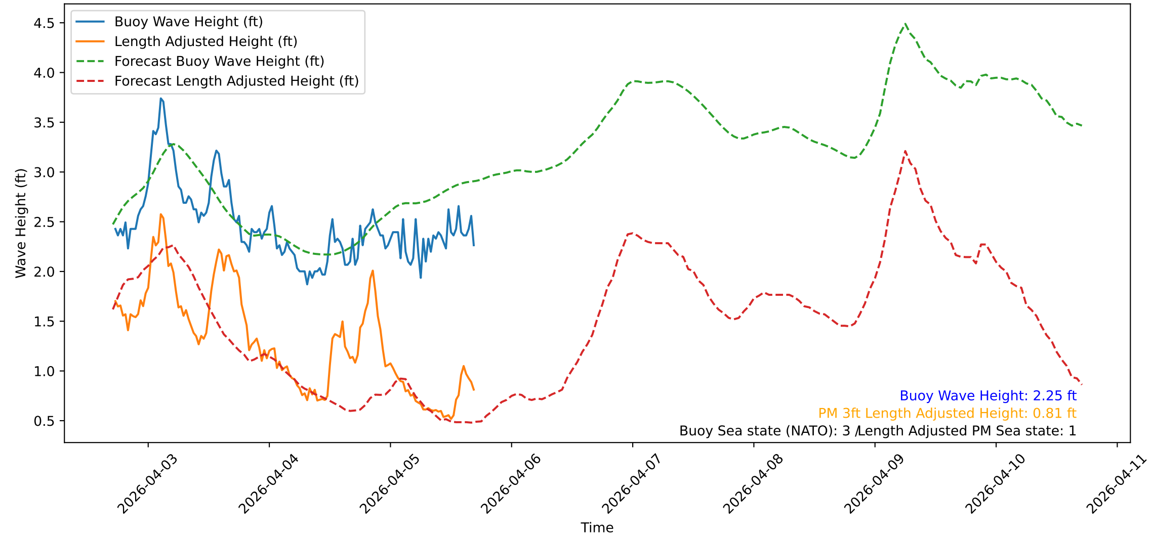
Wave Heights over Time for Red Beach at 2026-04-05 17:20:50
