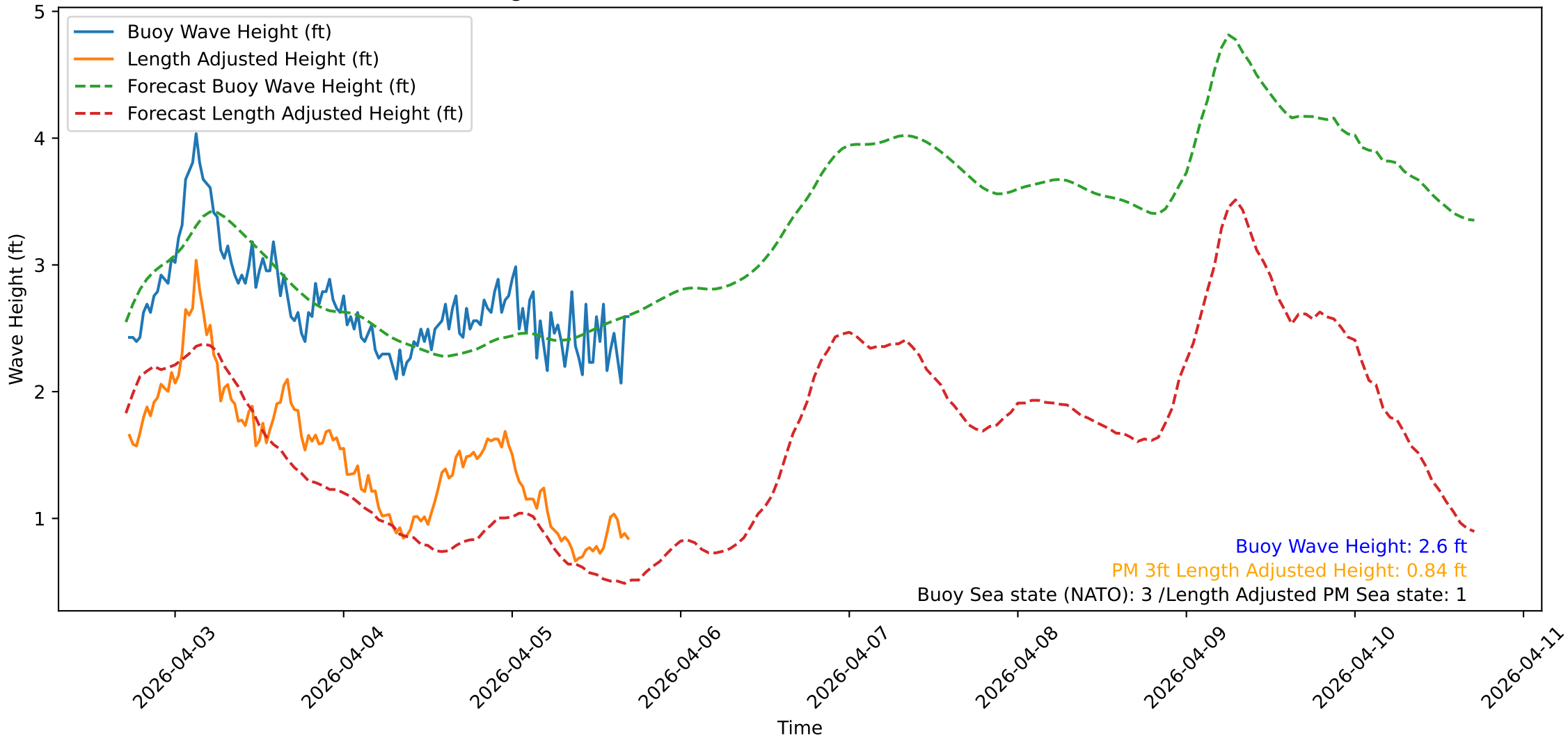
Wave Heights over Time for Oceanside Harbor at 2026-04-05 17:20:33
