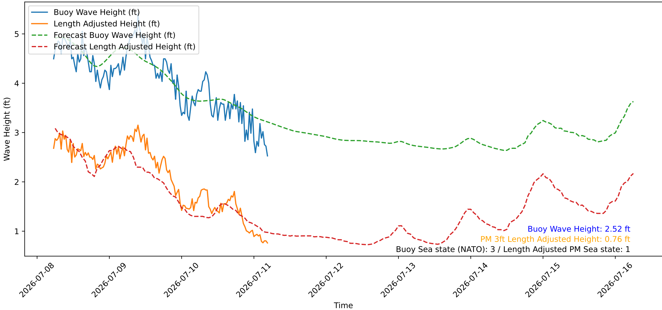
Wave Heights over Time for Oceanside Harbor at 2026-07-11 05:40:26
