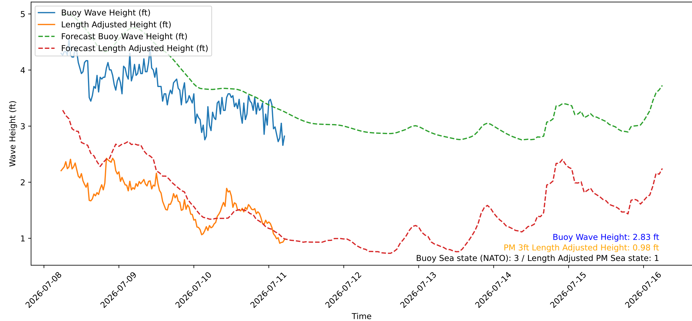
Wave Heights over Time for Green Beach at 2026-07-11 05:41:08
