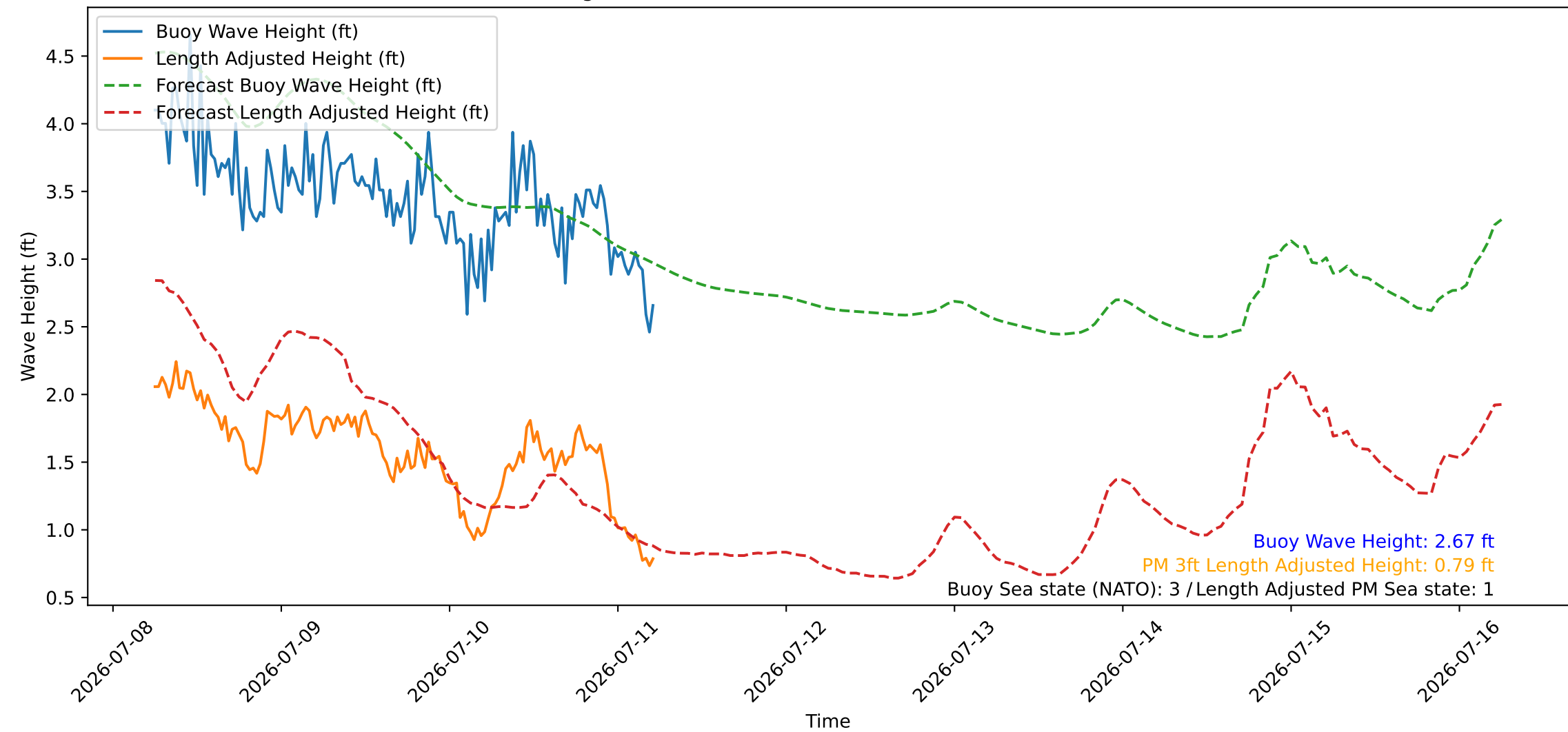
Wave Heights over Time for Red Beach at 2026-07-11 05:40:46
