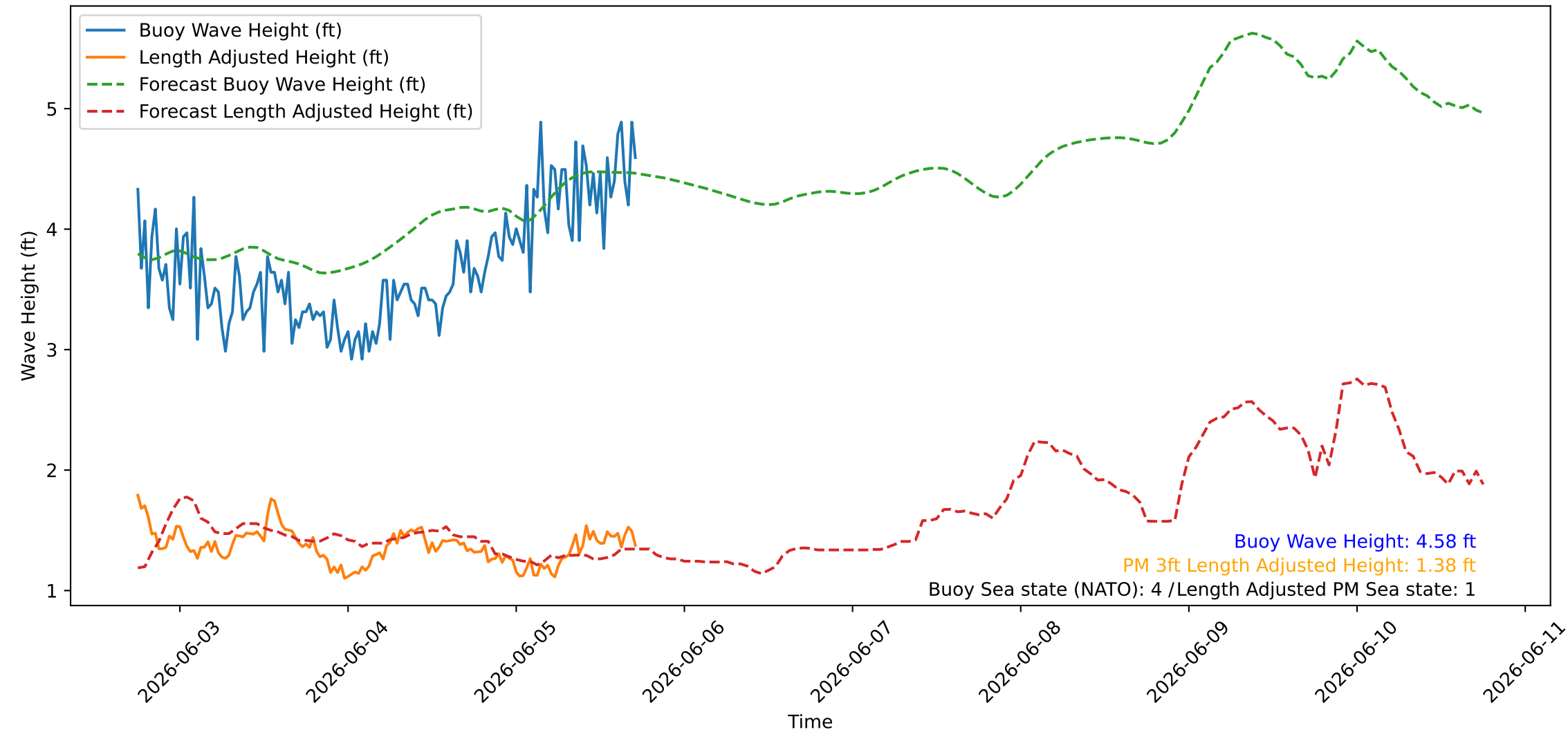
Wave Heights over Time for Oceanside Harbor at 2026-06-05 17:50:26
