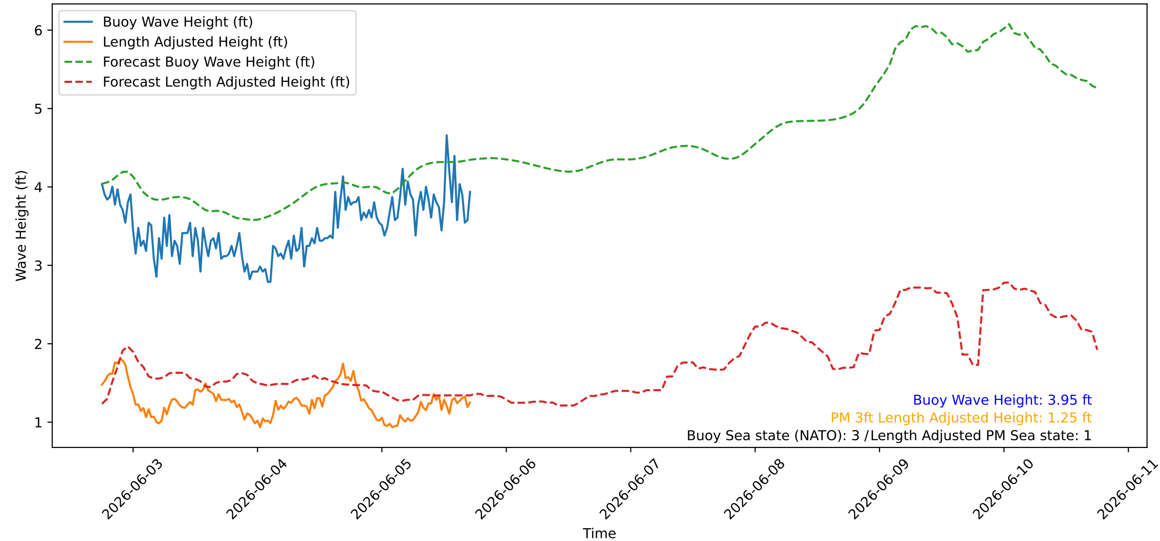
Wave Heights over Time for Green Beach at 2026-06-05 17:51:09
