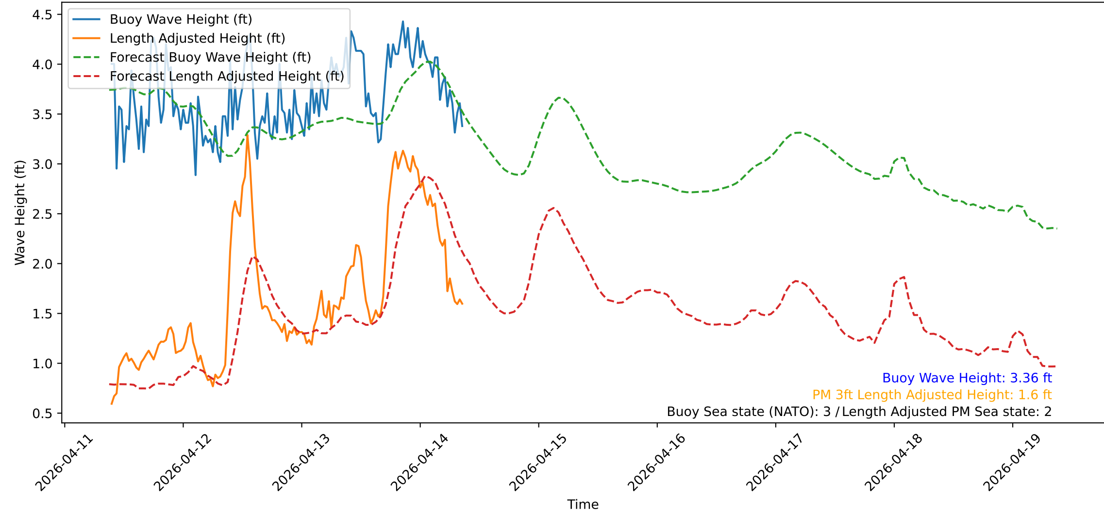
Wave Heights over Time for Red Beach at 2026-04-14 09:20:50
