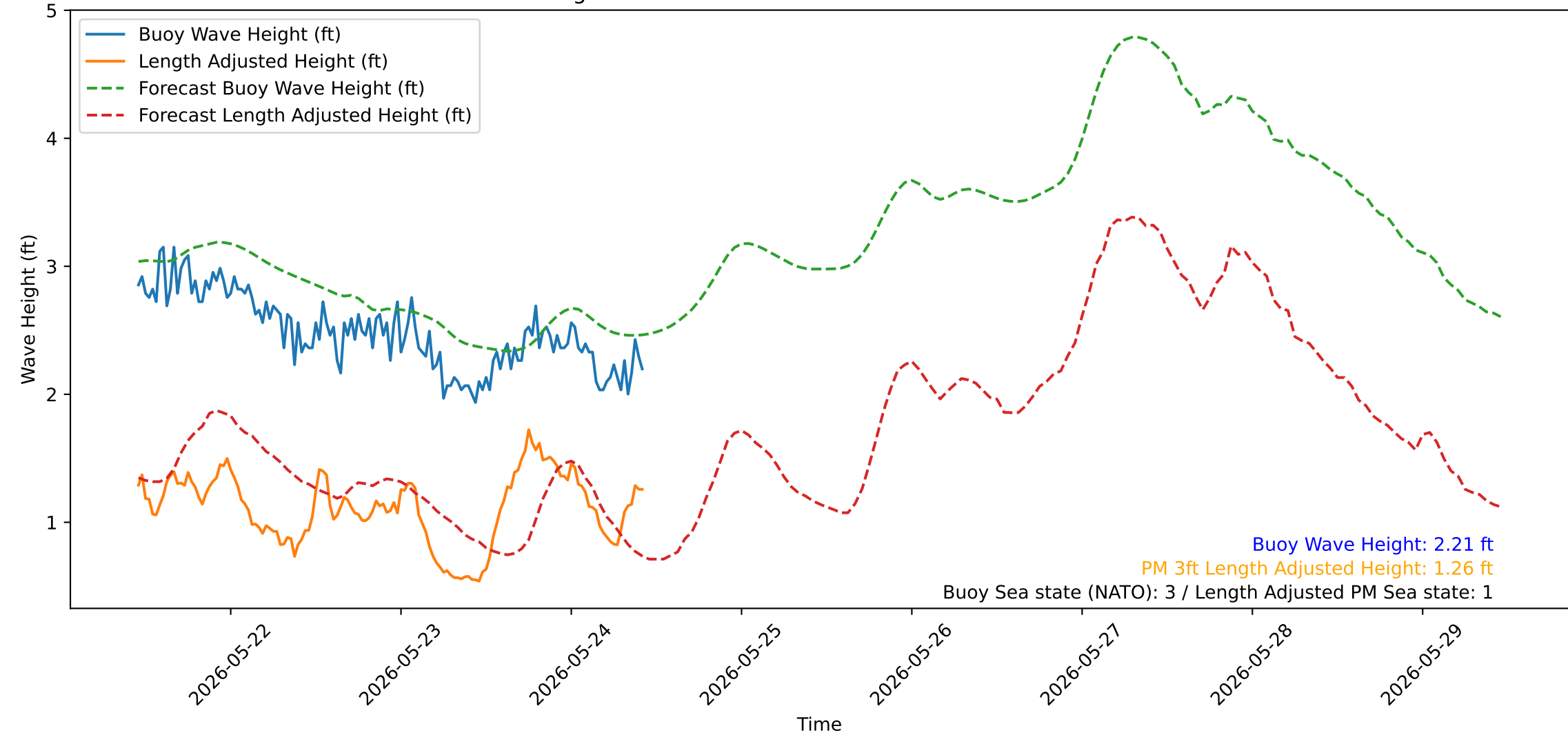
Wave Heights over Time for Red Beach at 2026-05-24 10:40:52
