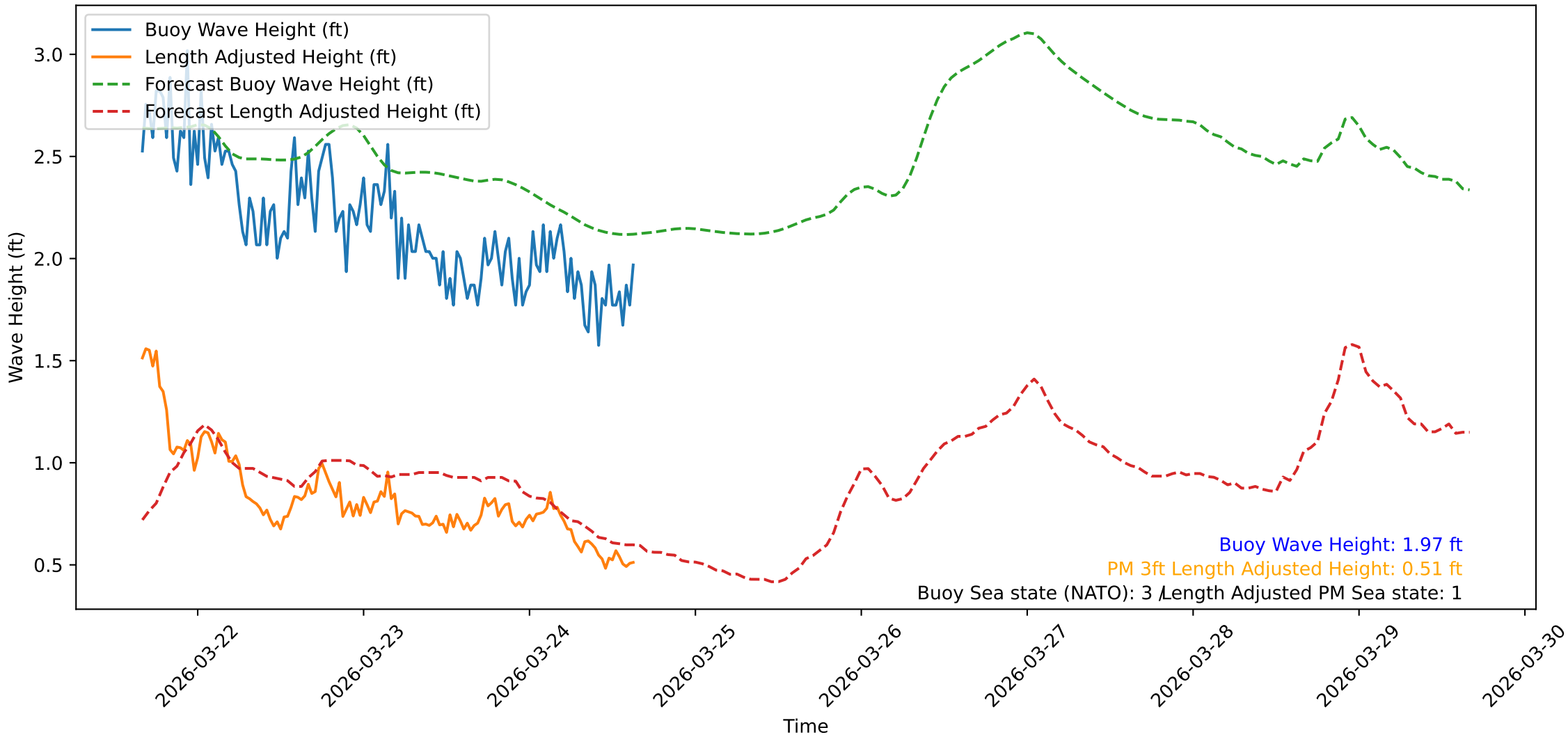
Wave Heights over Time for Oceanside Harbor at 2026-03-24 15:50:31
