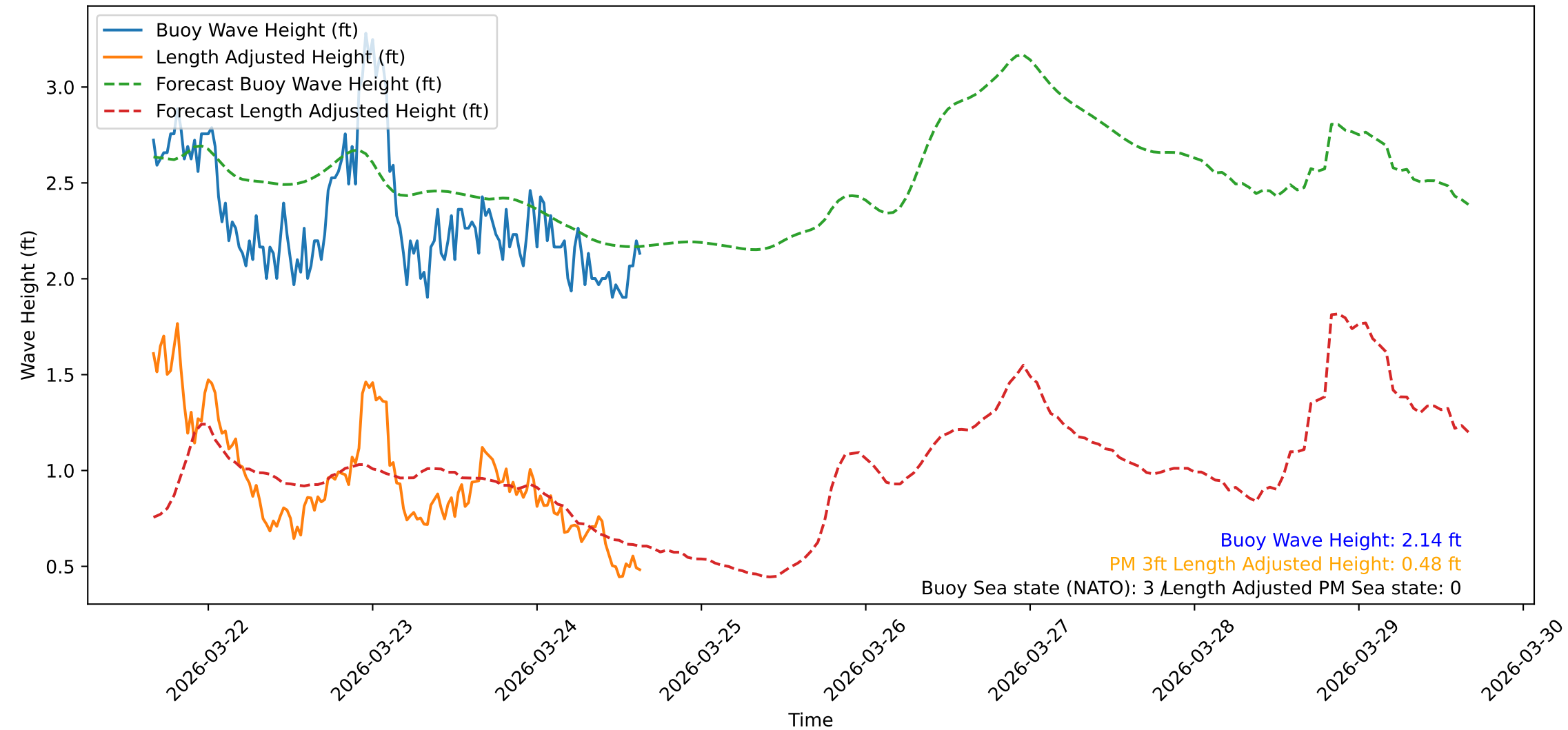
Wave Heights over Time for Green Beach at 2026-03-24 15:51:10
