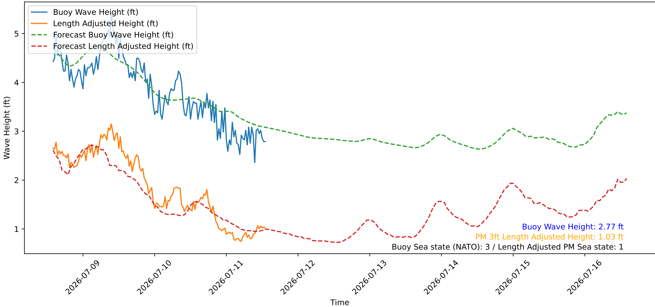
Wave Heights over Time for Oceanside Harbor at 2026-07-11 14:00:26
