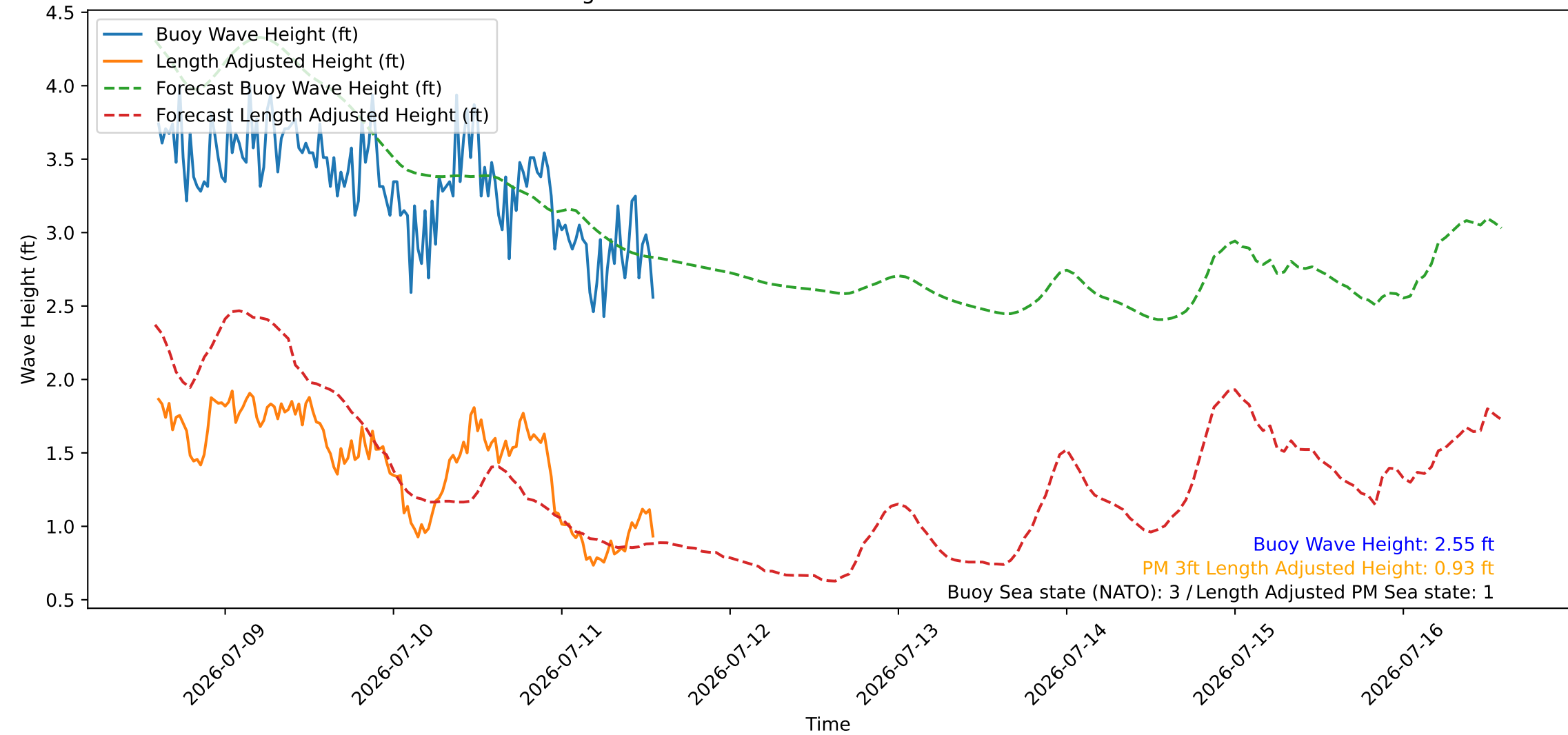
Wave Heights over Time for Red Beach at 2026-07-11 14:00:45
