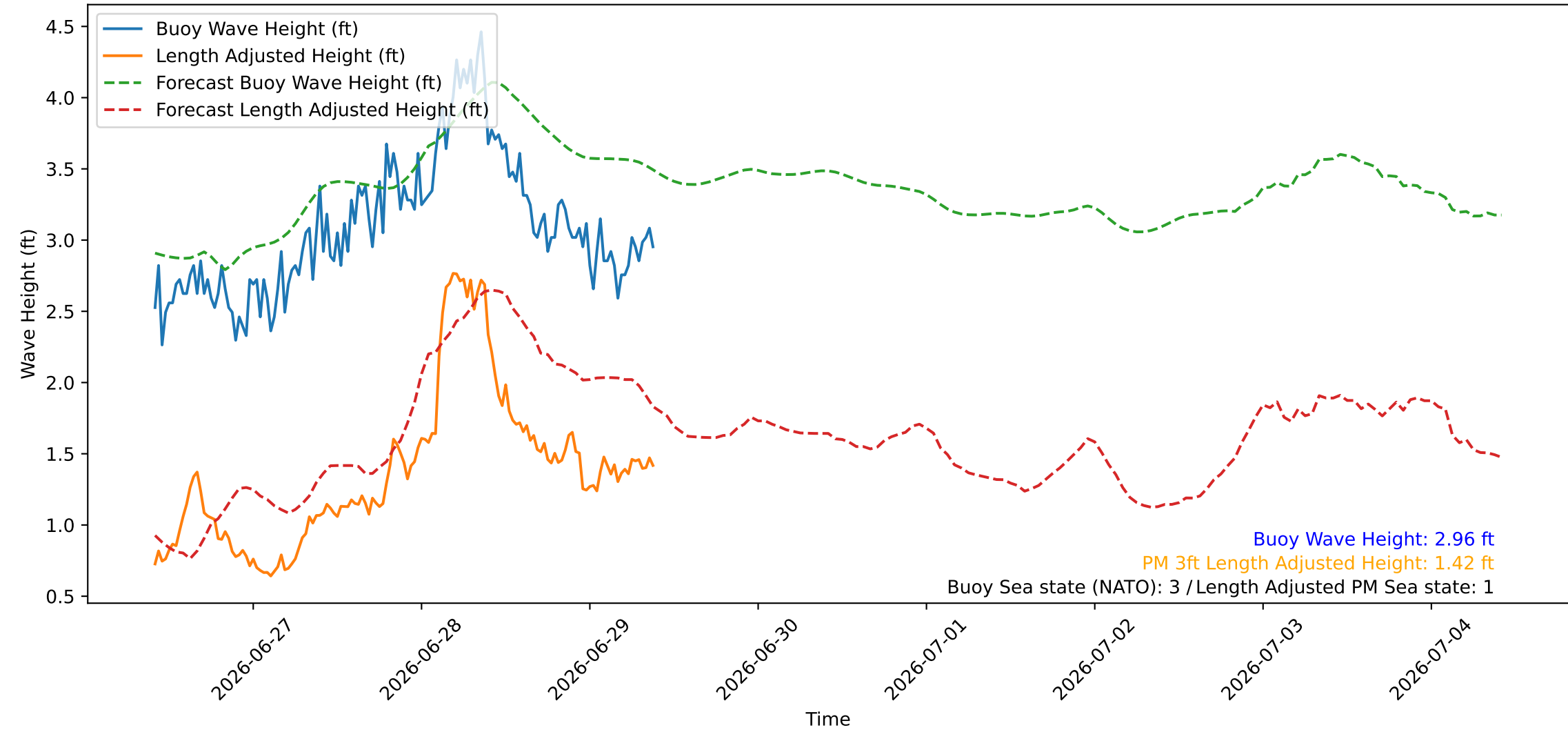
Wave Heights over Time for Red Beach at 2026-06-29 09:50:46
