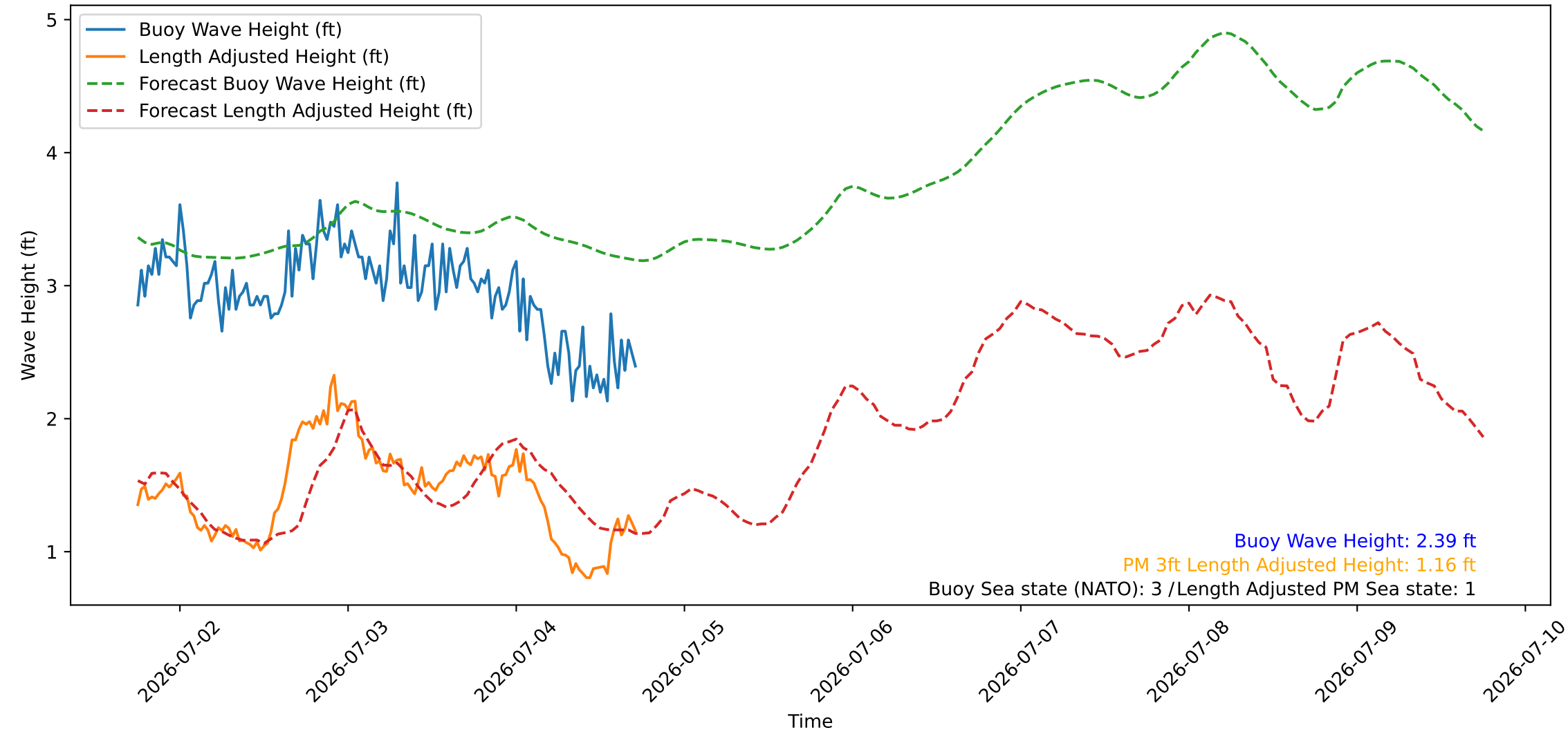
Wave Heights over Time for Oceanside Harbor at 2026-07-04 18:10:26
