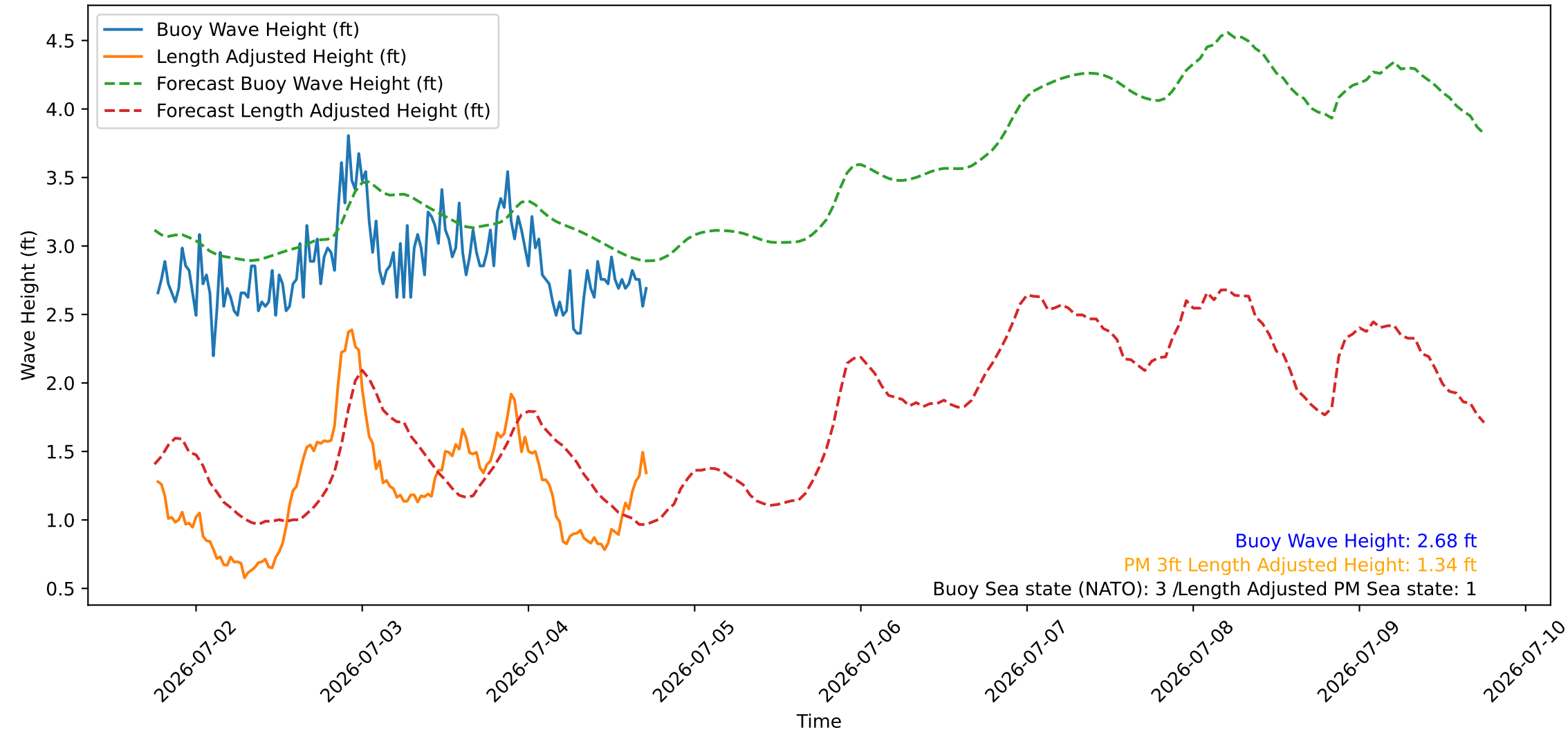
Wave Heights over Time for Red Beach at 2026-07-04 18:10:46
