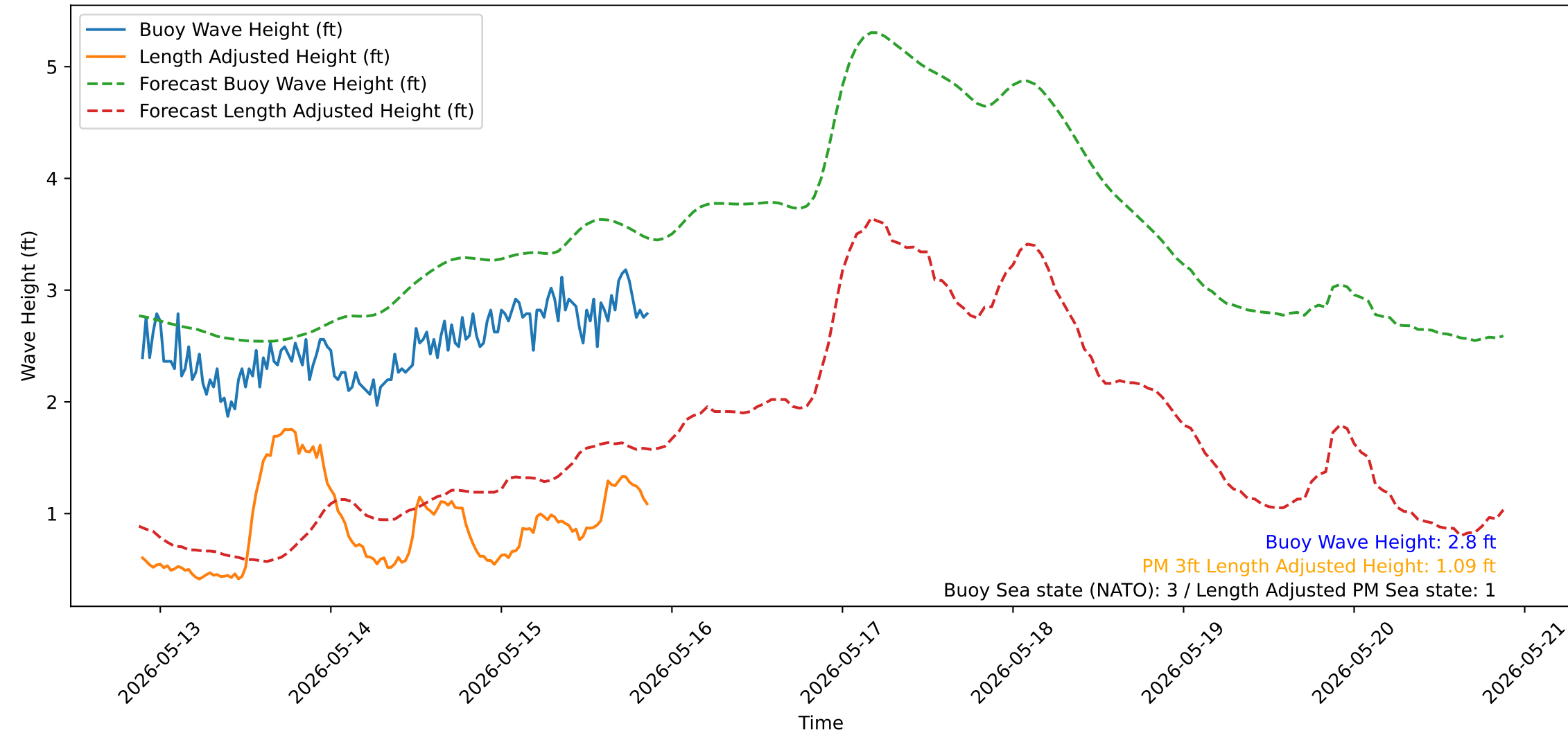
Wave Heights over Time for Red Beach at 2026-05-15 21:20:51
