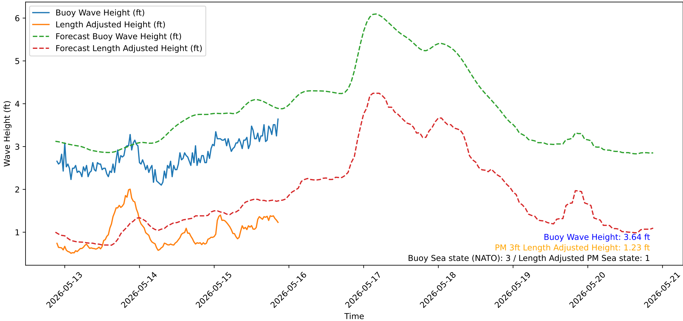
Wave Heights over Time for Green Beach at 2026-05-15 21:21:14
