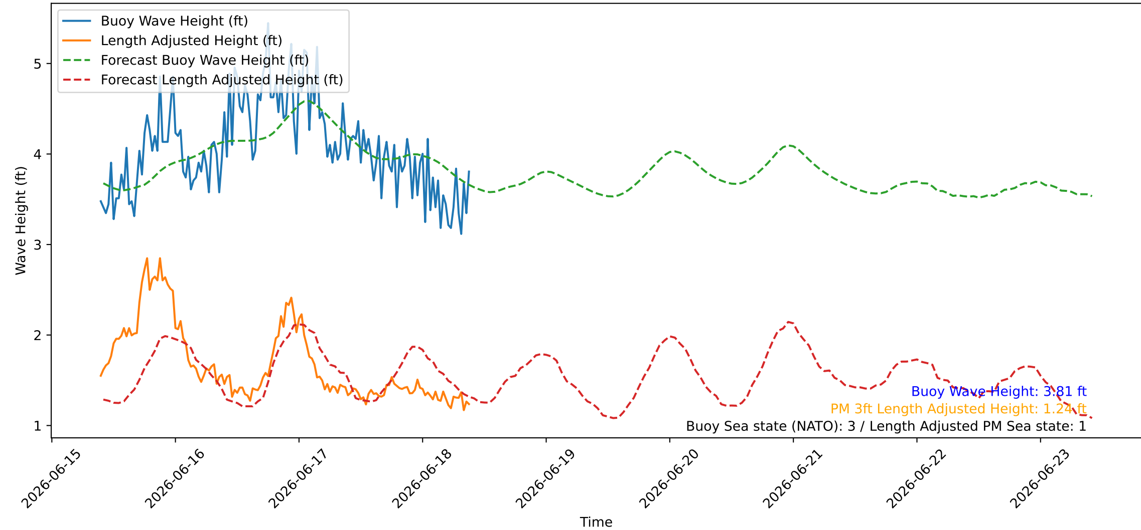
Wave Heights over Time for Oceanside Harbor at 2026-06-18 09:40:26
