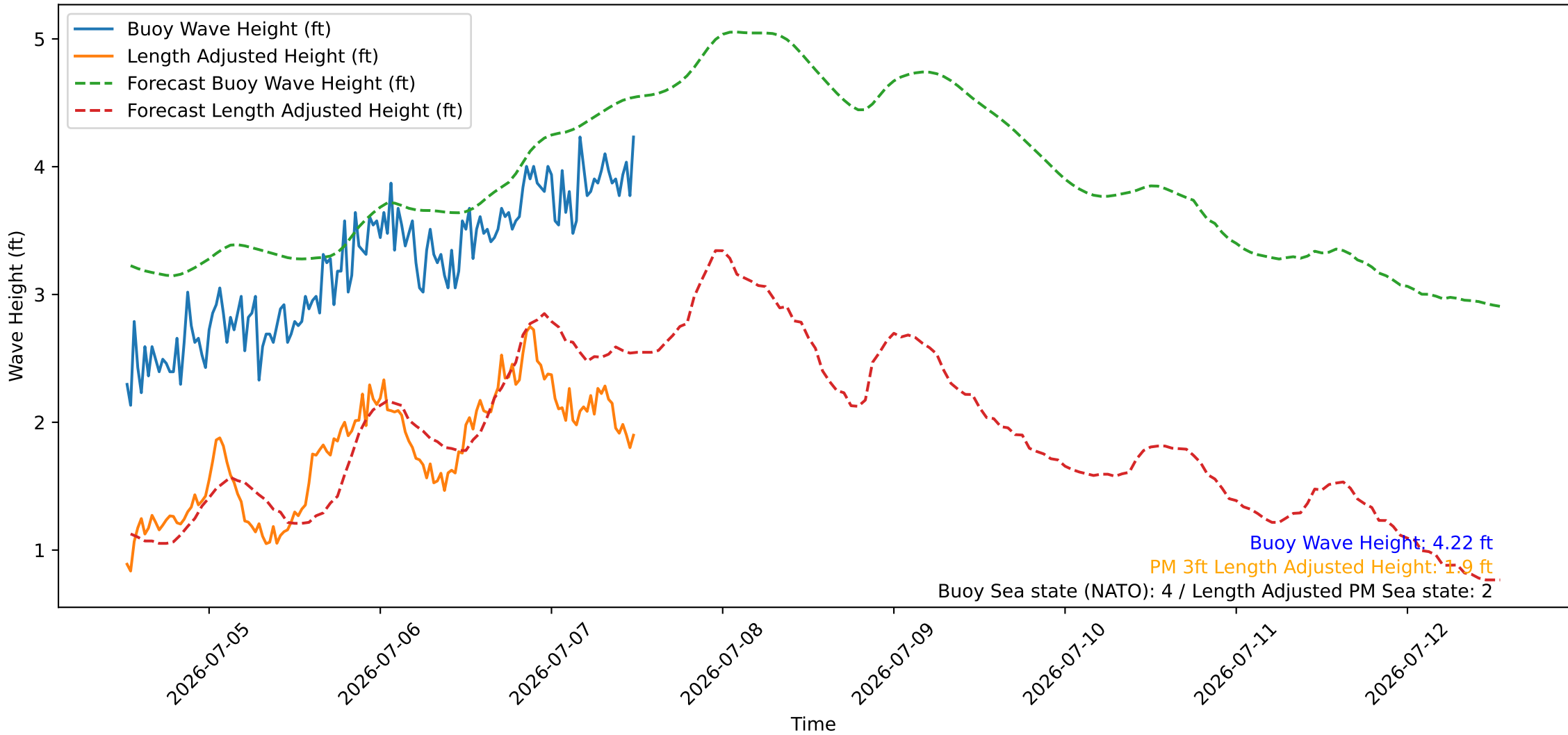
Wave Heights over Time for Oceanside Harbor at 2026-07-07 12:40:26
