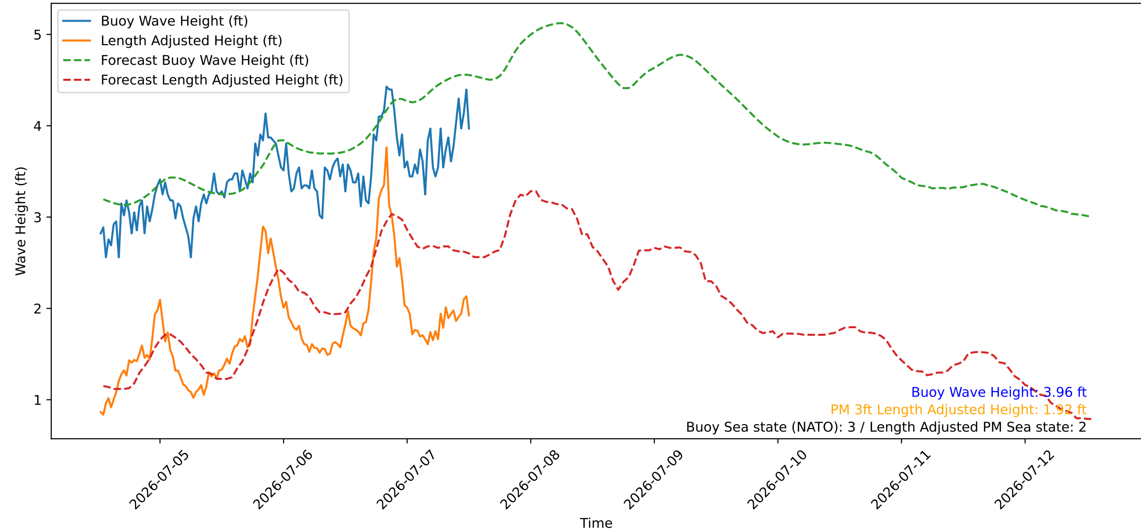
Wave Heights over Time for Green Beach at 2026-07-07 12:41:09
