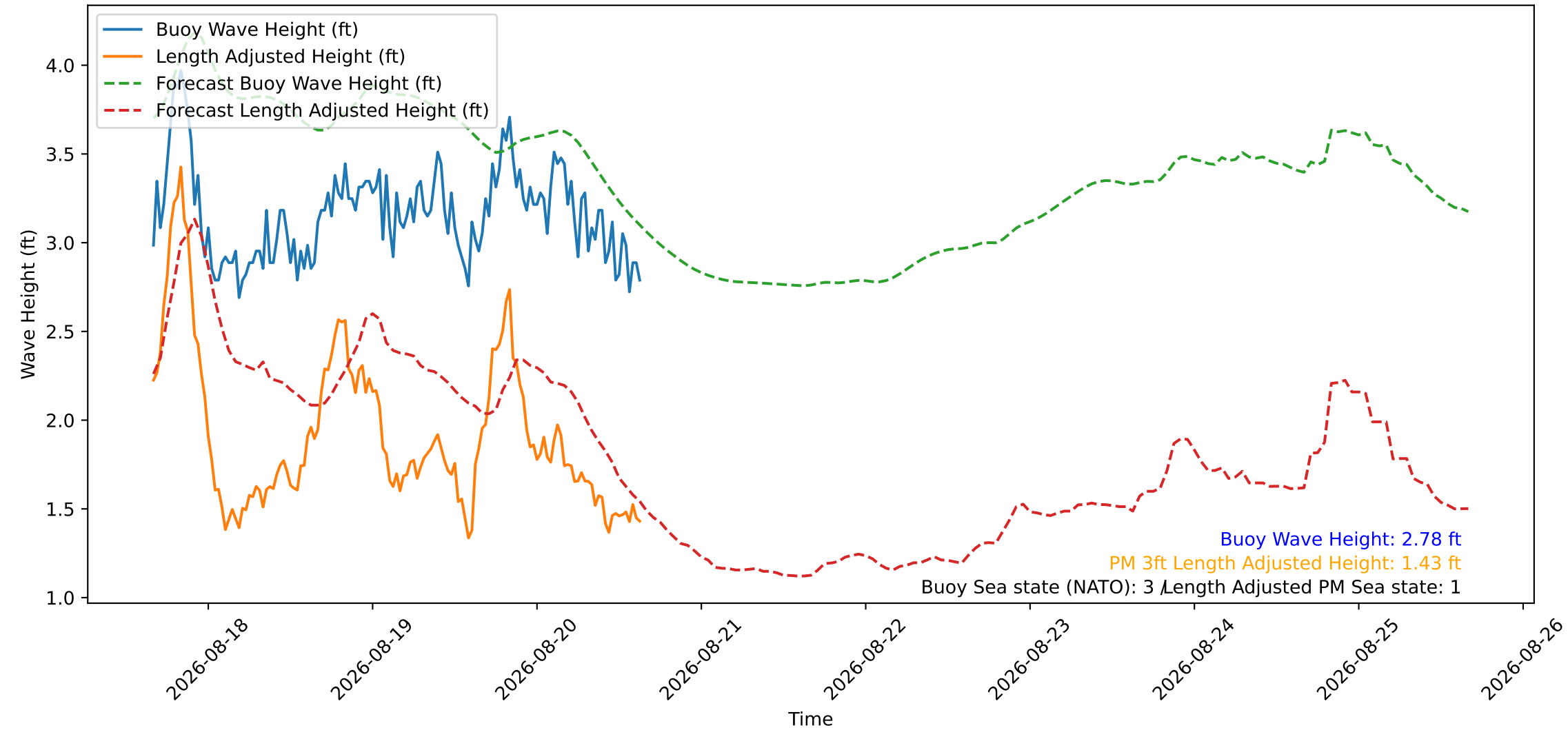
Wave Heights over Time for Green Beach at 2026-08-20 15:51:11
