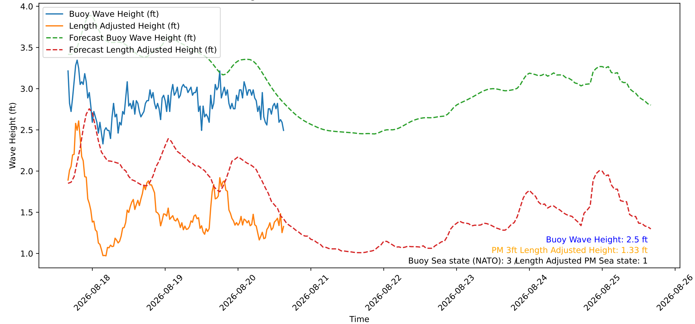
Wave Heights over Time for Red Beach at 2026-08-20 15:50:47
