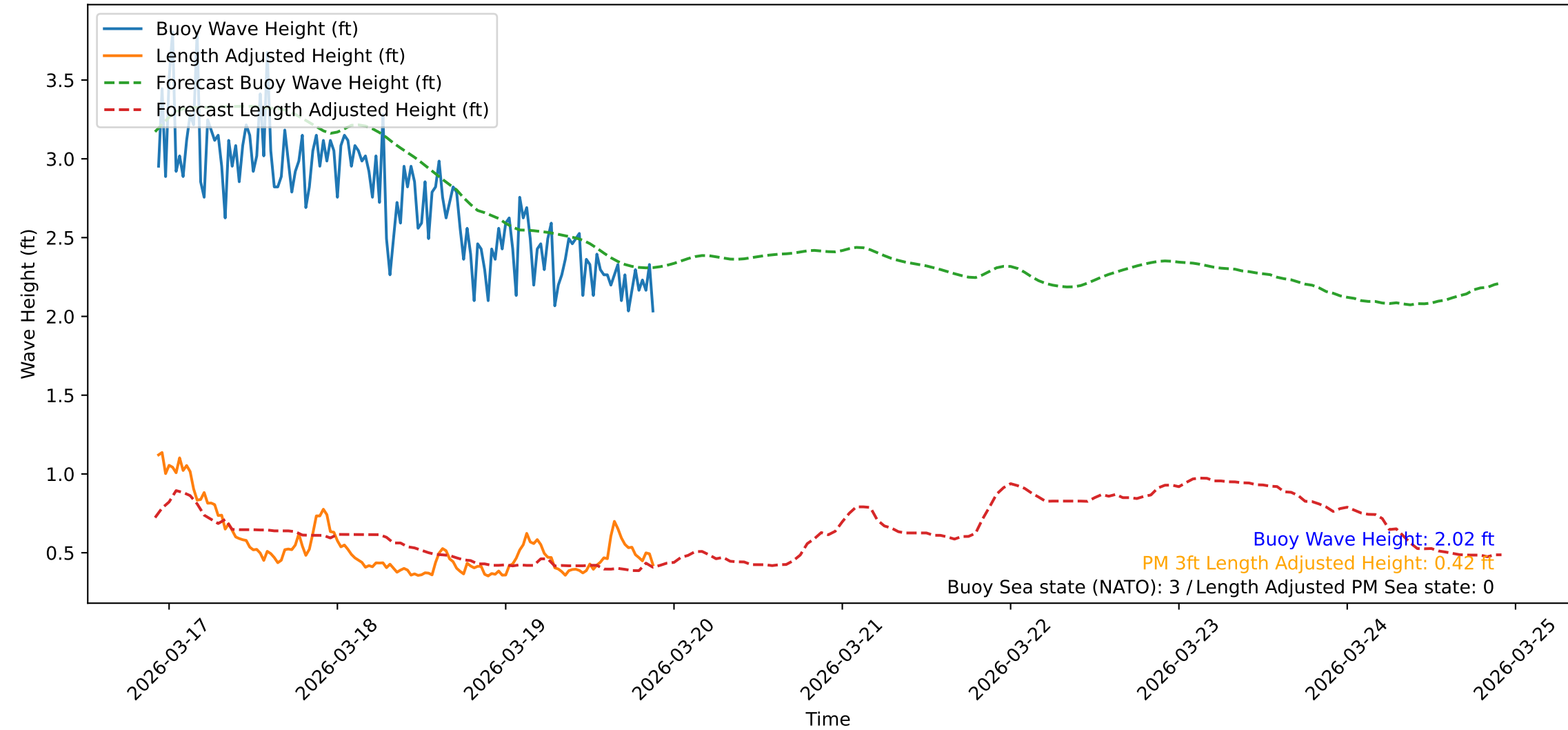
Wave Heights over Time for Red Beach at 2026-03-19 22:00:48
