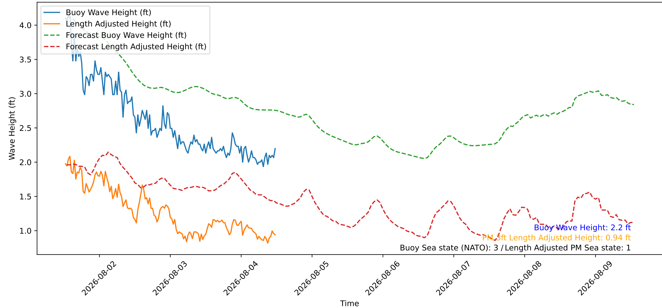
Wave Heights over Time for Green Beach at 2026-08-04 12:31:09
