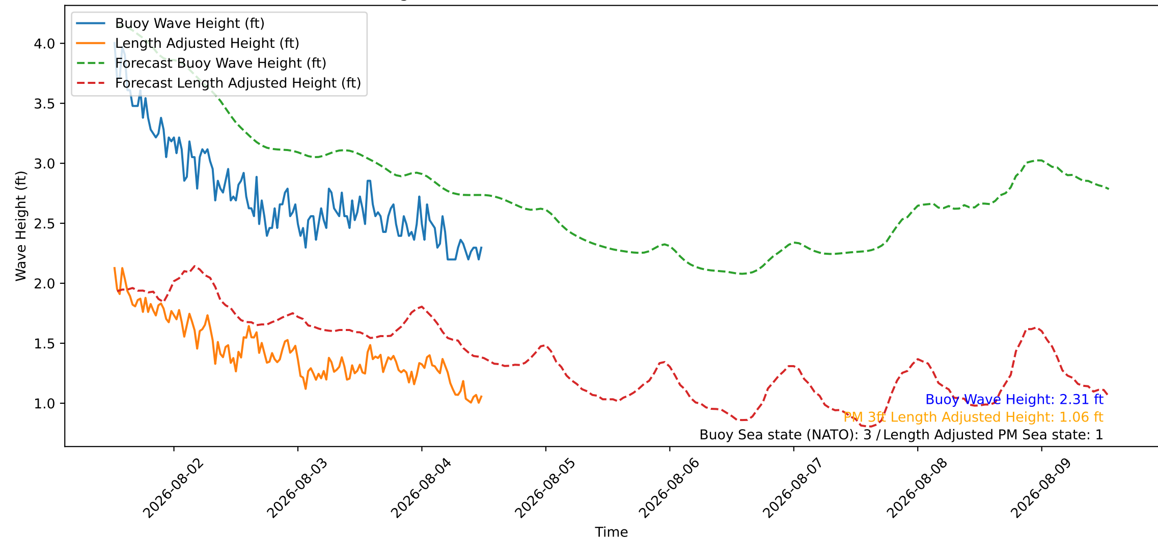
Wave Heights over Time for Oceanside Harbor at 2026-08-04 12:30:27
