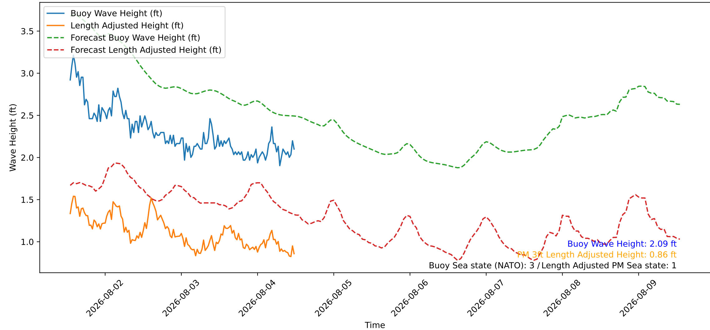
Wave Heights over Time for Red Beach at 2026-08-04 12:30:46
