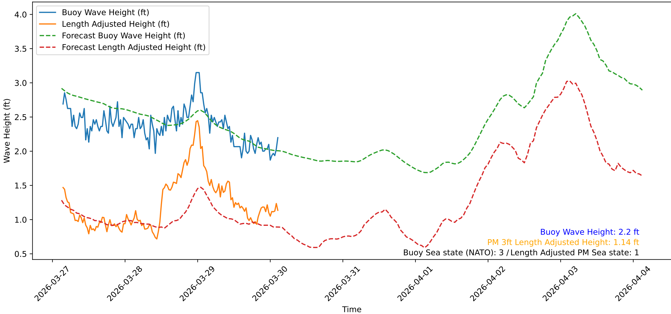
Wave Heights over Time for Oceanside Harbor at 2026-03-30 03:20:31
