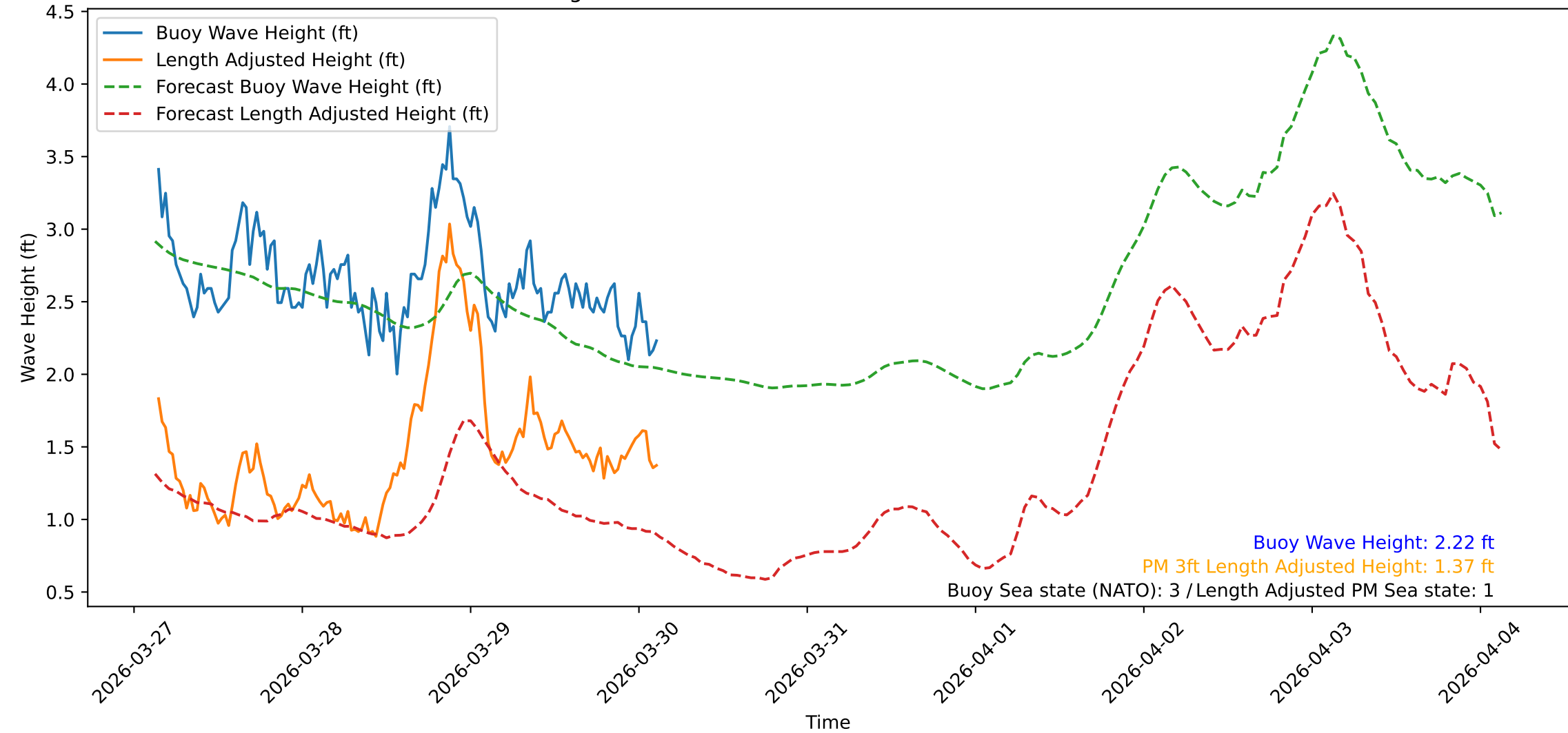
Wave Heights over Time for Green Beach at 2026-03-30 03:21:10
