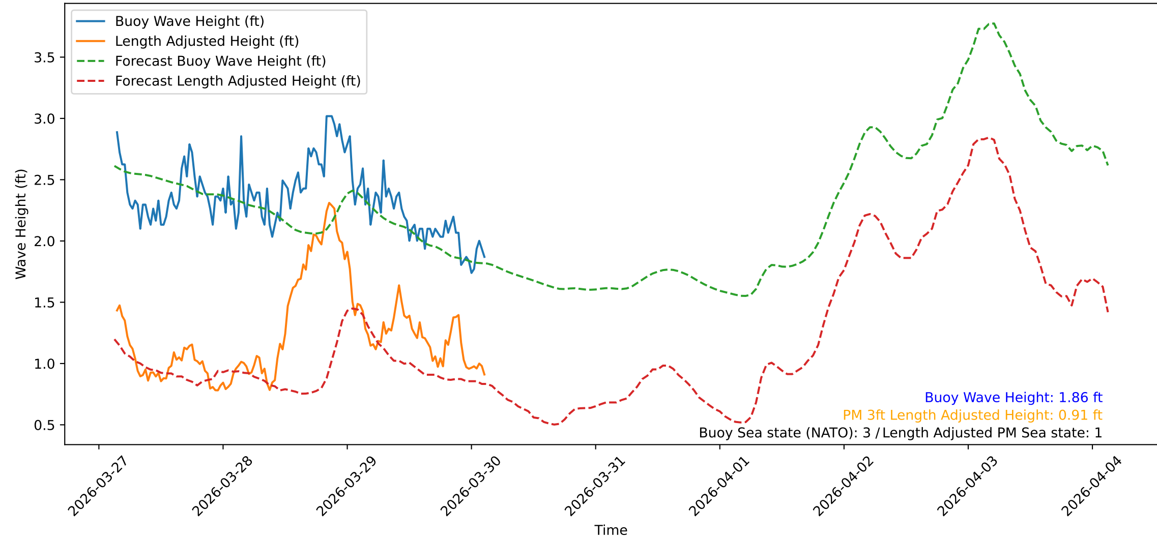
Wave Heights over Time for Red Beach at 2026-03-30 03:20:47
