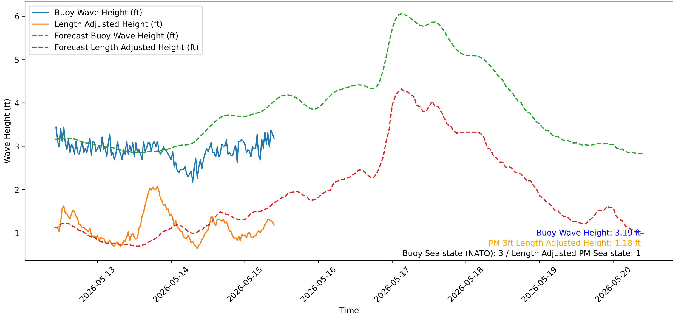
Wave Heights over Time for Oceanside Harbor at 2026-05-15 10:20:32
