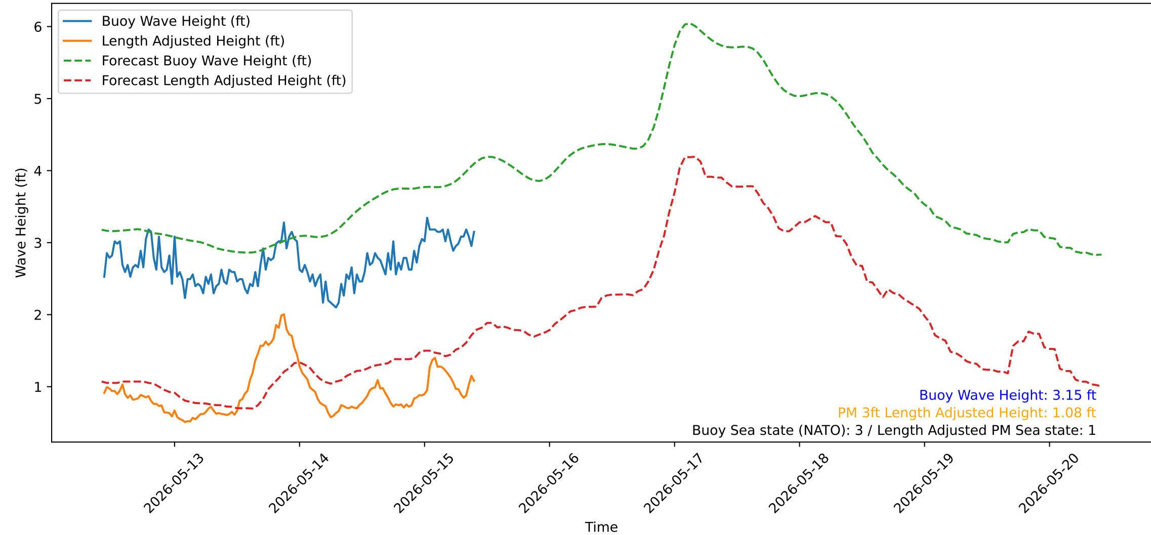
Wave Heights over Time for Green Beach at 2026-05-15 10:21:15
