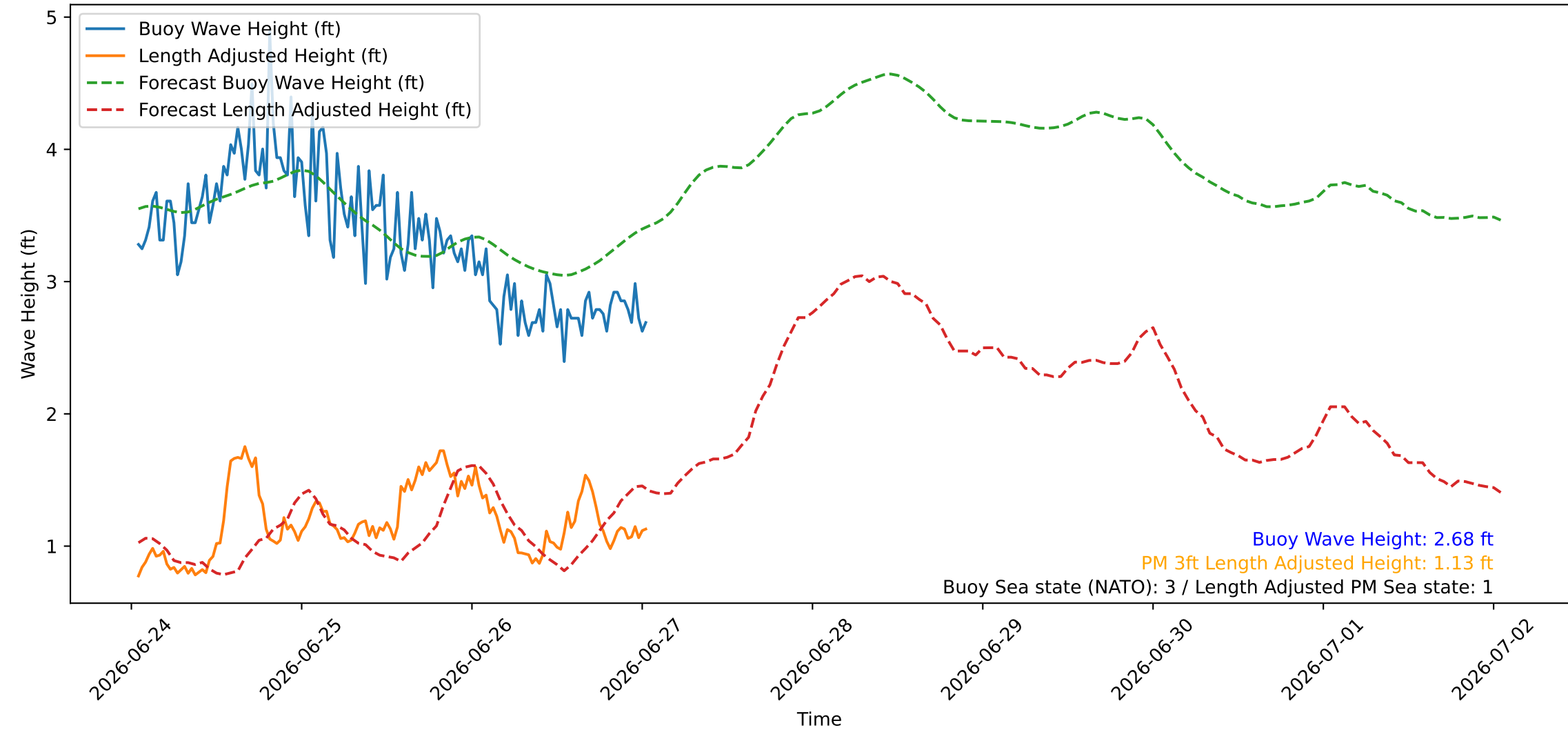
Wave Heights over Time for Oceanside Harbor at 2026-06-27 01:10:26
