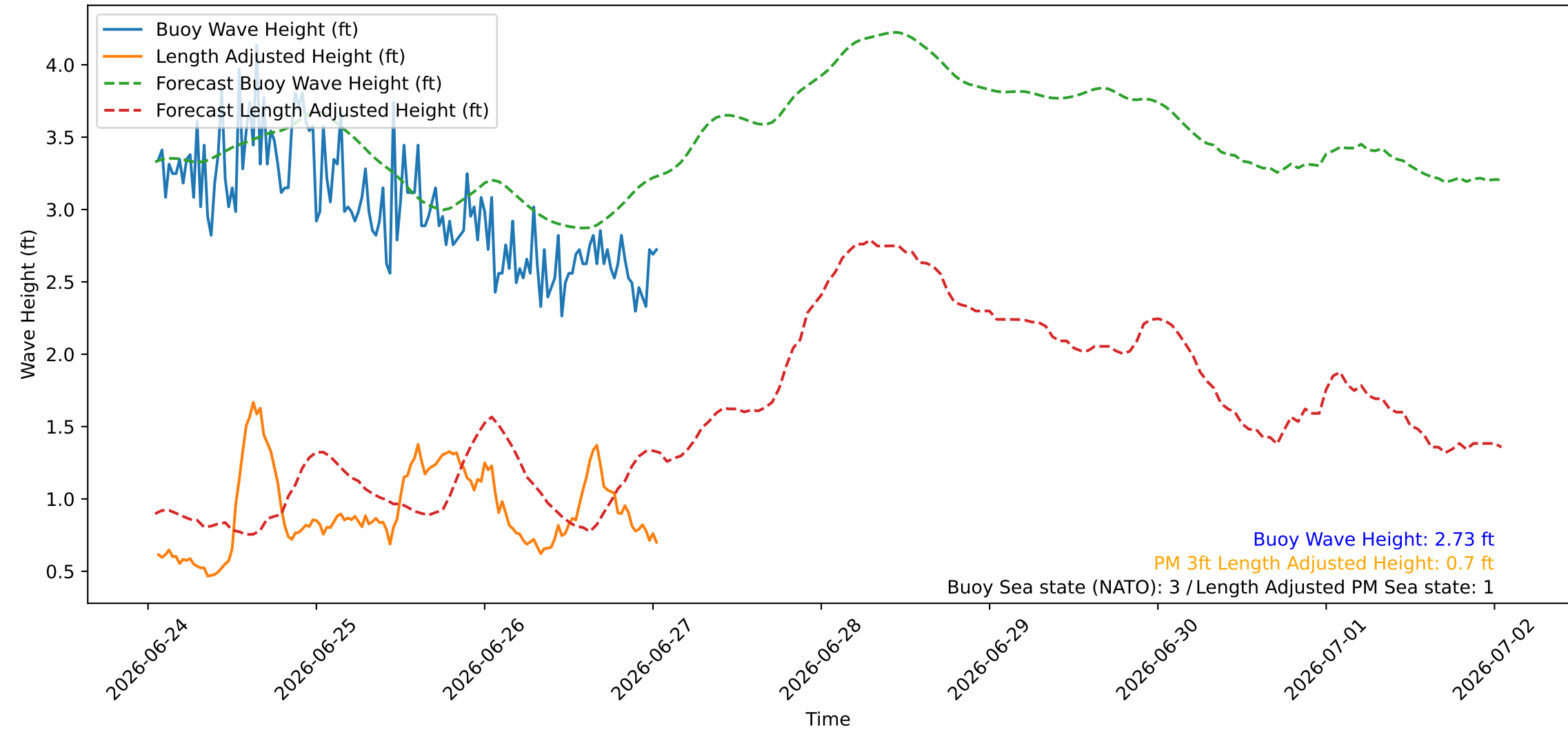
Wave Heights over Time for Red Beach at 2026-06-27 01:10:45
