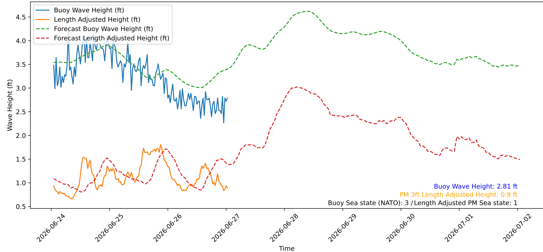
Wave Heights over Time for Green Beach at 2026-06-27 01:11:07
