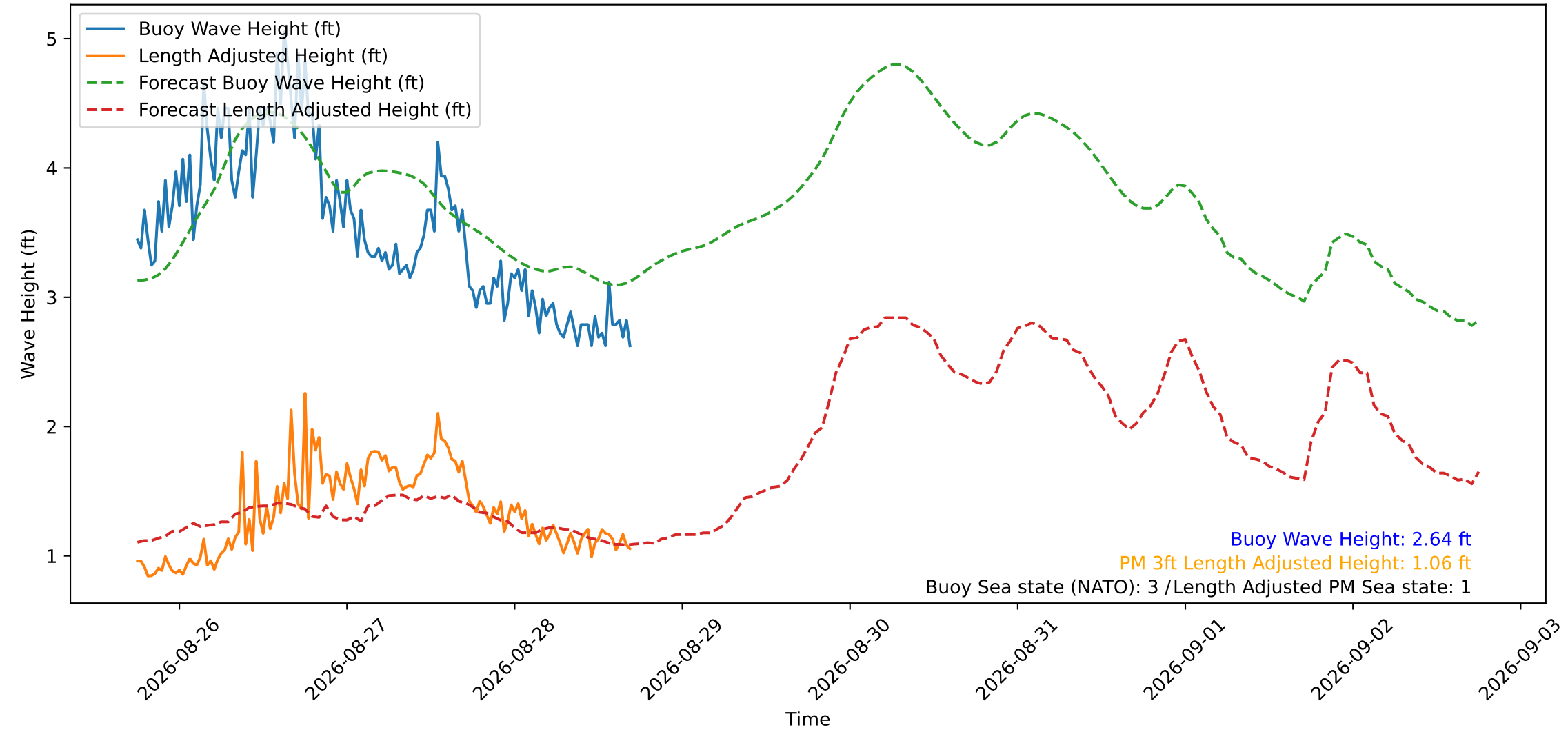
Wave Heights over Time for Red Beach at 2026-08-28 17:30:51
