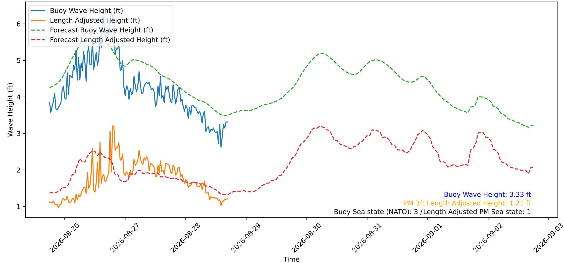
Wave Heights over Time for Green Beach at 2026-08-28 17:31:13
