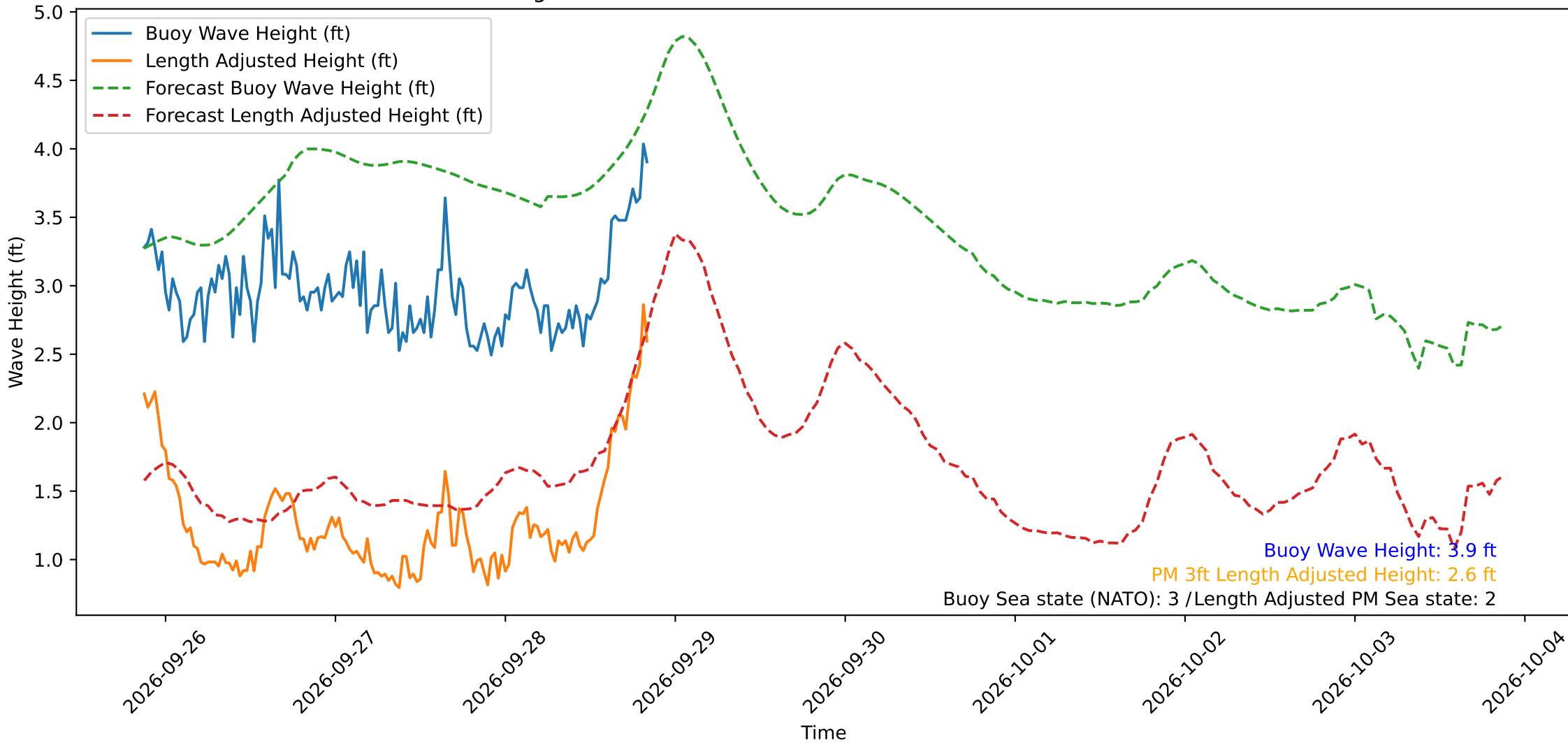
Wave Heights over Time for Oceanside Harbor at 2026-09-28 20:50:29
