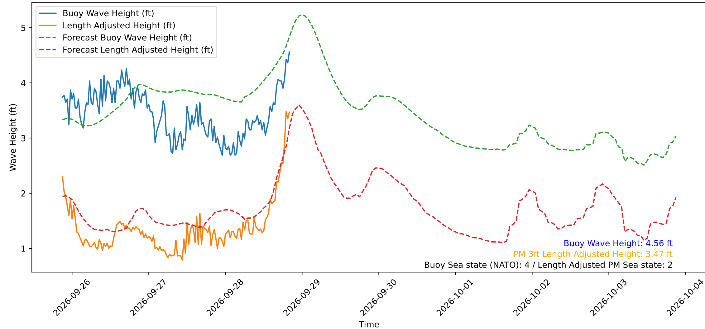
Wave Heights over Time for Green Beach at 2026-09-28 20:51:14
