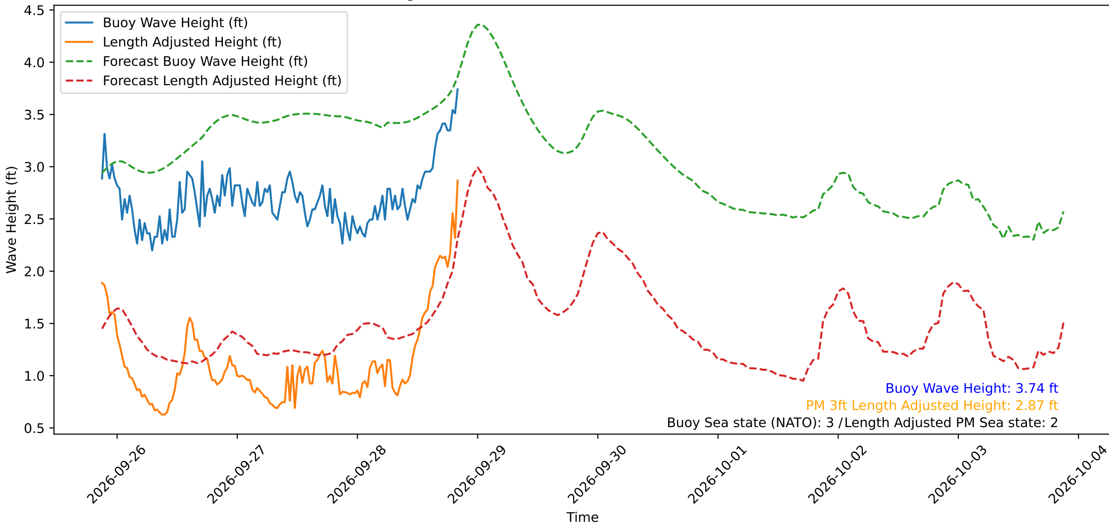
Wave Heights over Time for Red Beach at 2026-09-28 20:50:50
