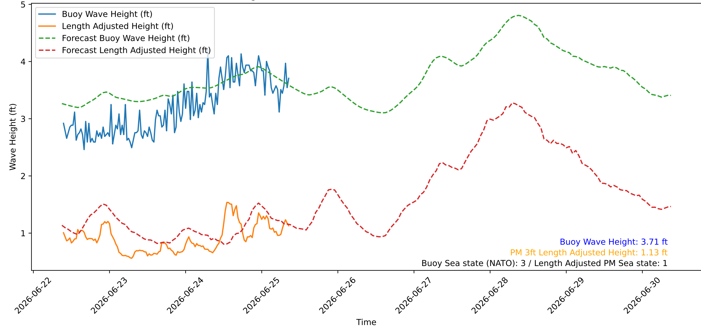
Wave Heights over Time for Green Beach at 2026-06-25 09:21:08
