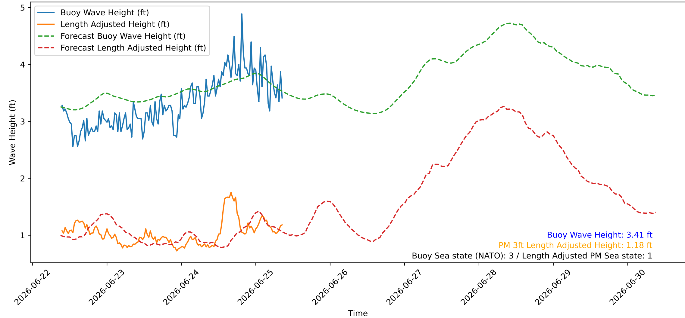
Wave Heights over Time for Oceanside Harbor at 2026-06-25 09:20:26
