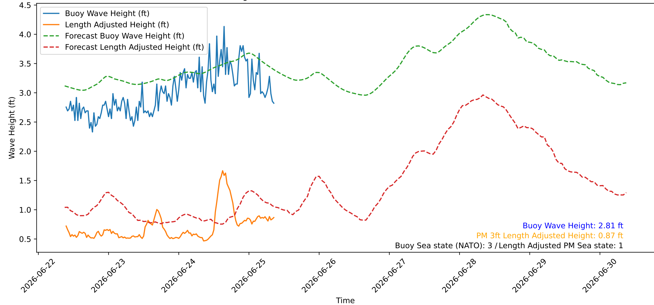
Wave Heights over Time for Red Beach at 2026-06-25 09:20:46
