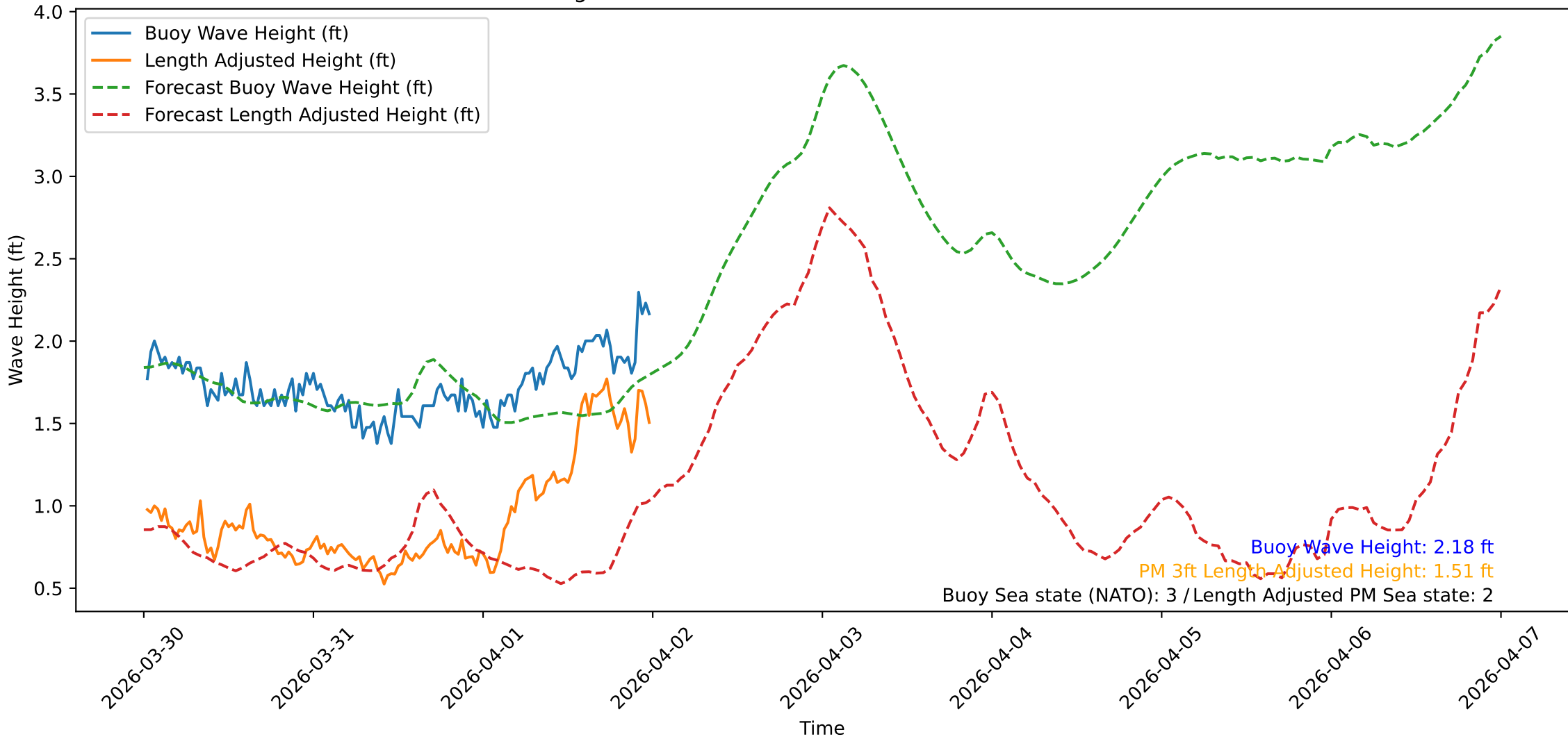
Wave Heights over Time for Red Beach at 2026-04-02 00:20:48
