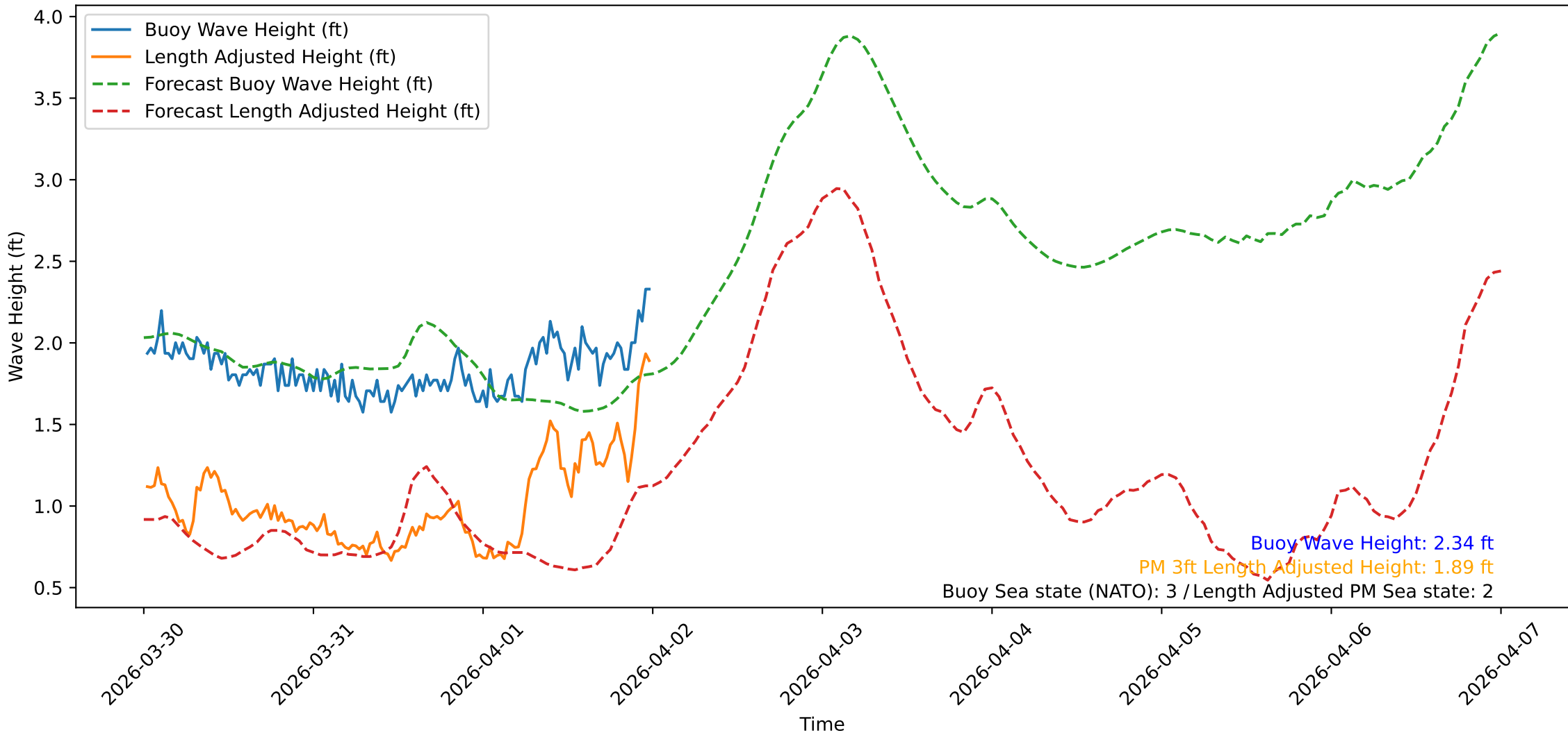
Wave Heights over Time for Oceanside Harbor at 2026-04-02 00:20:31
