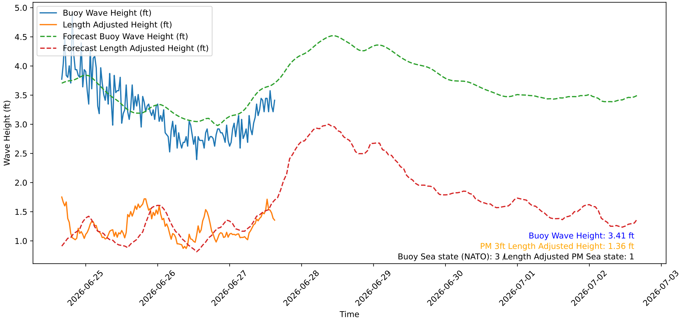
Wave Heights over Time for Oceanside Harbor at 2026-06-27 15:50:26
