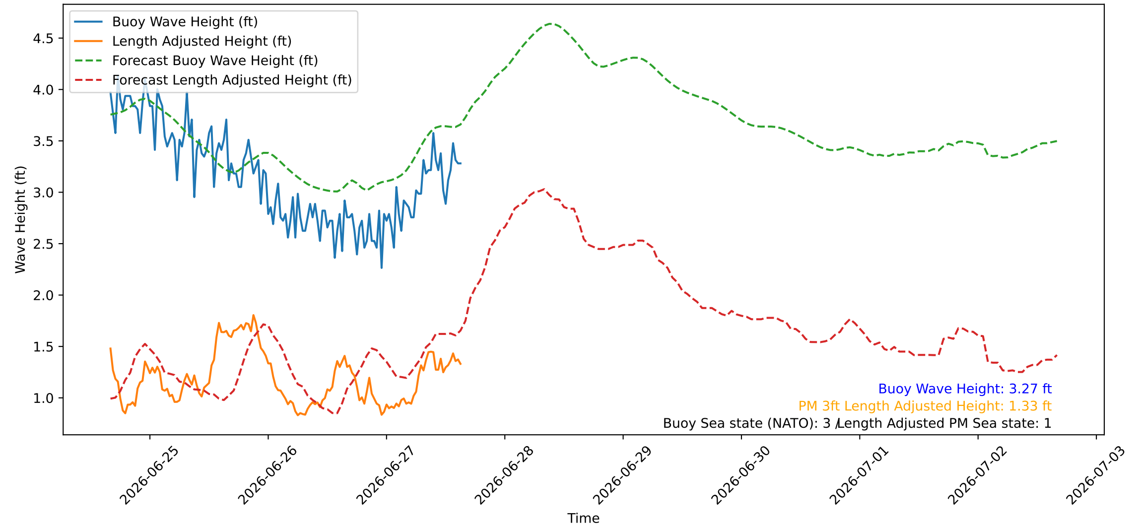
Wave Heights over Time for Green Beach at 2026-06-27 15:51:09
