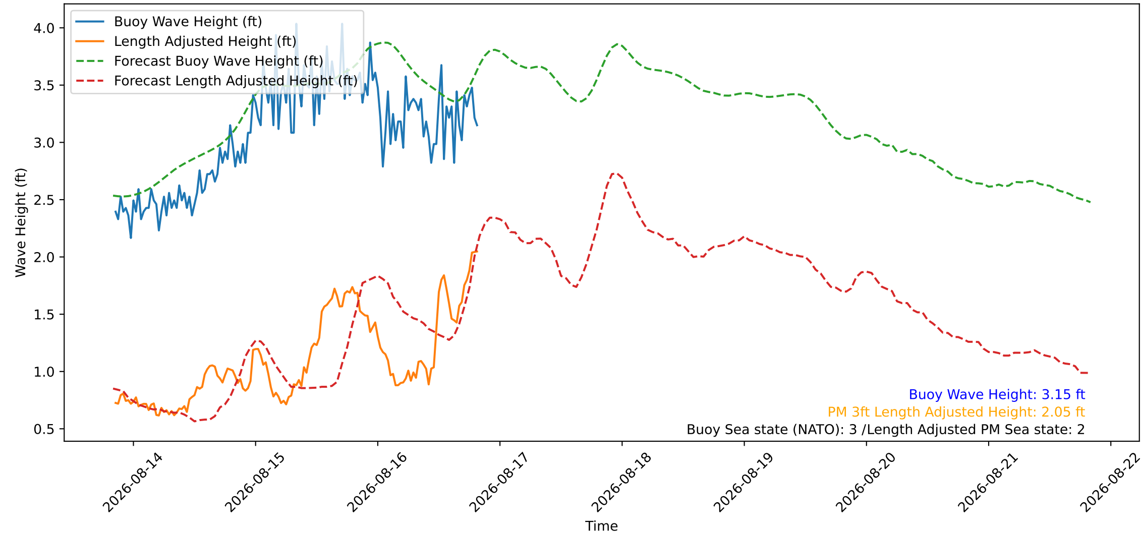
Wave Heights over Time for Red Beach at 2026-08-16 20:20:46
