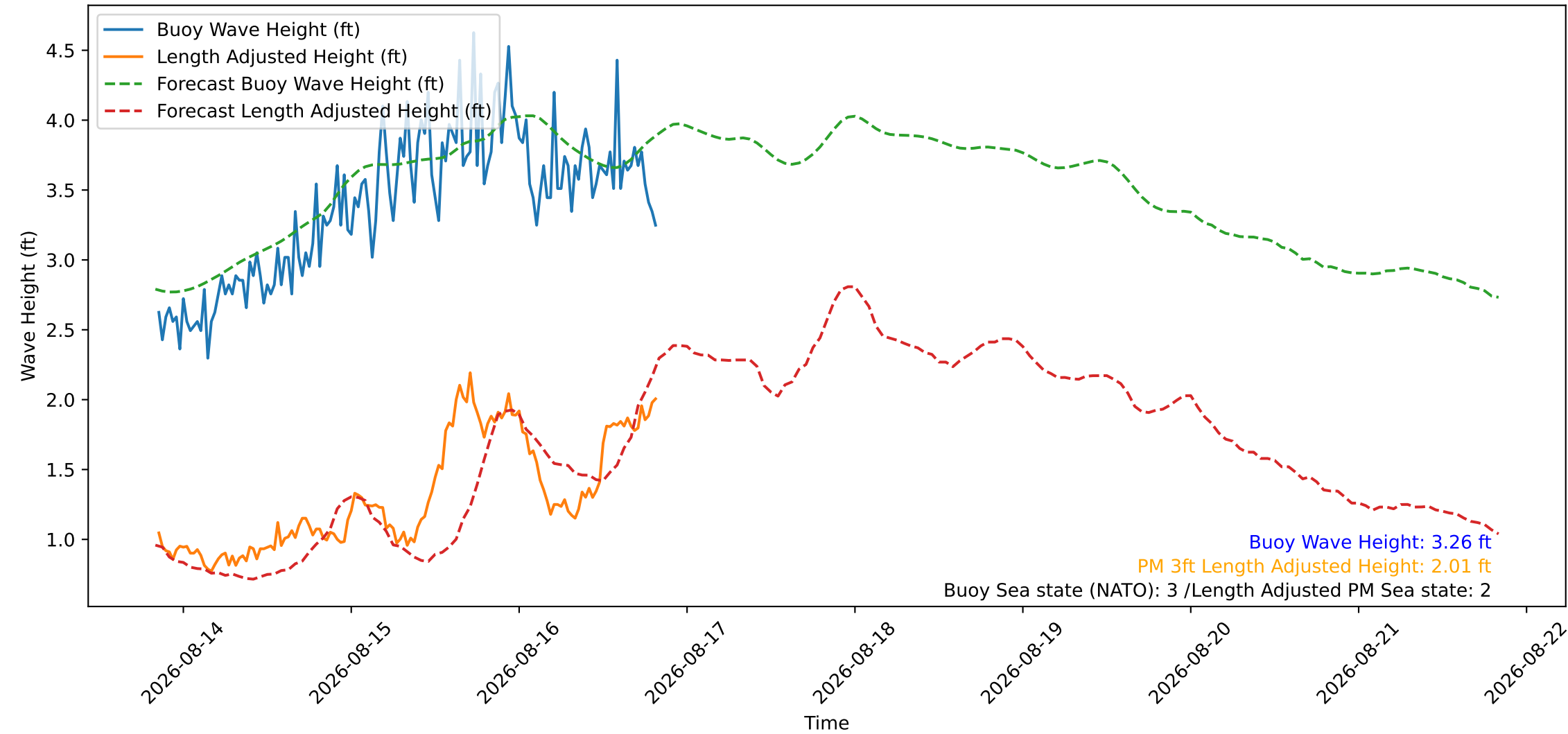
Wave Heights over Time for Oceanside Harbor at 2026-08-16 20:20:26
