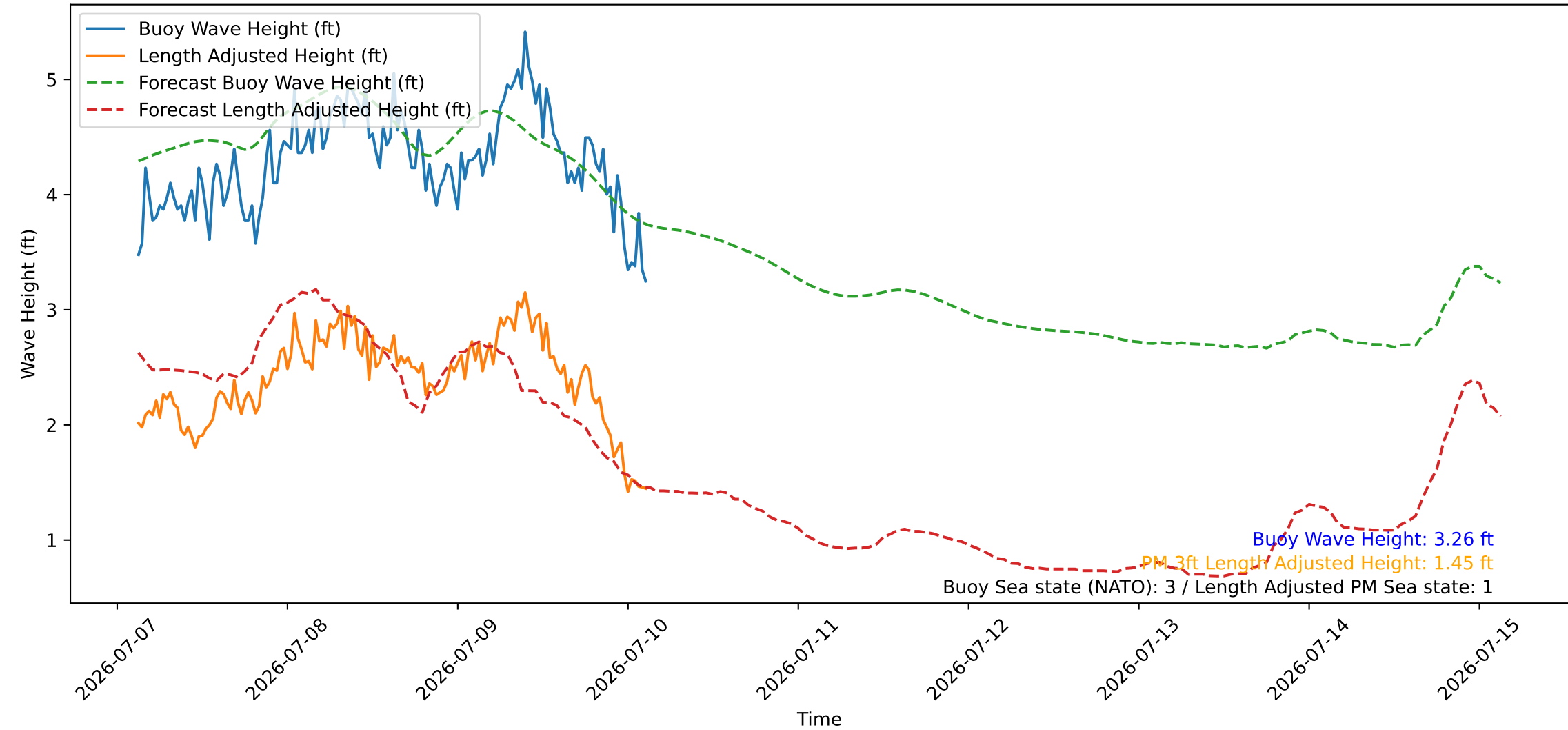
Wave Heights over Time for Oceanside Harbor at 2026-07-10 03:10:26
