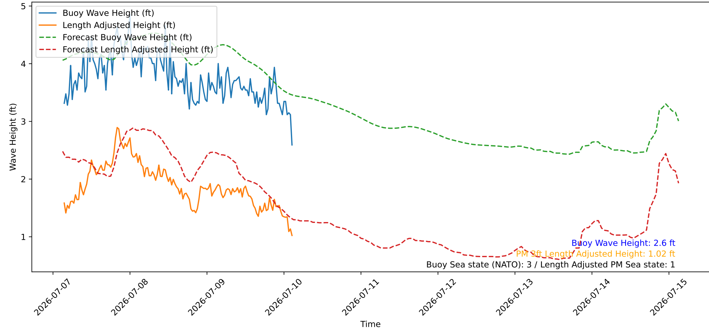
Wave Heights over Time for Red Beach at 2026-07-10 03:10:45
