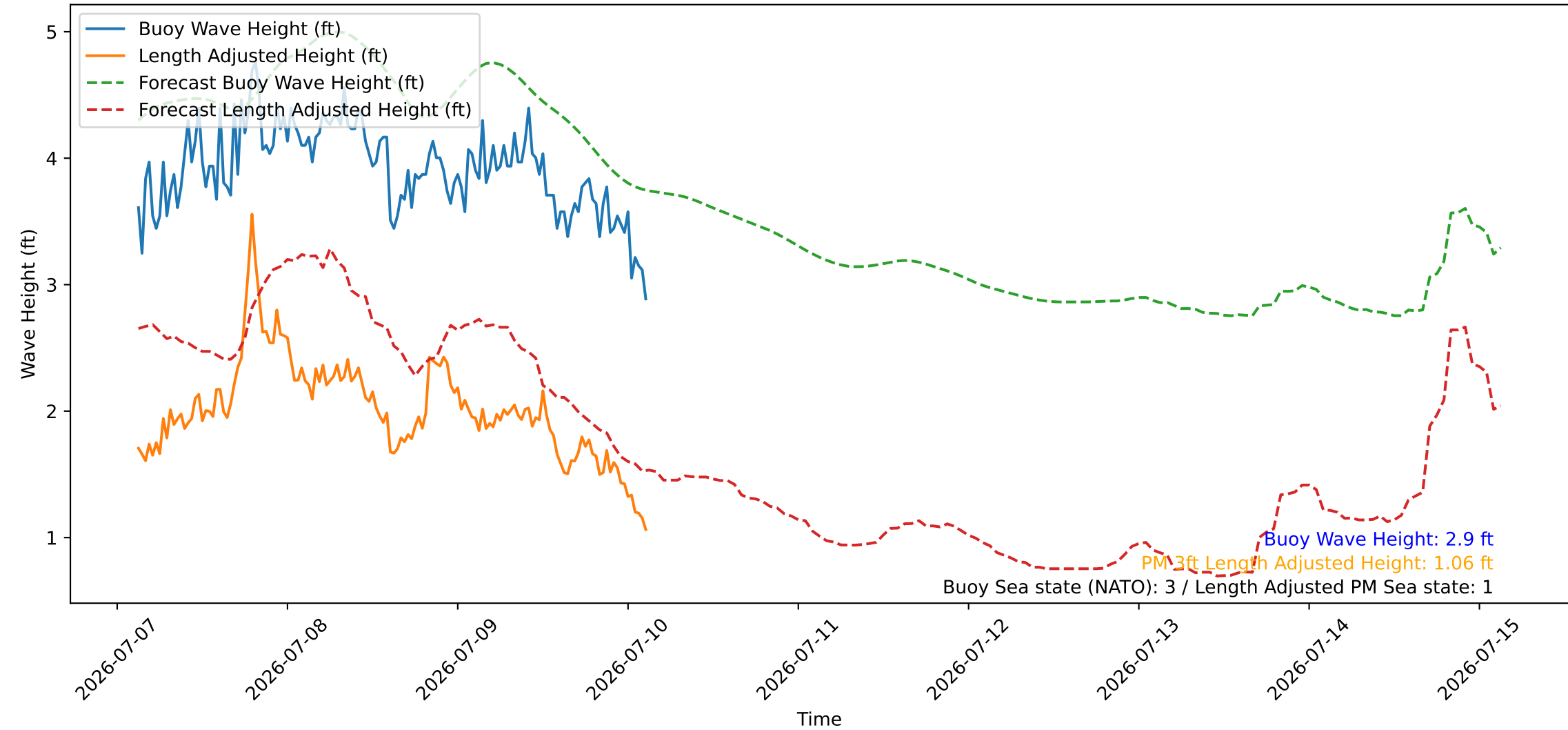
Wave Heights over Time for Green Beach at 2026-07-10 03:11:08
