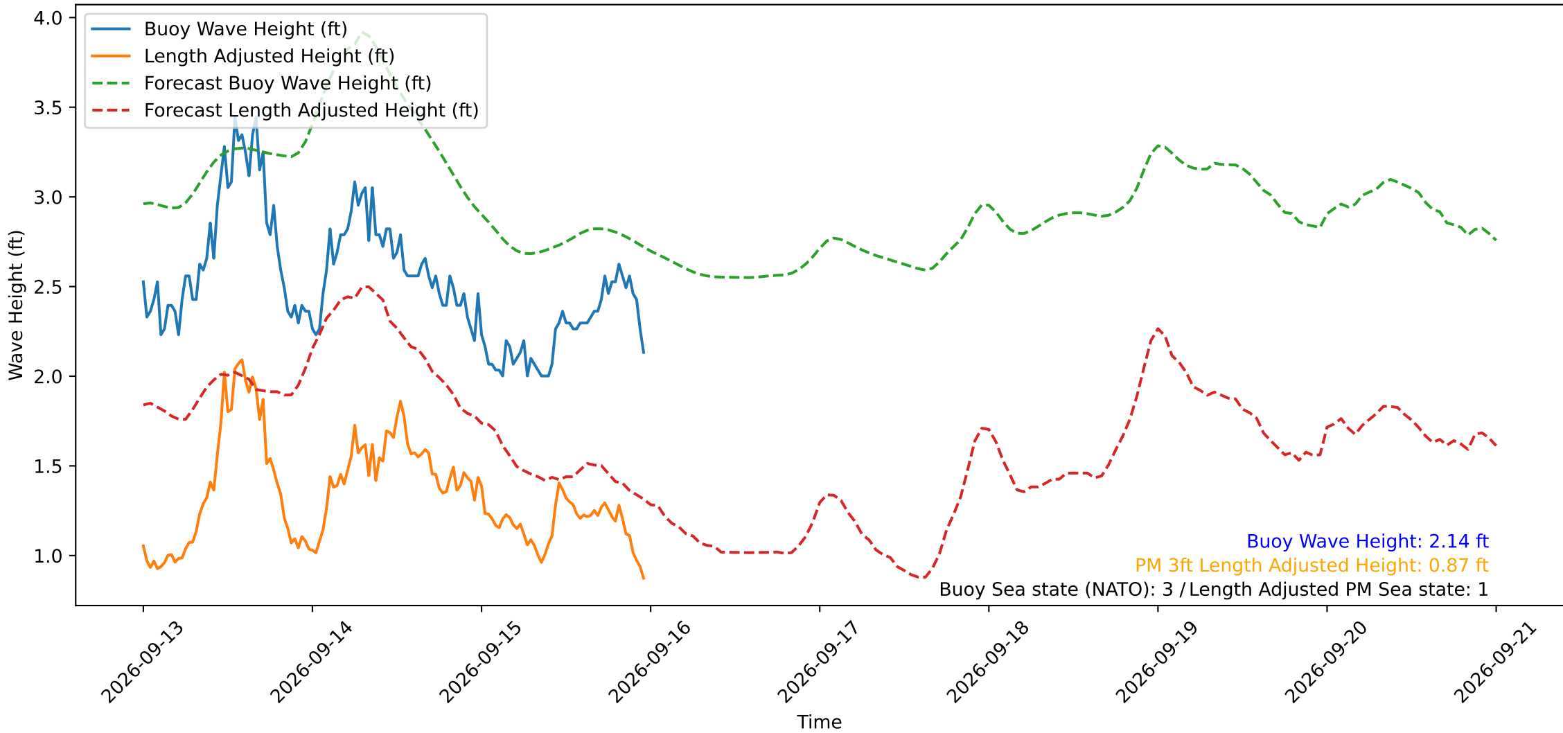
Wave Heights over Time for Red Beach at 2026-09-15 23:40:49
