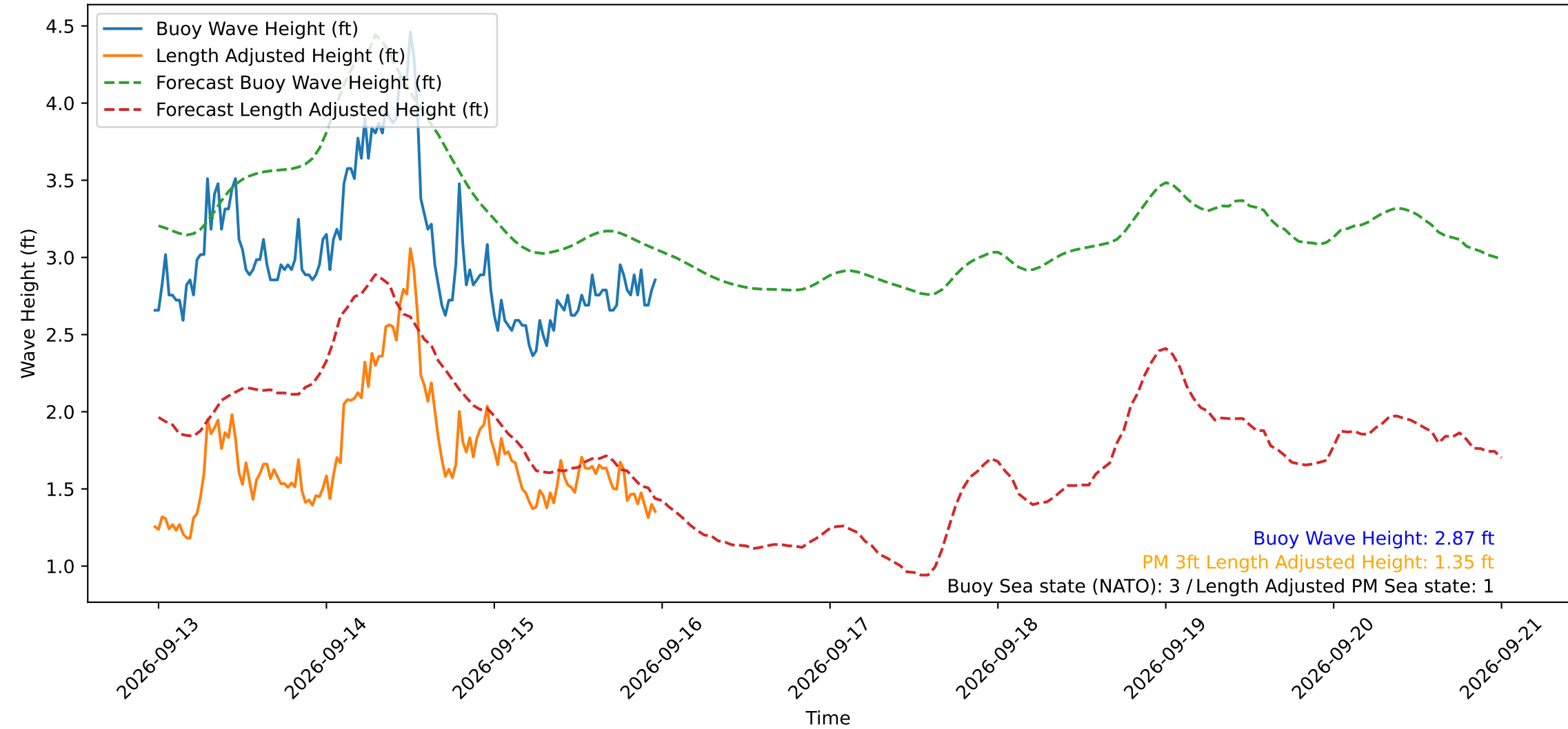
Wave Heights over Time for Oceanside Harbor at 2026-09-15 23:40:30
