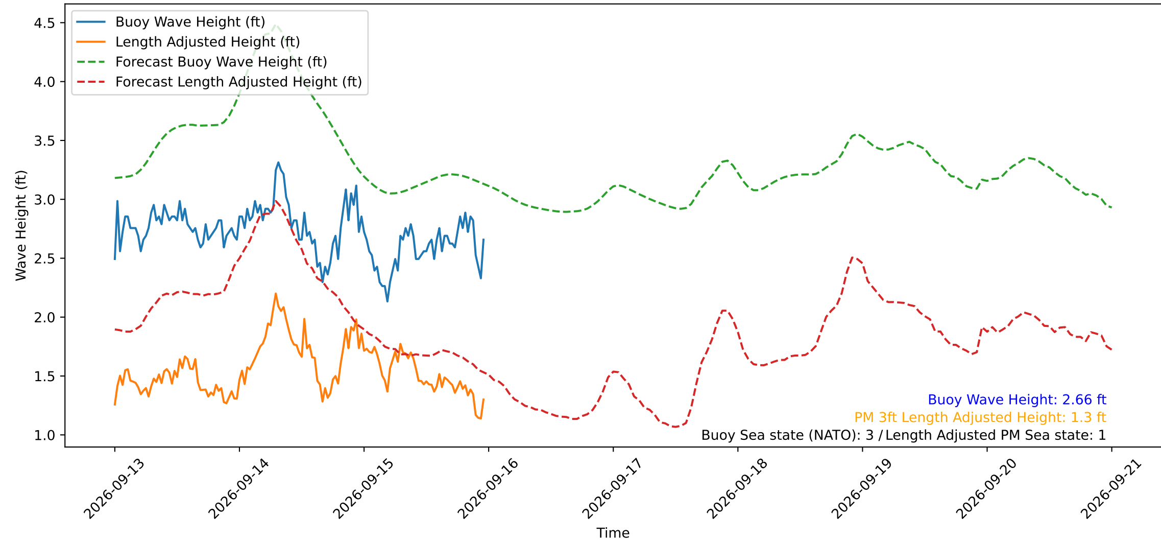
Wave Heights over Time for Green Beach at 2026-09-15 23:41:11
