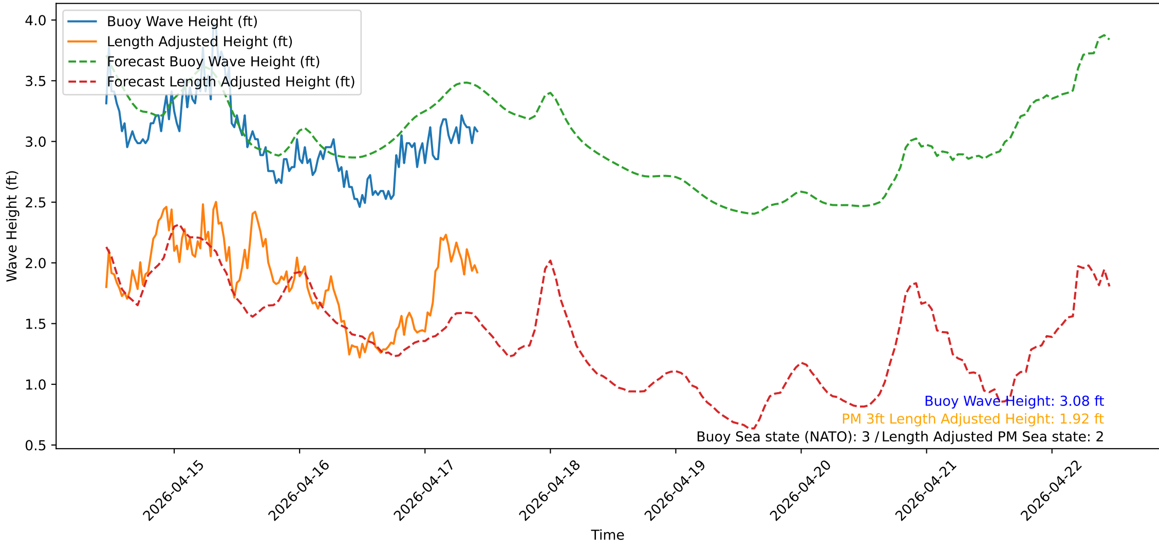
Wave Heights over Time for Green Beach at 2026-04-17 10:51:14
