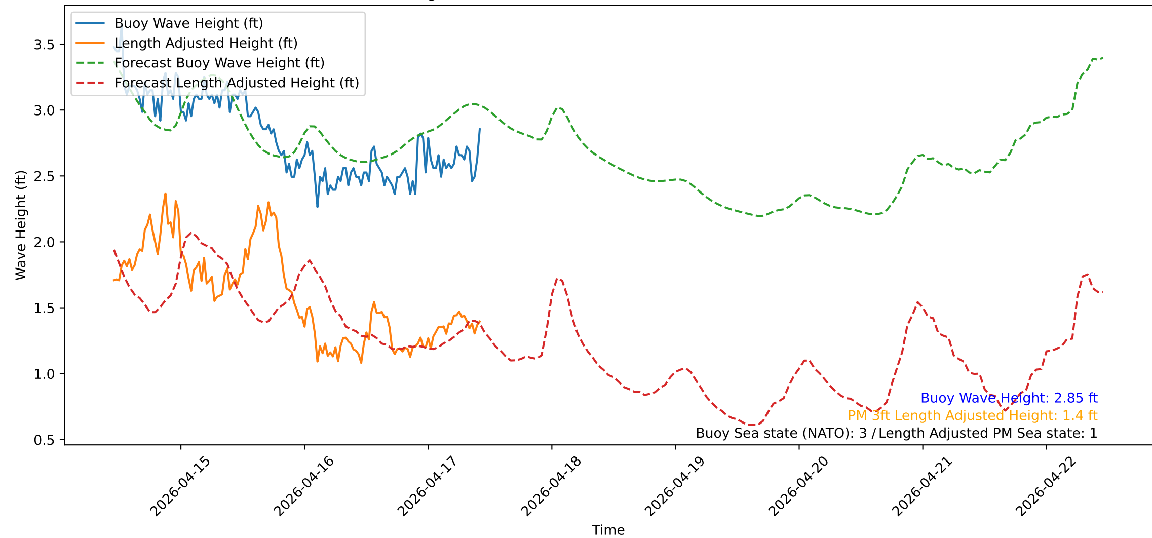
Wave Heights over Time for Red Beach at 2026-04-17 10:50:52
