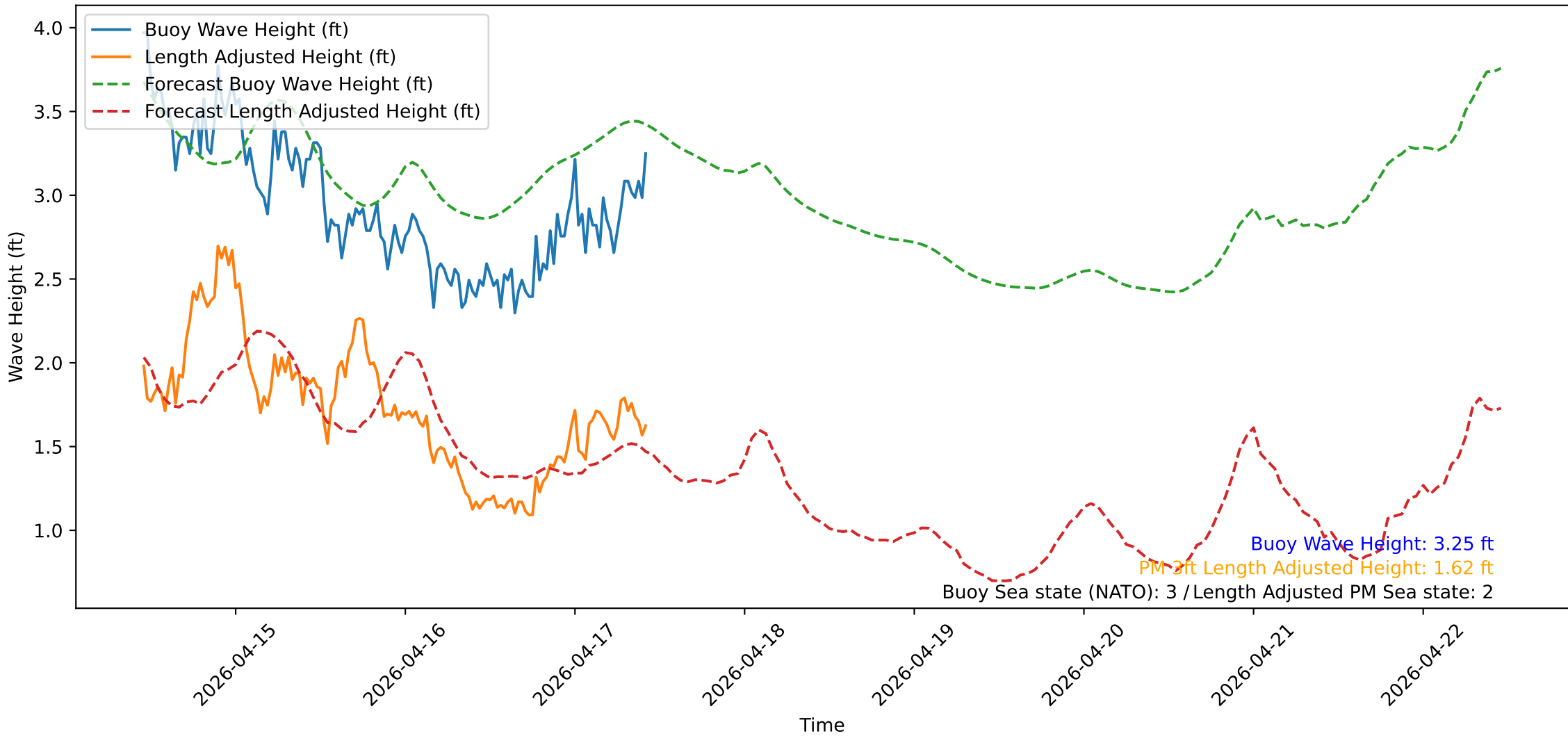
Wave Heights over Time for Oceanside Harbor at 2026-04-17 10:50:31
