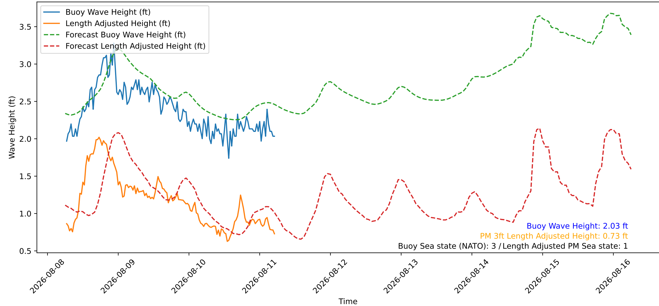
Wave Heights over Time for Red Beach at 2026-08-11 06:10:46
