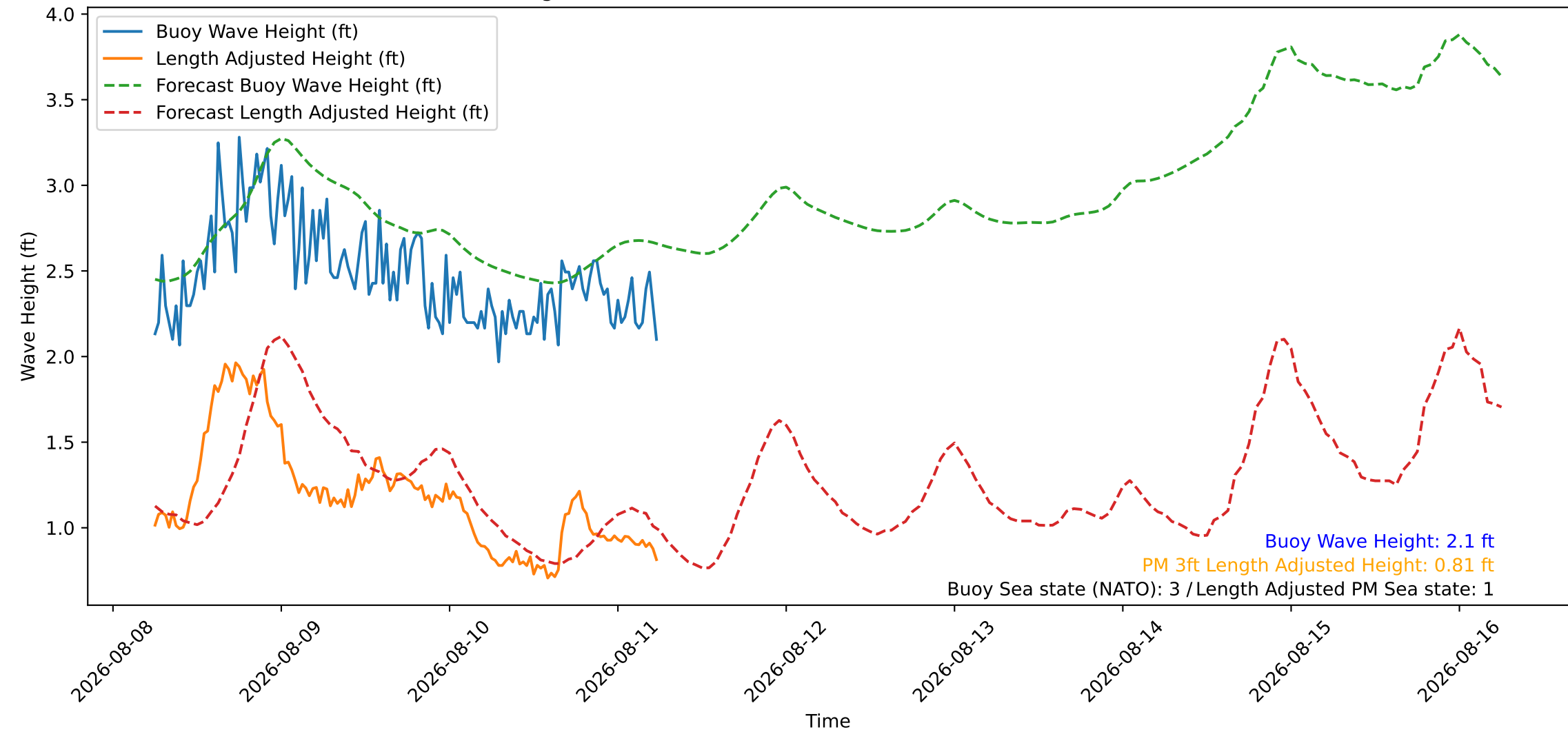
Wave Heights over Time for Oceanside Harbor at 2026-08-11 06:10:27
