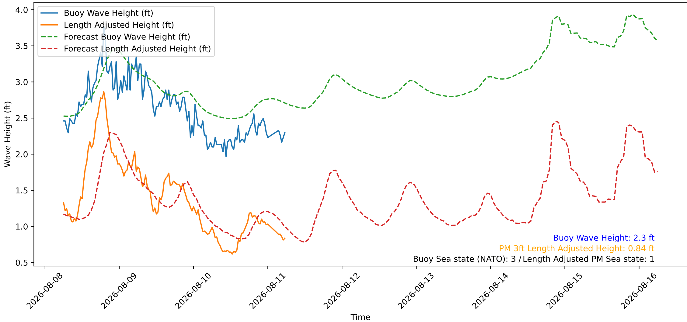
Wave Heights over Time for Green Beach at 2026-08-11 06:11:09
