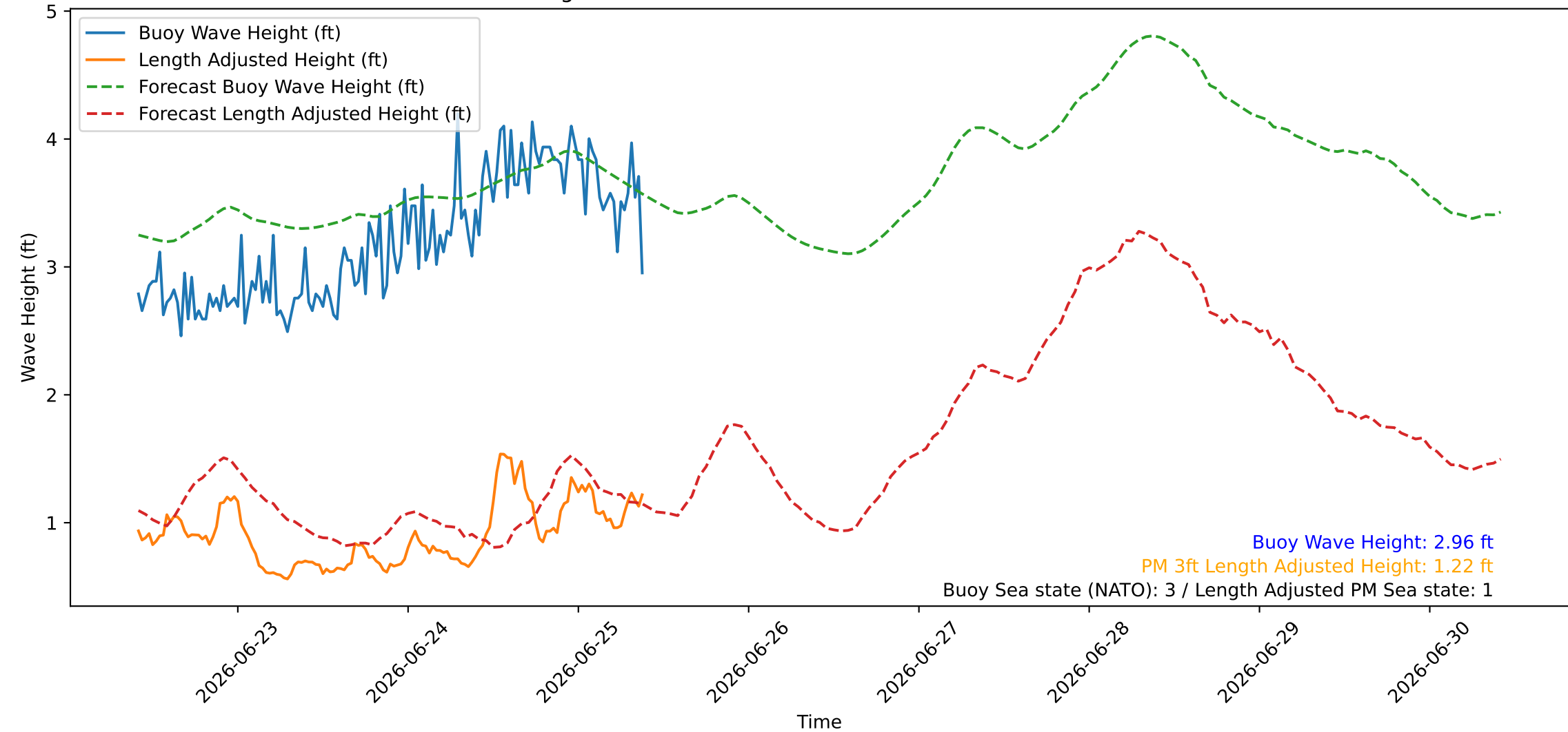
Wave Heights over Time for Green Beach at 2026-06-25 09:51:09
