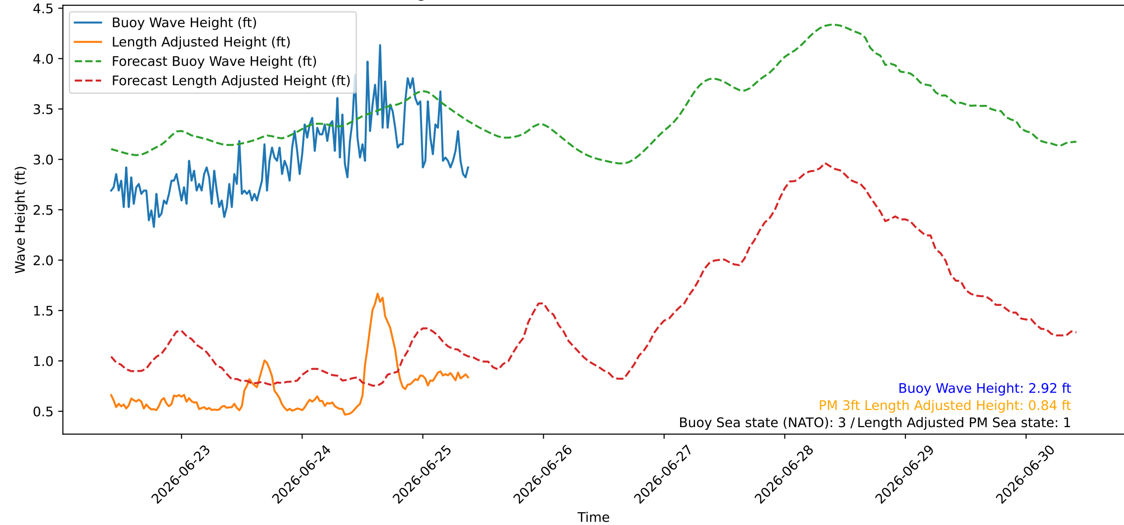
Wave Heights over Time for Red Beach at 2026-06-25 09:50:47
