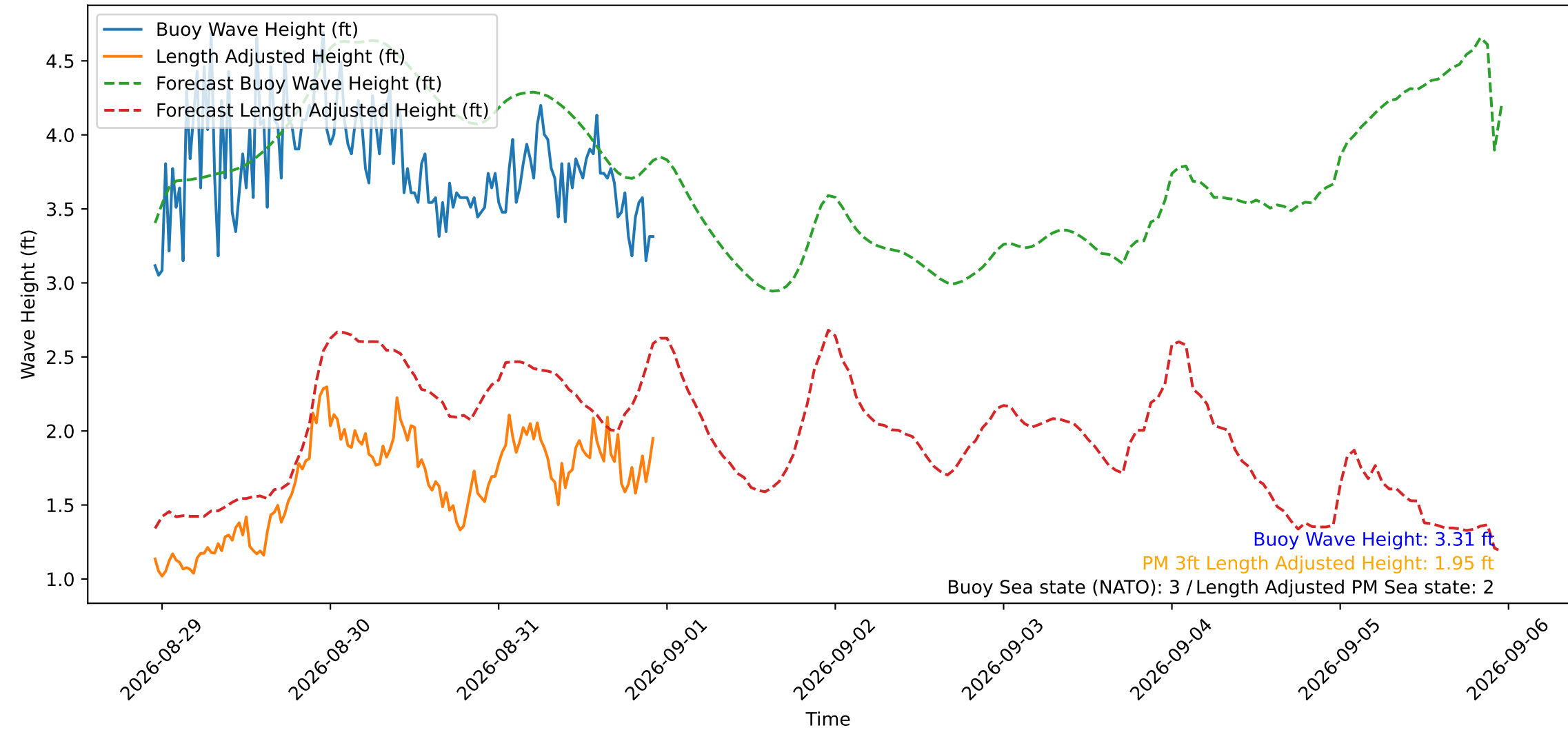
Wave Heights over Time for Red Beach at 2026-08-31 22:40:49
