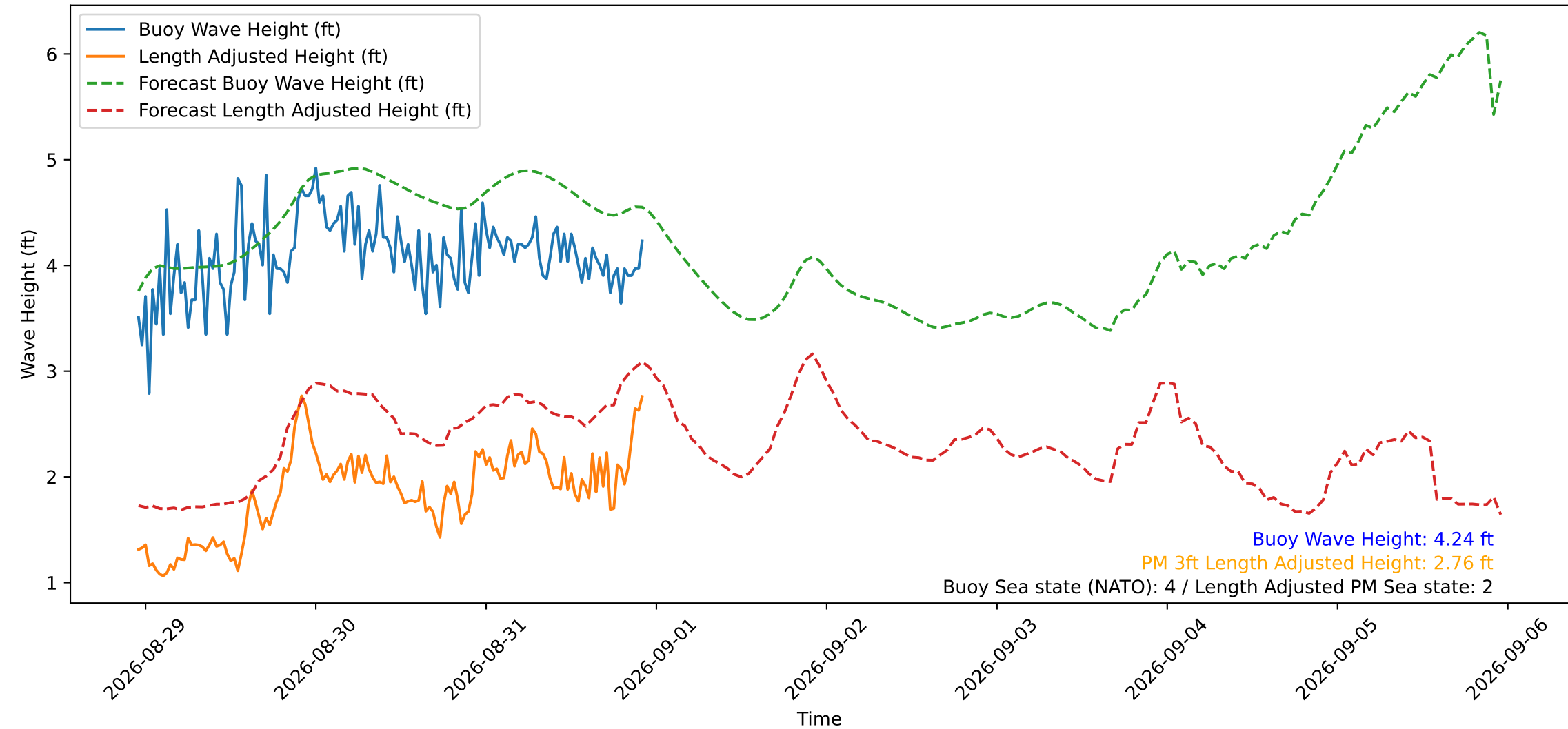
Wave Heights over Time for Green Beach at 2026-08-31 22:41:12
