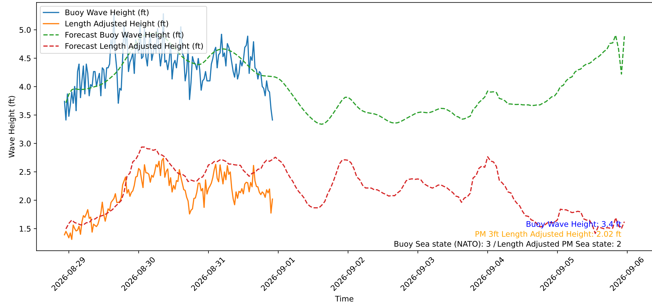
Wave Heights over Time for Oceanside Harbor at 2026-08-31 22:40:29
