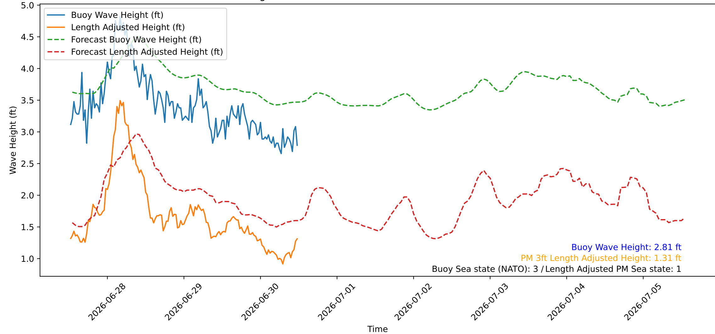
Wave Heights over Time for Green Beach at 2026-06-30 12:31:07
