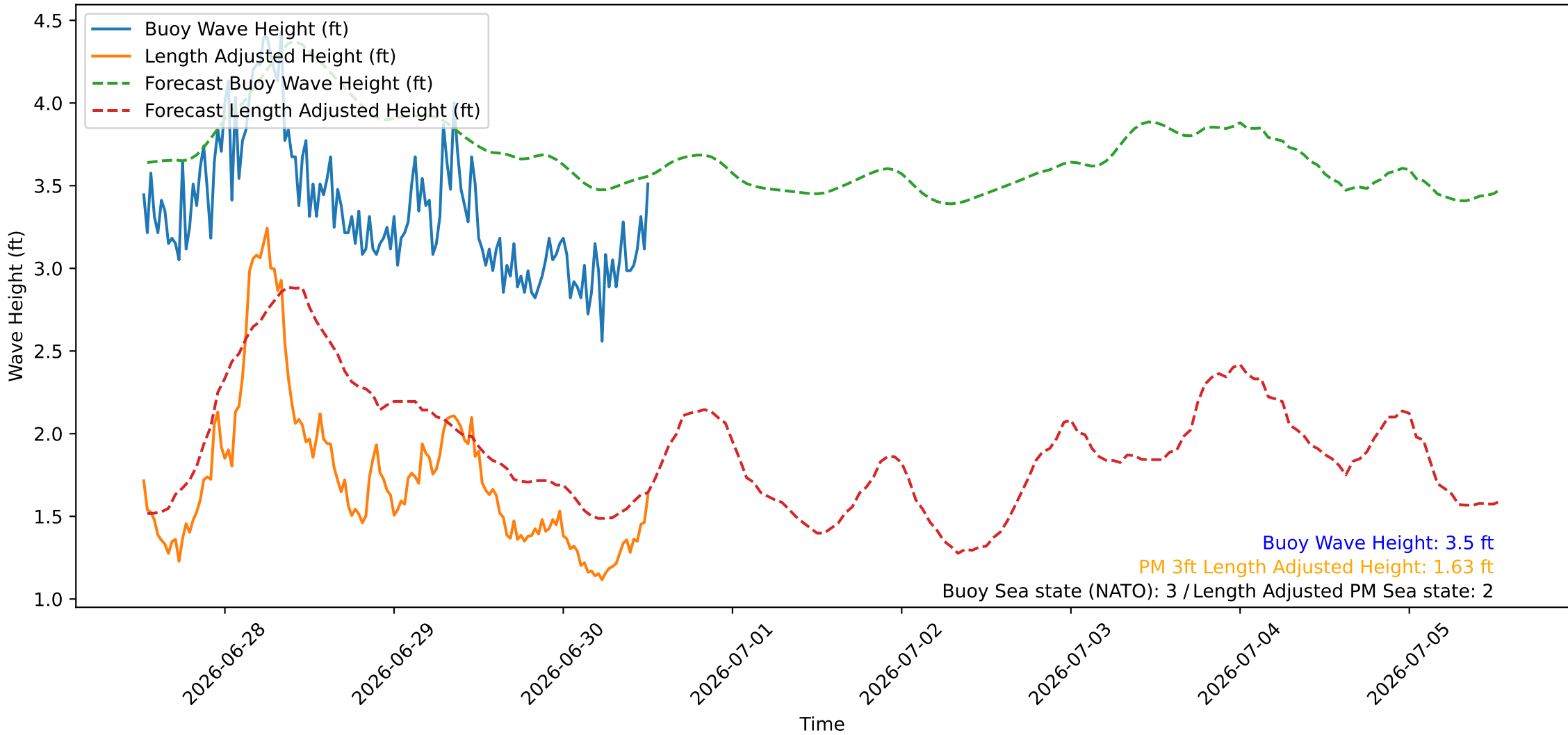
Wave Heights over Time for Oceanside Harbor at 2026-06-30 12:30:26
