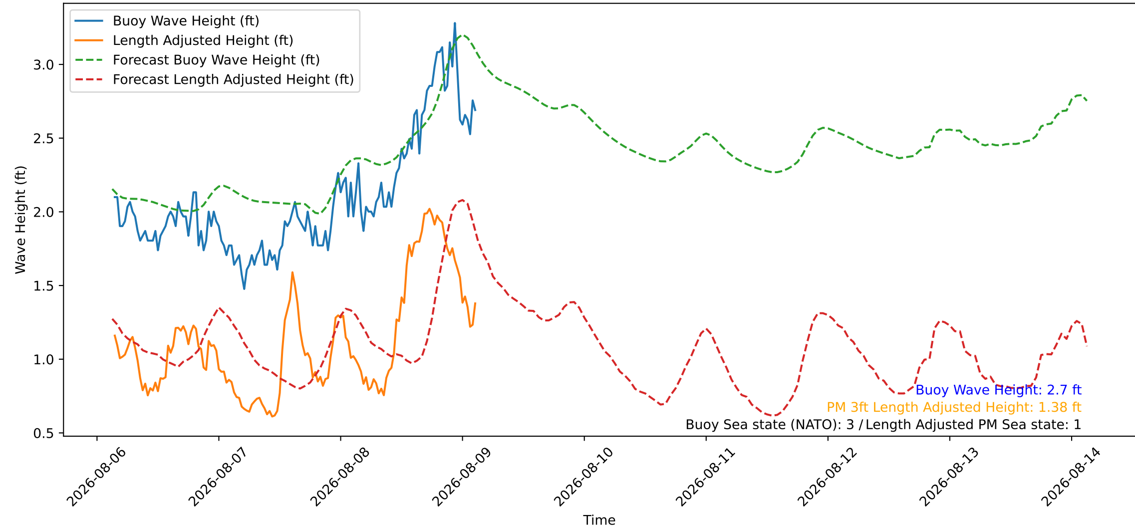
Wave Heights over Time for Red Beach at 2026-08-09 03:20:47
