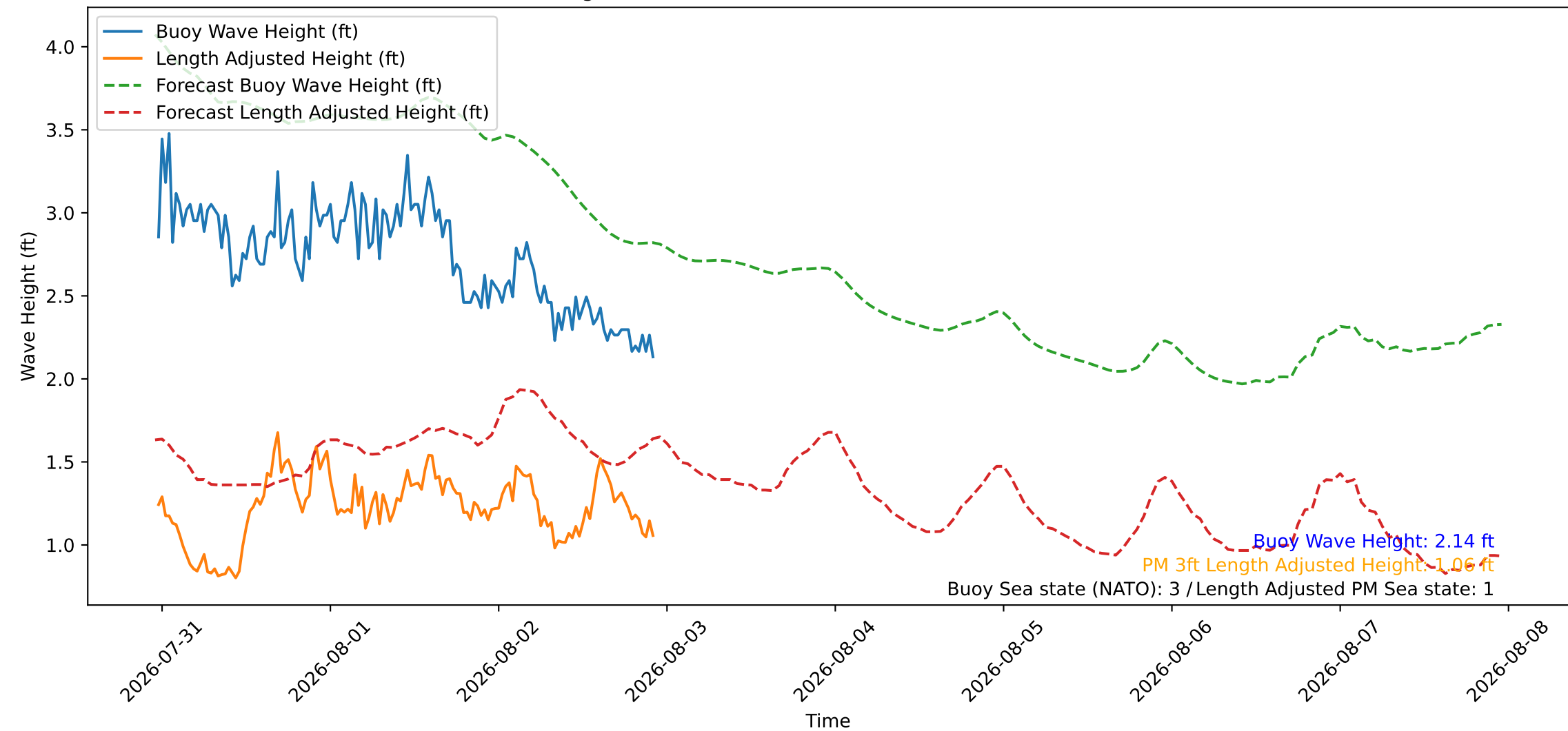
Wave Heights over Time for Red Beach at 2026-08-02 23:00:46
