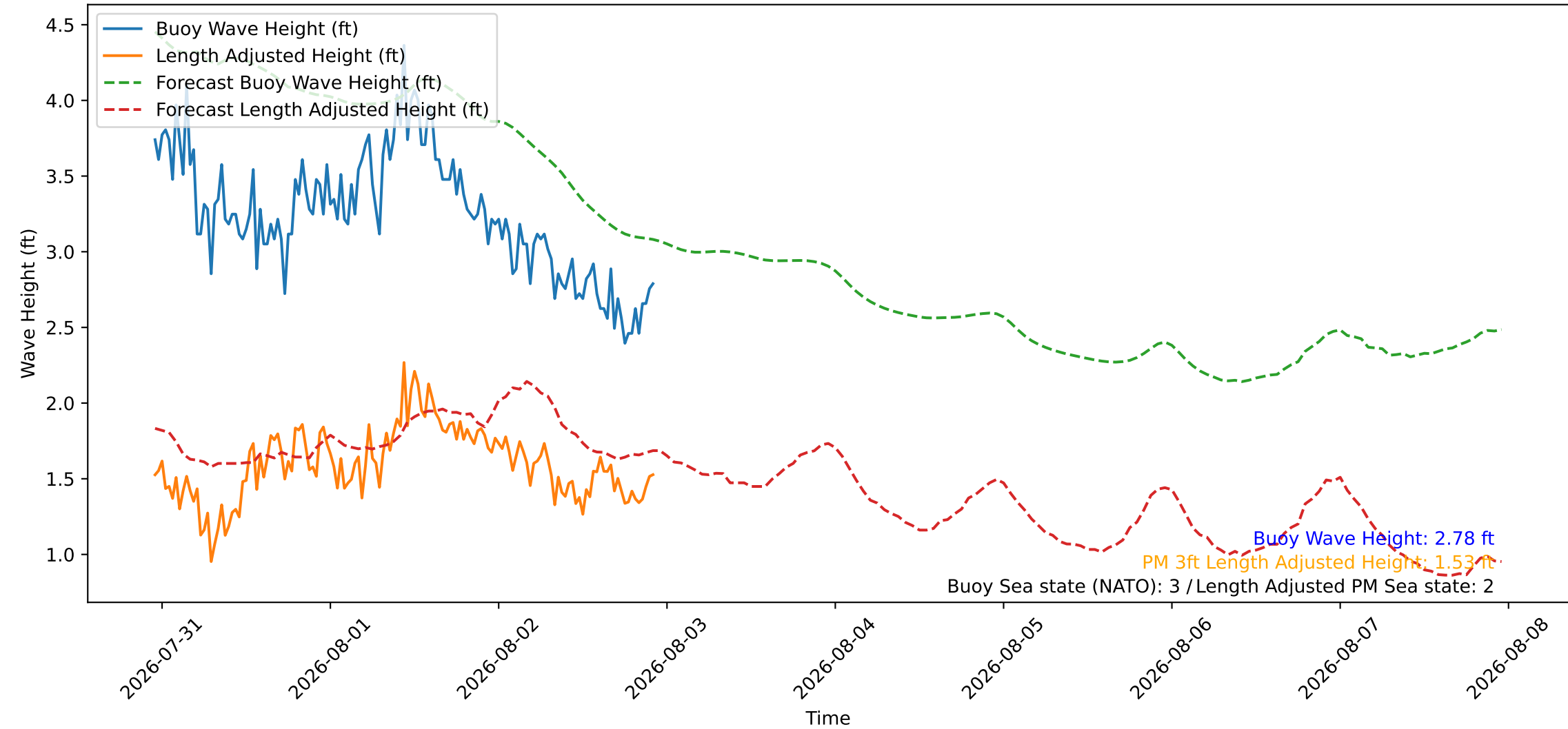
Wave Heights over Time for Oceanside Harbor at 2026-08-02 23:00:27
