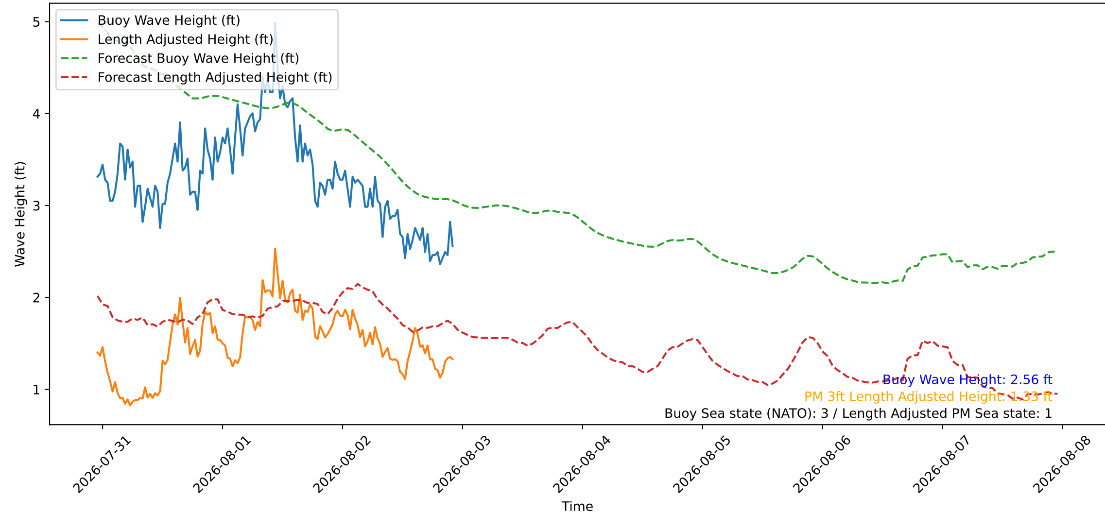
Wave Heights over Time for Green Beach at 2026-08-02 23:01:08
