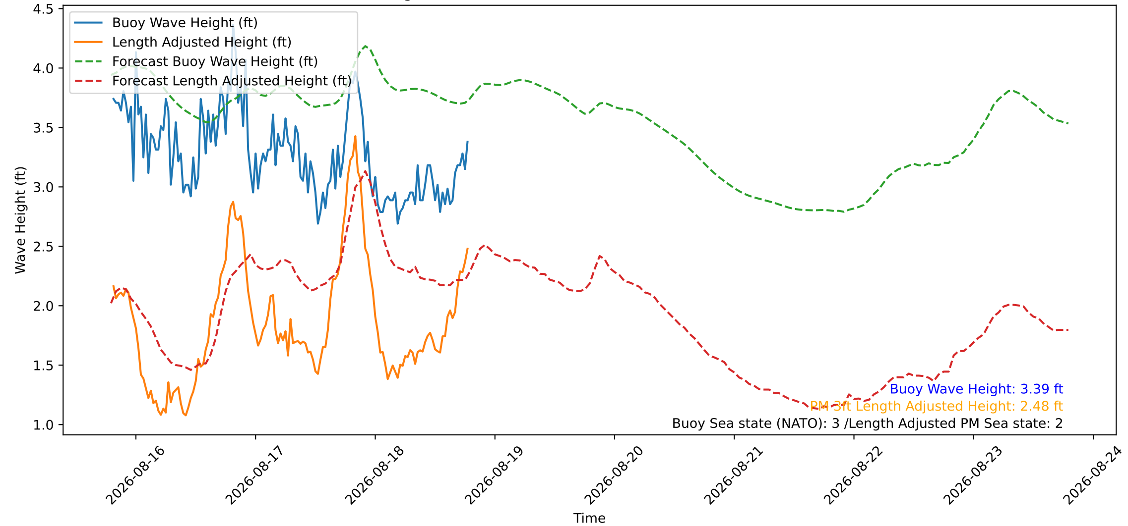
Wave Heights over Time for Green Beach at 2026-08-18 19:21:12
