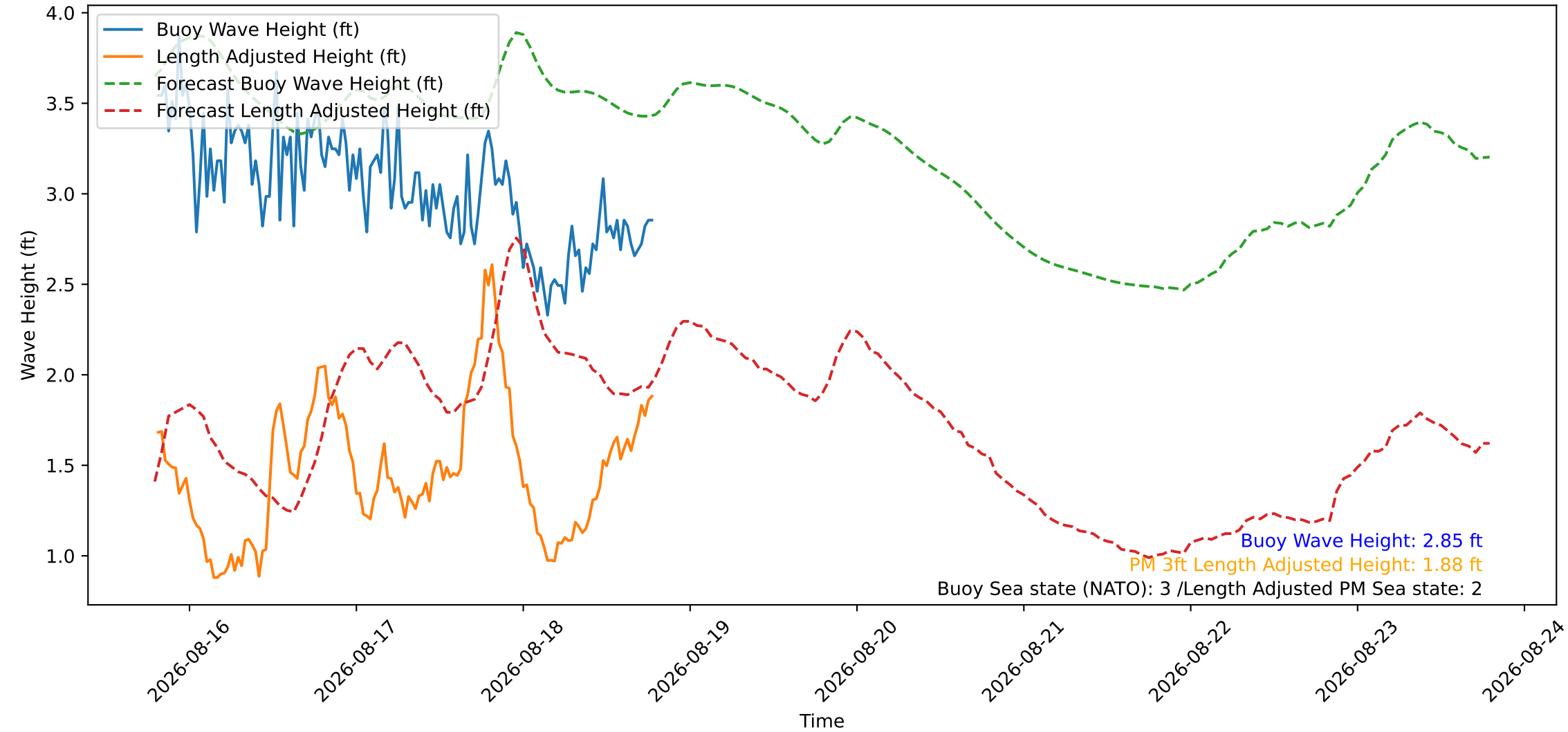
Wave Heights over Time for Red Beach at 2026-08-18 19:20:48
