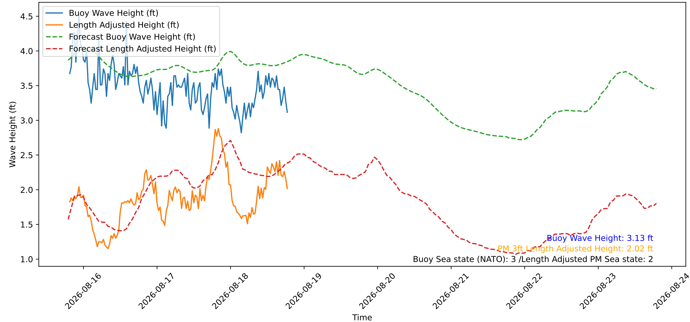
Wave Heights over Time for Oceanside Harbor at 2026-08-18 19:20:27
