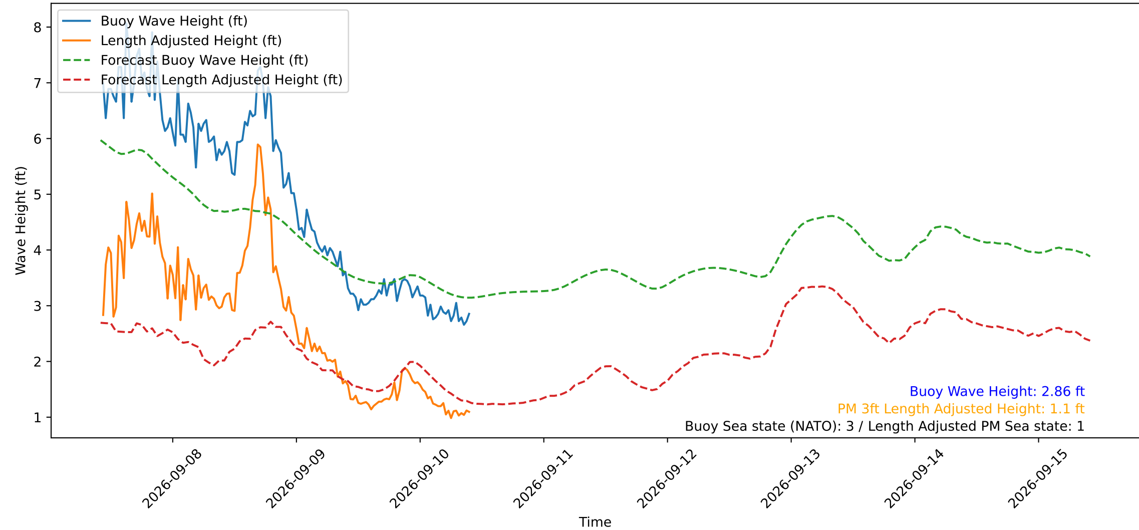
Wave Heights over Time for Green Beach at 2026-09-10 10:11:12
