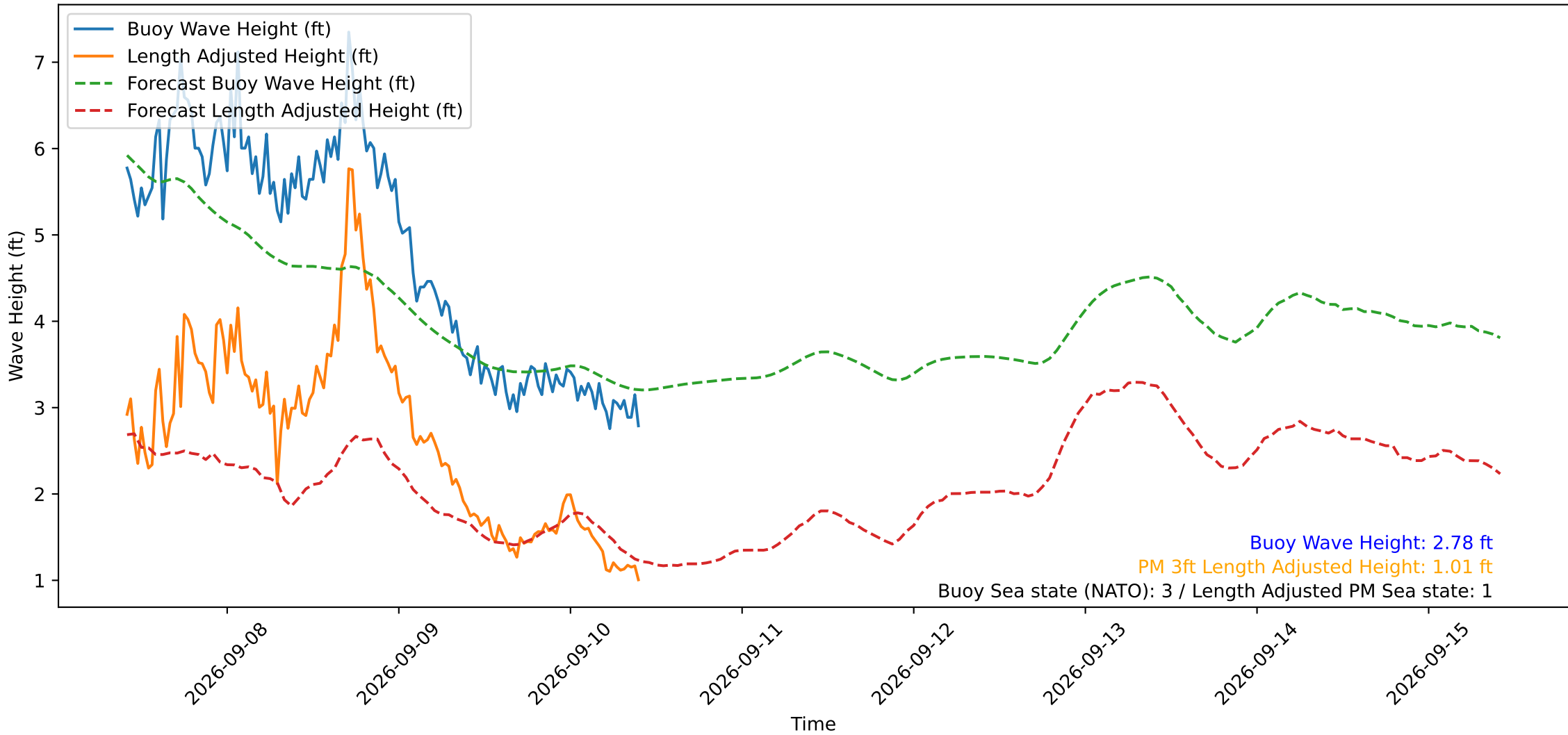
Wave Heights over Time for Oceanside Harbor at 2026-09-10 10:10:29
