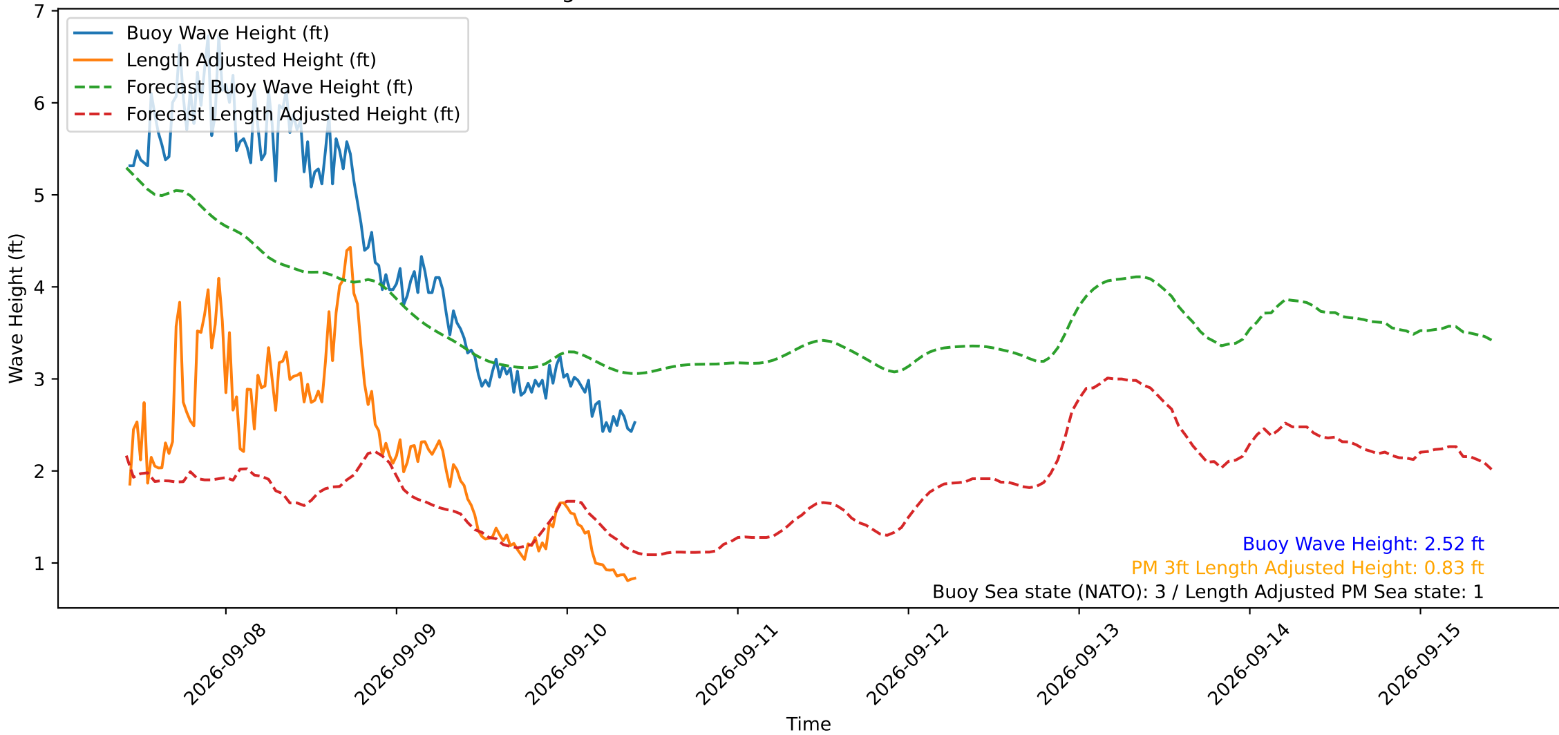
Wave Heights over Time for Red Beach at 2026-09-10 10:10:49
