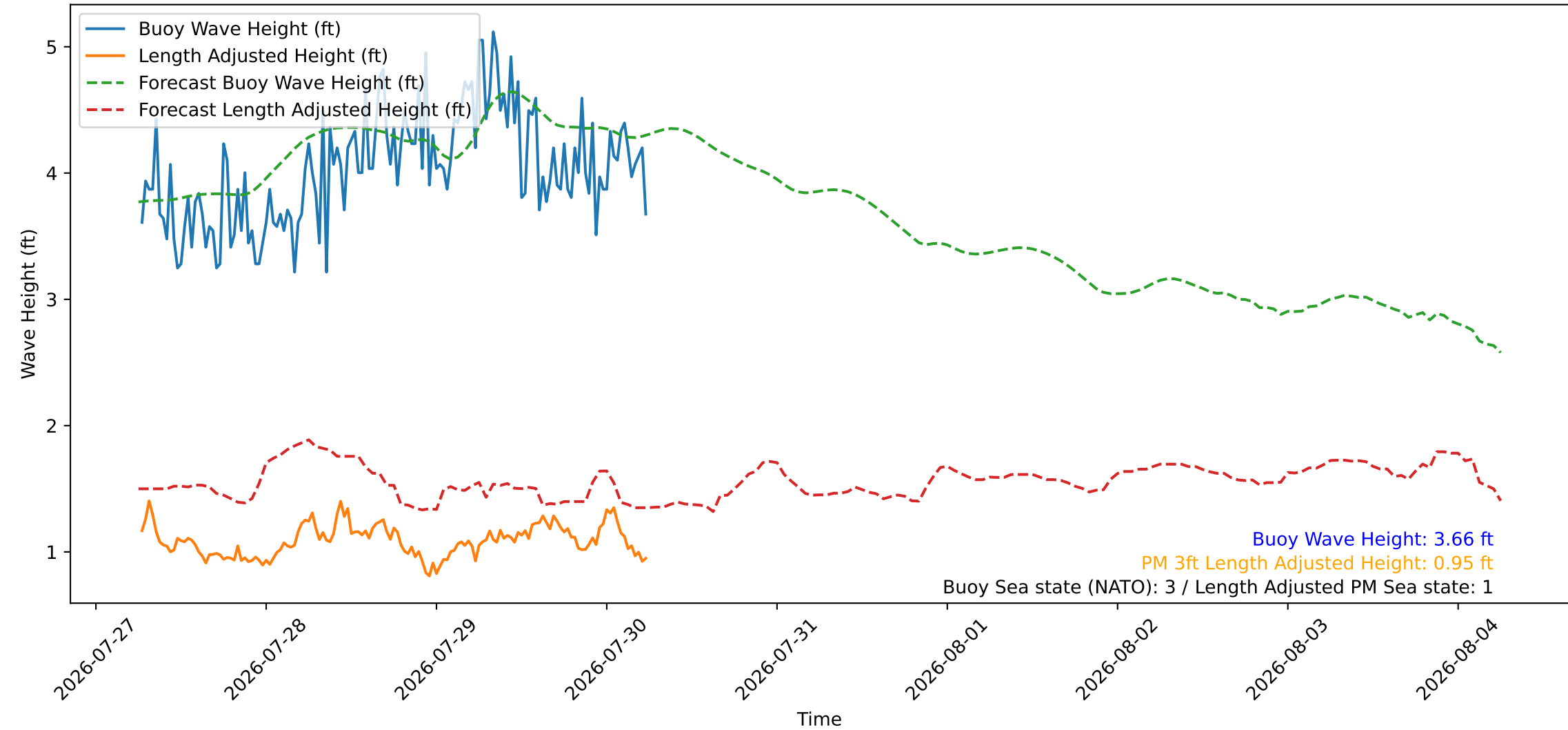
Wave Heights over Time for Red Beach at 2026-07-30 06:20:47
