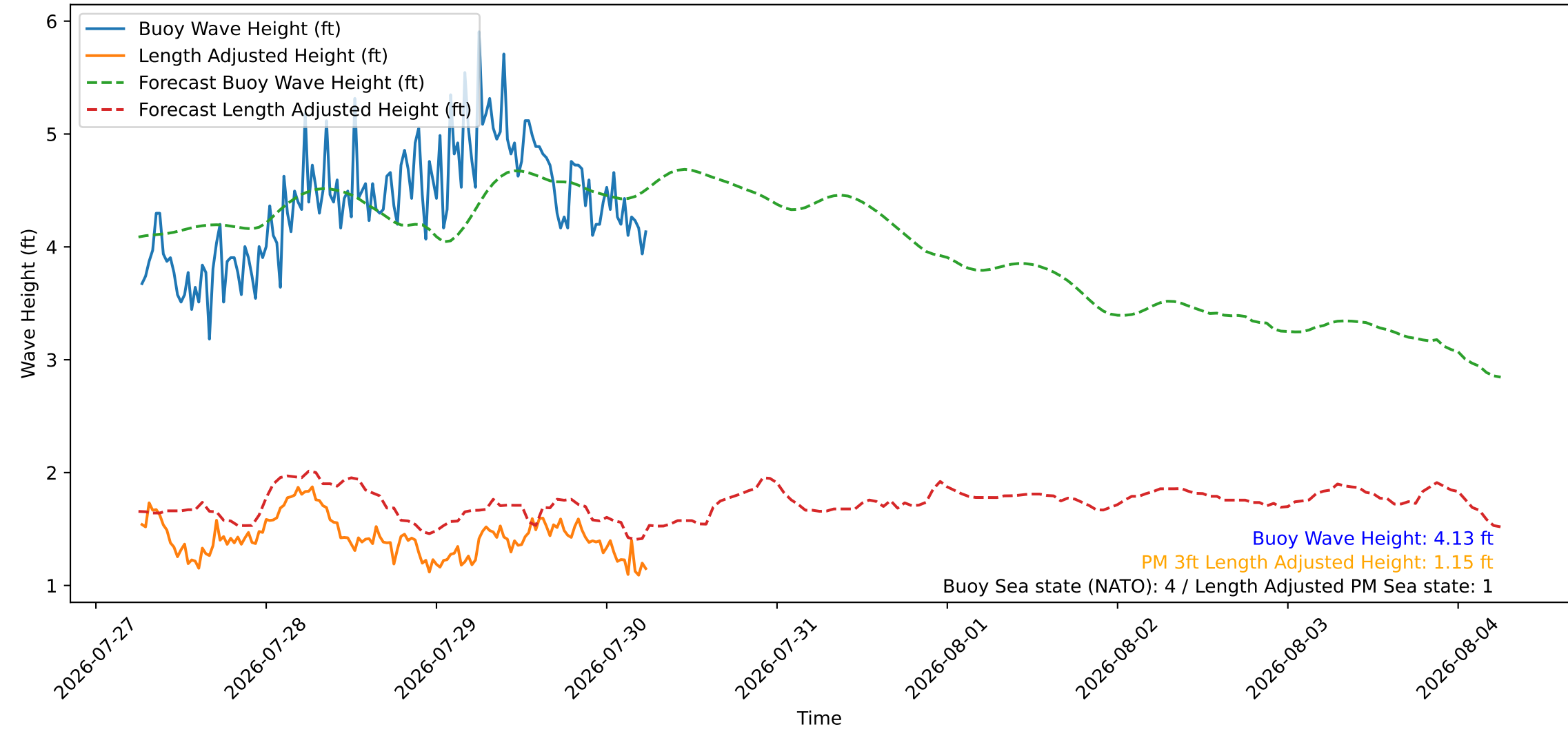
Wave Heights over Time for Oceanside Harbor at 2026-07-30 06:20:26
