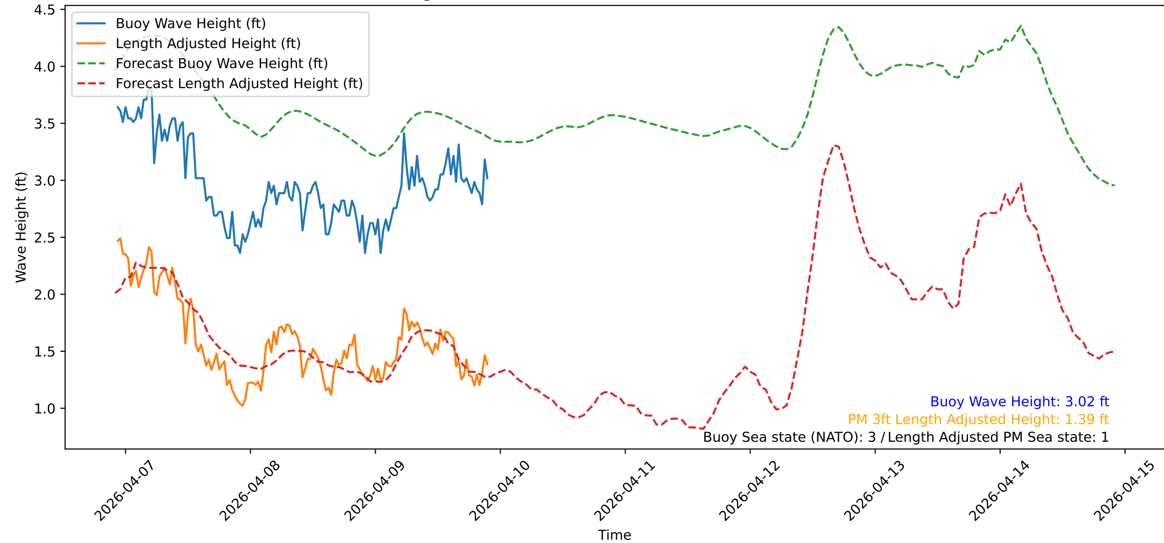
Wave Heights over Time for Green Beach at 2026-04-09 22:21:10
