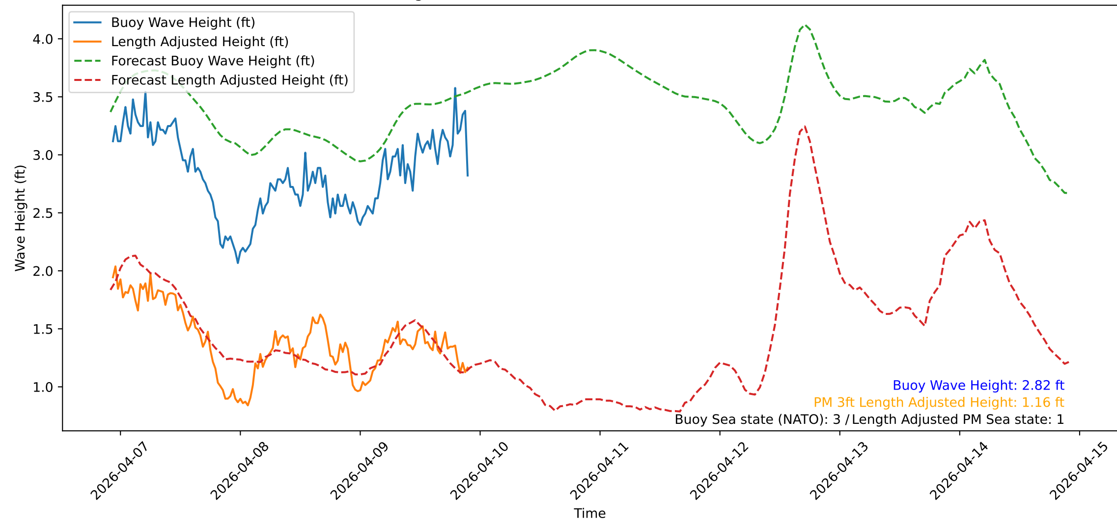
Wave Heights over Time for Red Beach at 2026-04-09 22:20:48
