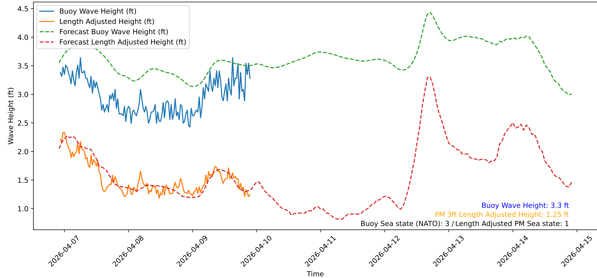
Wave Heights over Time for Oceanside Harbor at 2026-04-09 22:20:32
