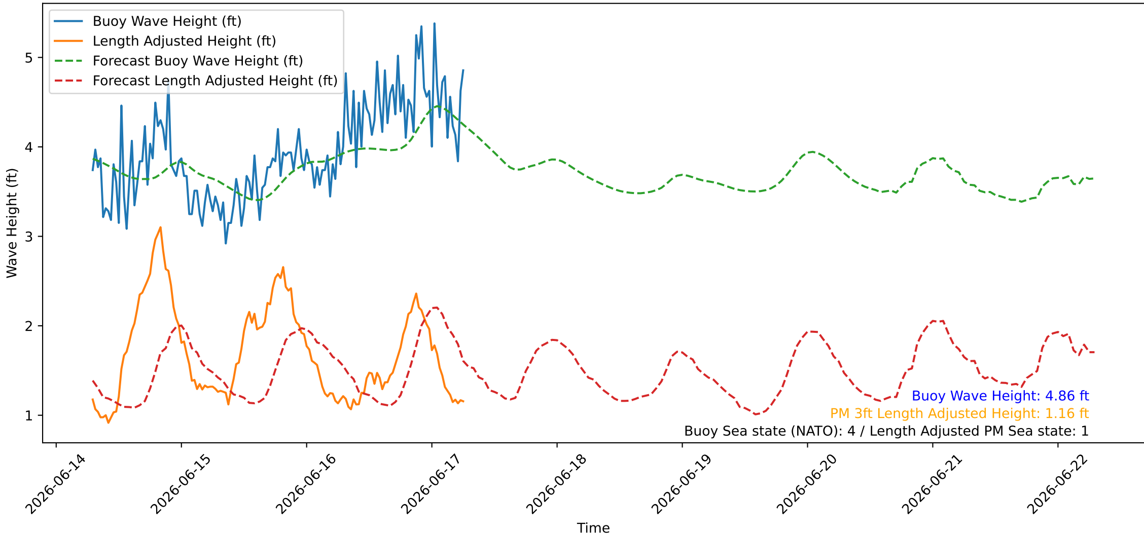
Wave Heights over Time for Red Beach at 2026-06-17 06:40:46
