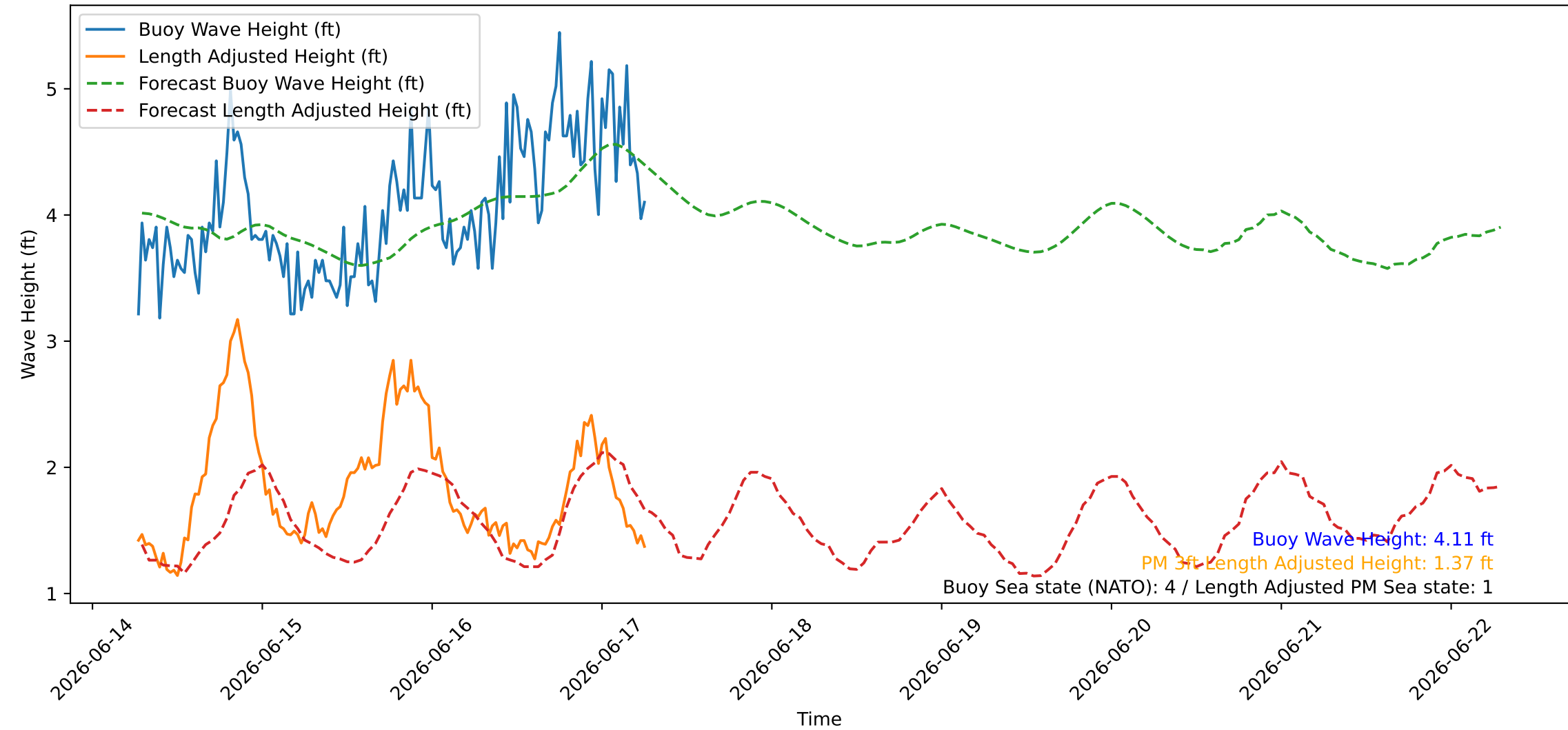
Wave Heights over Time for Oceanside Harbor at 2026-06-17 06:40:27
