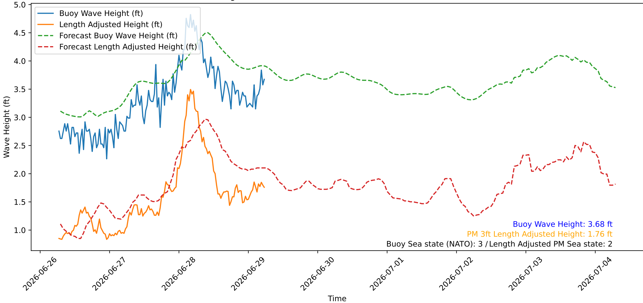
Wave Heights over Time for Green Beach at 2026-06-29 06:31:07
