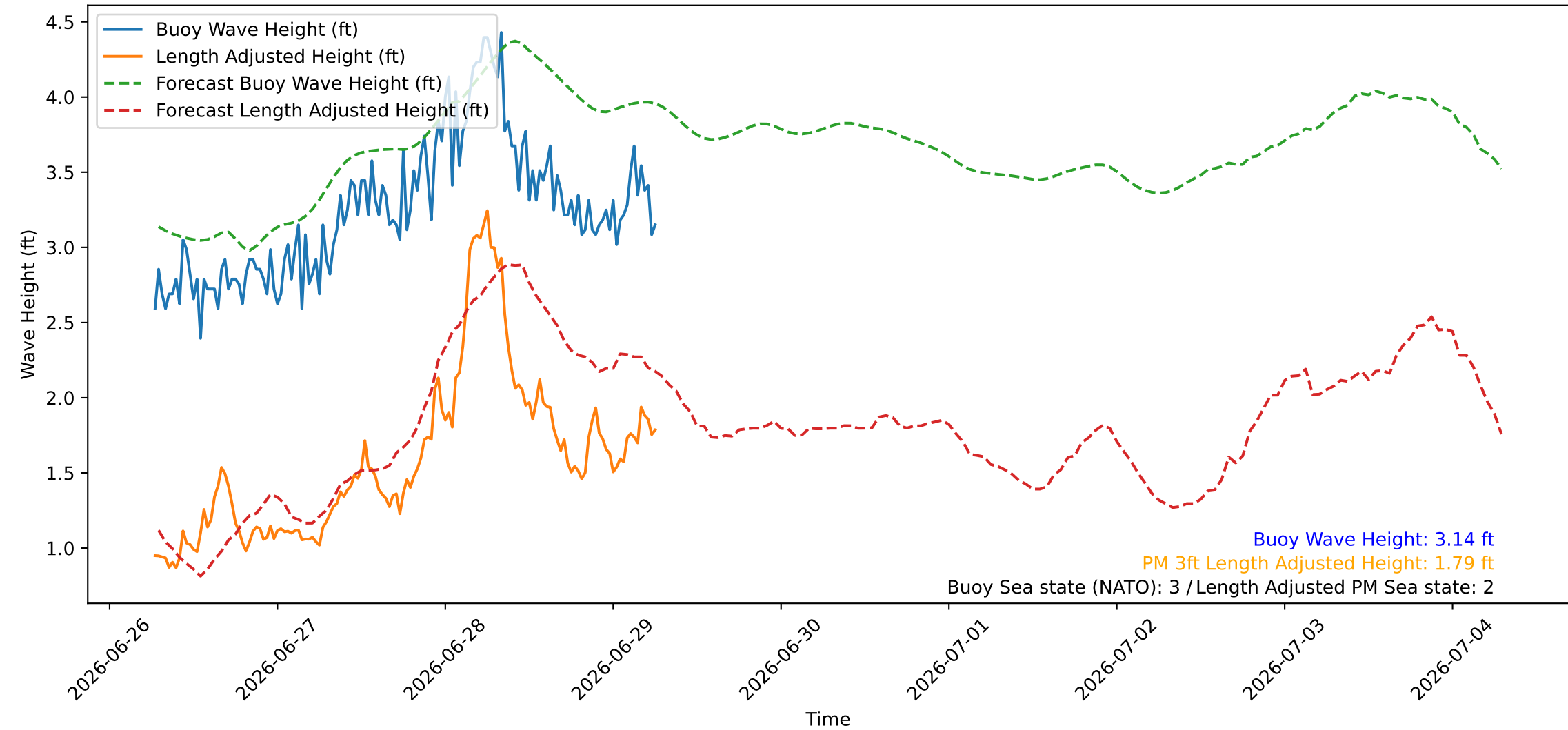
Wave Heights over Time for Oceanside Harbor at 2026-06-29 06:30:26
