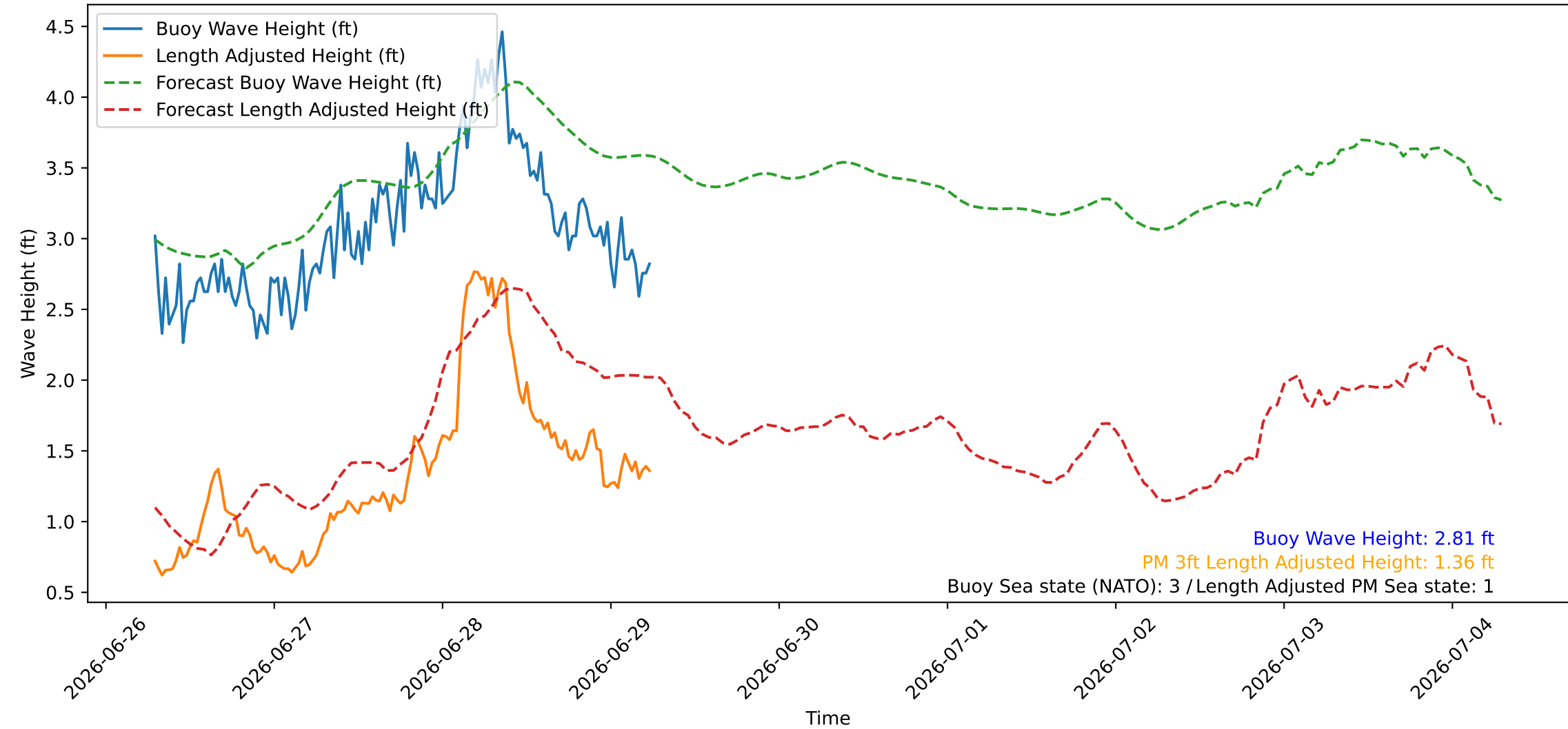
Wave Heights over Time for Red Beach at 2026-06-29 06:30:45
