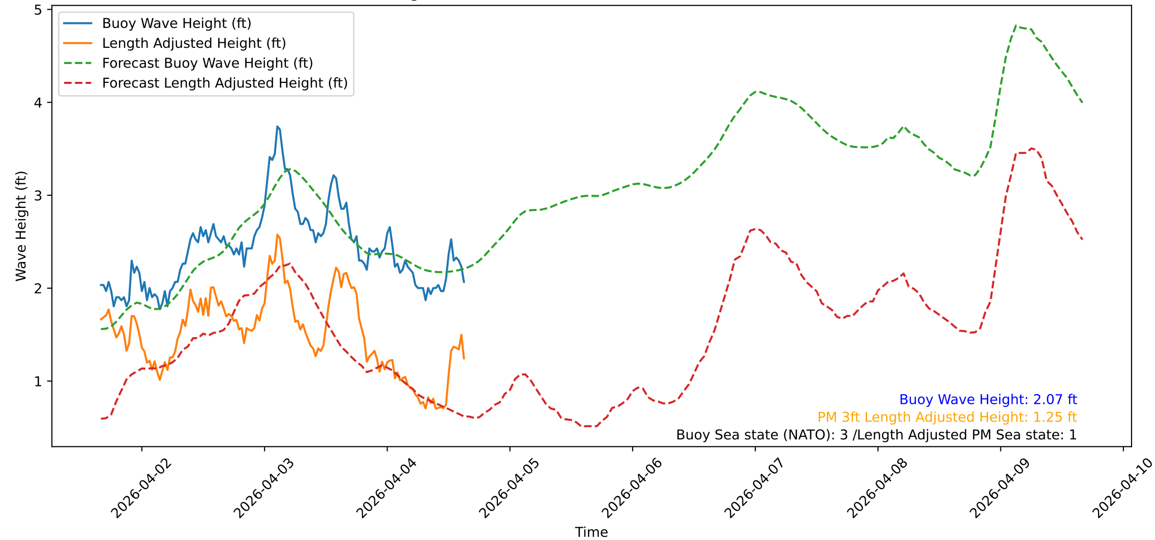
Wave Heights over Time for Red Beach at 2026-04-04 15:50:51
