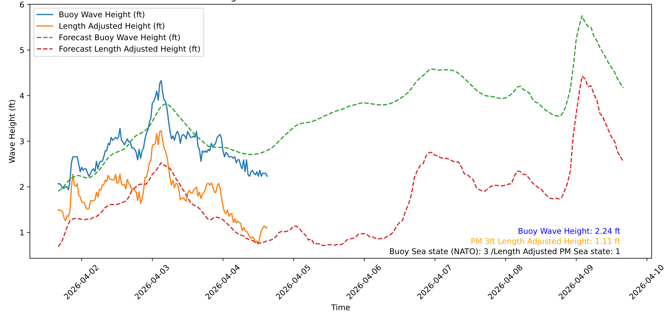
Wave Heights over Time for Green Beach at 2026-04-04 15:51:16
