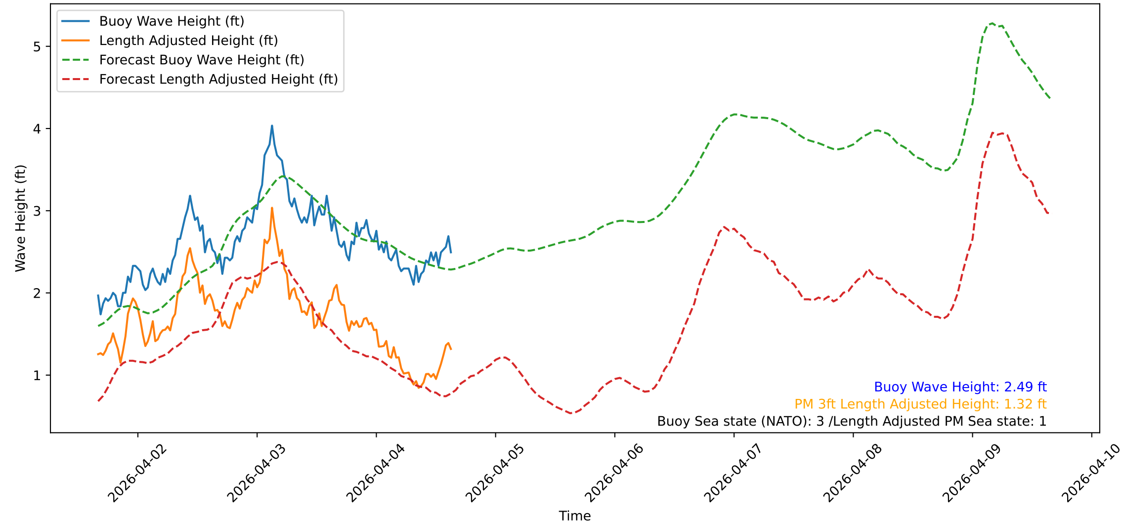
Wave Heights over Time for Oceanside Harbor at 2026-04-04 15:50:33
