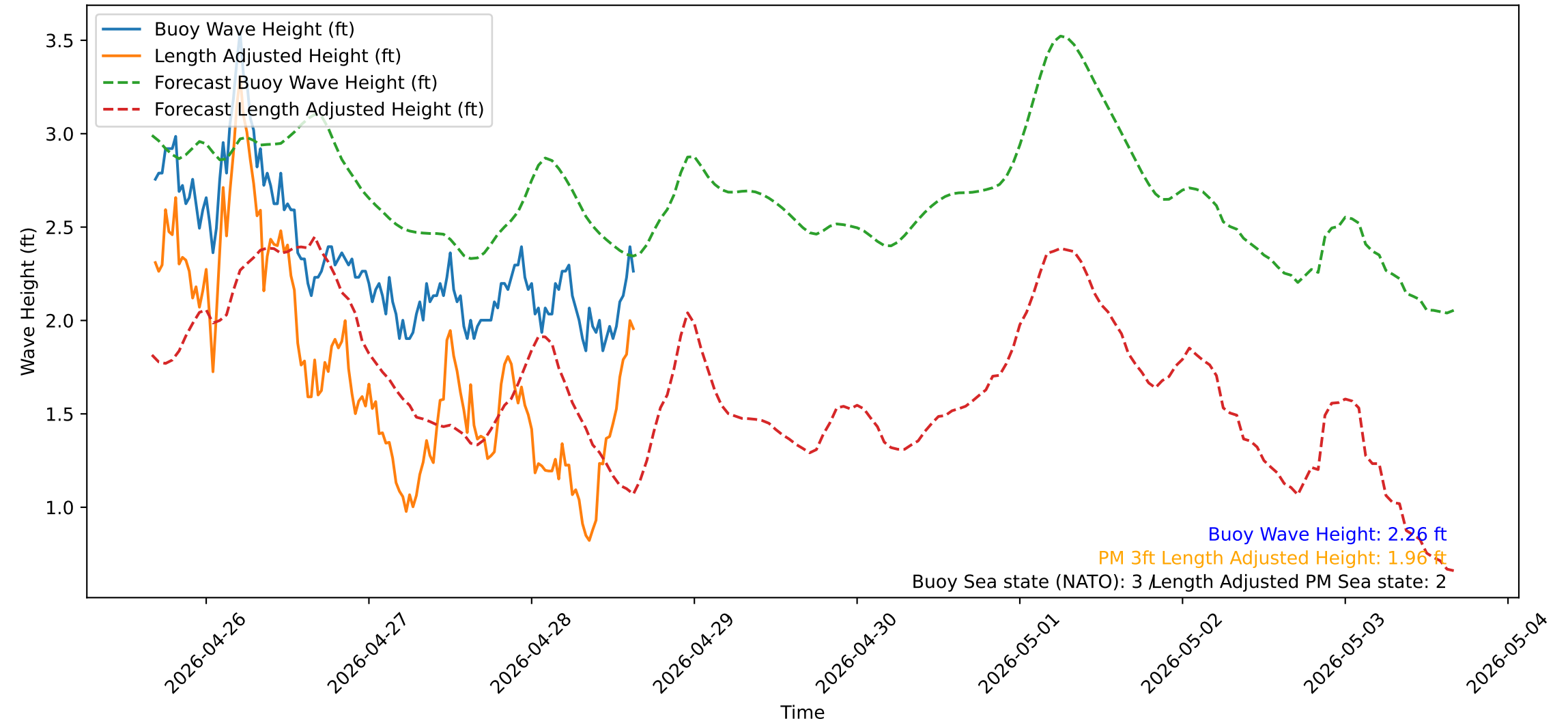
Wave Heights over Time for Red Beach at 2026-04-28 16:00:50
